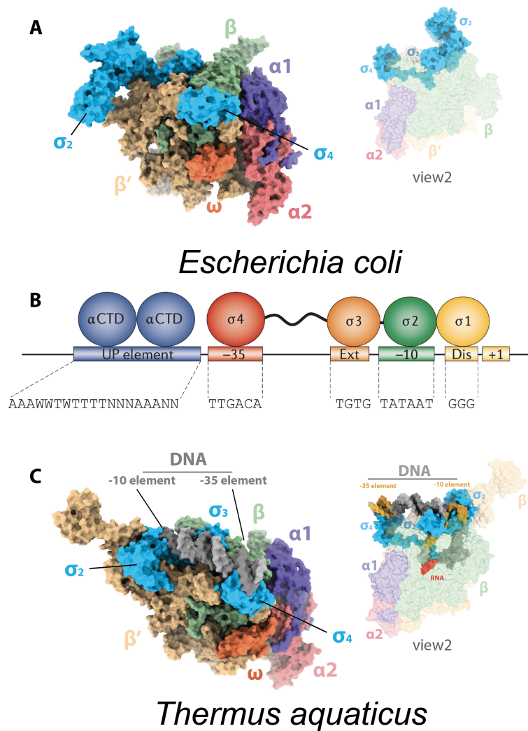
Figure 2 Bacterial promoter DNA and its interaction with RNAP and \sigma factor.
