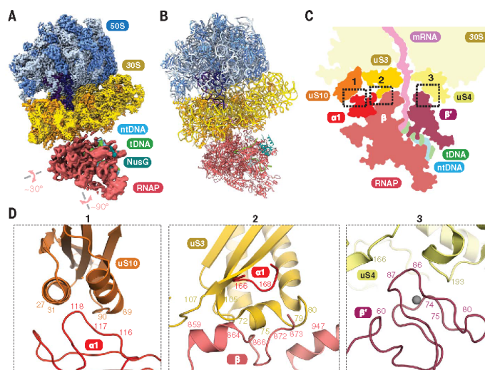
Fig. 3. Structural models of the collided expressome. (A and B) Cryo-EM map and model of the collided expressome. (C) Schematic cross section indicating three regions of close contact between RNAP and ribosome (indicated by dashed rectangles). (D) Details of the interaction interfaces of RNAP with the ribosome. Rectangles 1 to 3 correspond to the dashed rectangles in (C).
