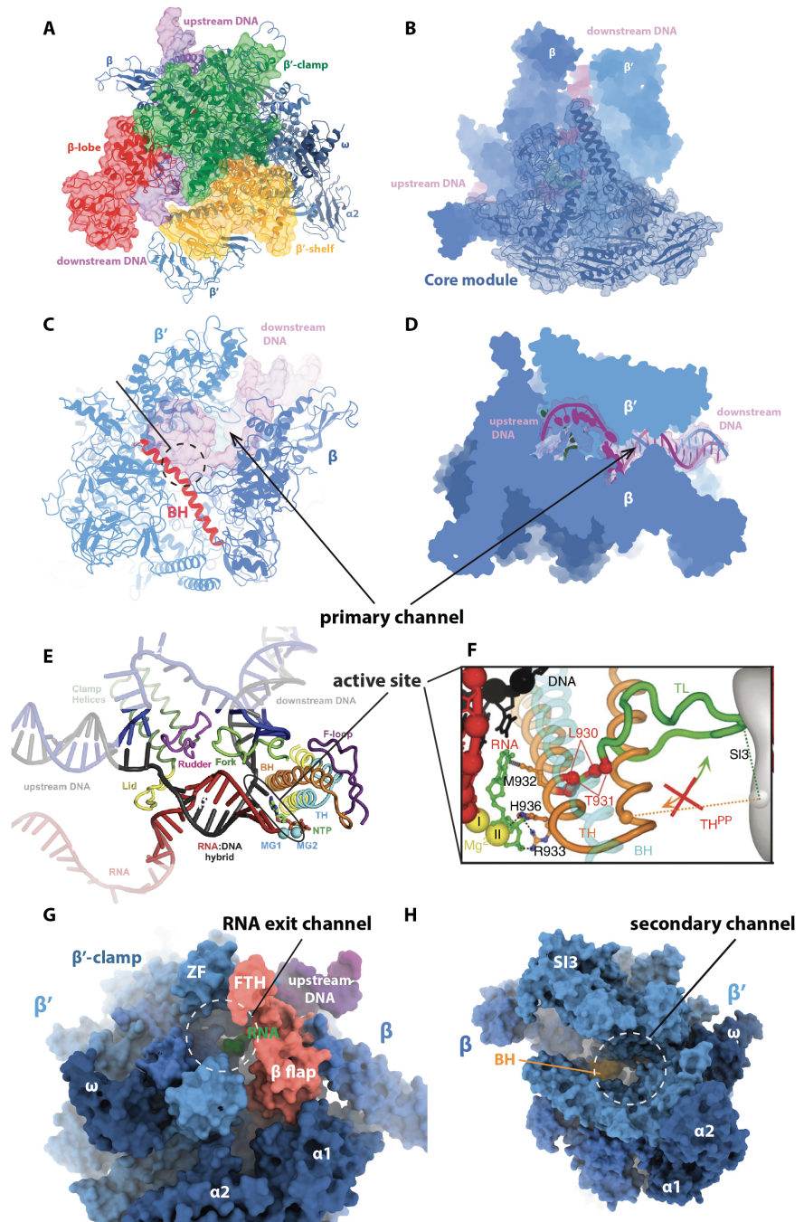
Figure 4 : Structure of elongation complex with its active site. Different elements, modules, domains and subunits of RNAP are labelled in the figure in A-H. E and F adopted from (Belogurov and Artsimovitch, 2019; Zhang et al., 2010).
