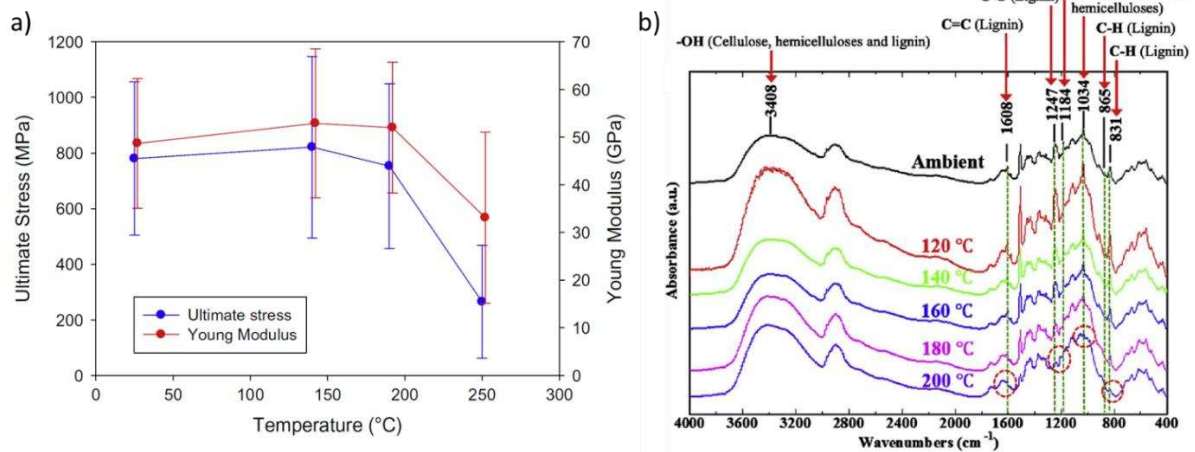
Figure 1-28: a) Temperature influences on the tensile mechanical properties of elementary flax fibres [193], b) Evolution of the biochemical components of elementary flax fibres investigated through FTIR [195].
