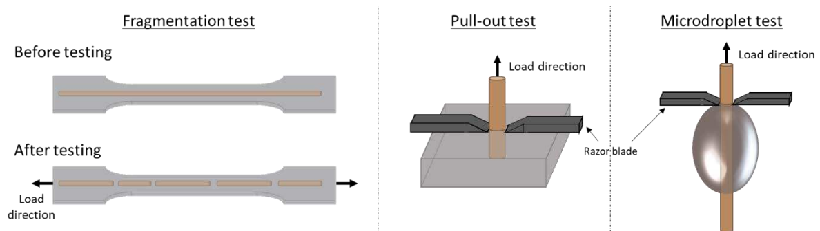
Figure 1-16: Description of the micro-scale investigation protocol for interface strength quantification.
