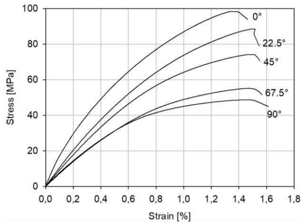
Figure 3-9: Tensile behaviour of non-woven flax/PLA with 50 wt% of fibres at several loading angles. The 0° refer to the machine direction (of the preform manufacturing) and the 90° to the cross direction.
