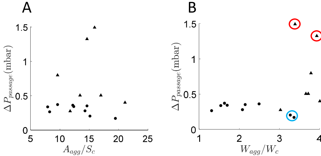
Fig. 39. Graph displaying the pressure of passage \Delta P_{pass} as a function of the size of the aggregates, in terms of the rescaled area (A) or width (B). Circles correspond to experiments performed at Constant pressure and the triangles to experiments performed at Increasing pressure steps. The aggregates which display behaviors that do not follow the general trend are highlighted with colored circles. Red circles correspond to large aggregates that display an abnormally high \Delta P_{pass} and blue circles indicate large aggregates with an unusually low \Delta P_{pass} . The error of \Delta P_{pass} corresponds to the precision of the pressure control system and is of \pm 0.01 mbar (error bar not shown).
