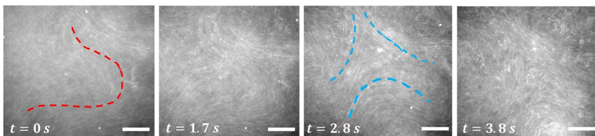
Fig. 22. Biomimetic cytoskeleton reconstitution transitioning from a +1/2 to a -1/2 topological defect. (lines in red and blue respectively). The microtubule filaments condense in the interface between the aqueous solution and the oil, displaying an active nematic behavior. When the antiparallel microtubule filaments slide against each other, they produce internal flows. Scale bar 50\ \mu\text{m} .
