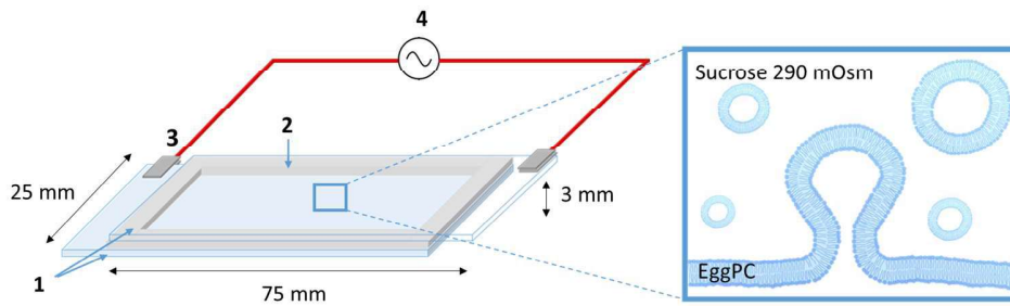
Fig. 17. Drawing of an electroformation chamber with its different parts. The inset displays the electroswelling of a lipid bilayer. 1) ITO glasses, 2) PDMS spacer, 3) Clamps and copper wire, 4) AC generator.
