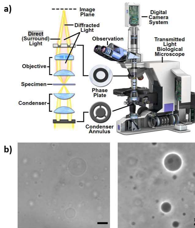
Fig. 23.A. Structure of a phase contrast microscope. Light coming from the light source passes through the condenser annulus and gets focused by the condenser lens. As it reaches the specimen, the light passing through it gets refracted, changing the angle in which it hits the objective lens. The phase plate shifts the phase between the refracted and non-refracted light, creating a phase difference that is visible for the observer. Adapted from [127]. B. Photo of GUV sample in bright field (left) and phase contrast (right). The inner part of the vesicles is filled with a 290 mOsm sucrose solution and the media is a 300 mOsm glucose solution.
