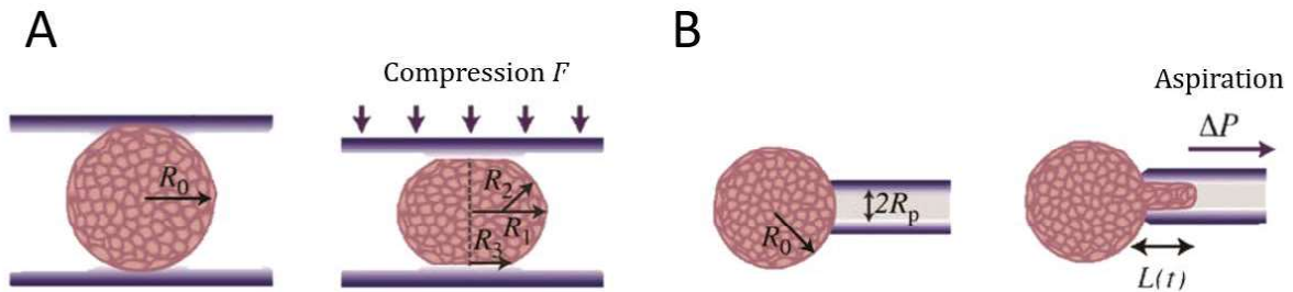
Fig. 11. A. Parallel plate compression experiments. R_0 is the initial radius of the aggregate. Upon compression at a certain force F , the aggregate deforms until a new equilibrium state is reached. R_1 and R_2 correspond to the curvature radii of the compressed aggregate. R_3 is the radii of the contact area of the aggregate with the plates. The surface tension, viscosity and the elastic modulus can be inferred from tracking the changes in the shape deformation with time. B. Micropipette aspiration experiments. The aggregate with an initial radius R_0 is aspirated at a constant pressure difference \Delta P in a glass micropipette with a radius R_p . The evolution of the protrusion length with time L(t) is tracked, and the viscosity and elastic modulus are calculated from the stress-strain curves. The aggregates' surface tension is calculated by relating the minimal applied pressure to aspirate the aggregate P_c with R_0, R_p . From [86].
