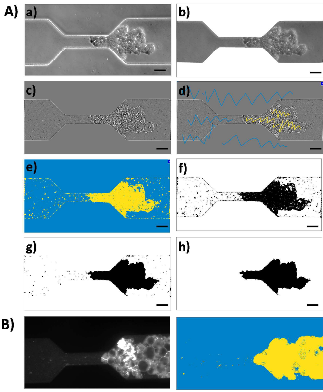
Fig. 32. A. Steps of the image treatment process. a) Original phase contrast image. b) Channel edge removal. c) Application of Convolve and Bandpass filters to increase the edge contrast of the aggregate and smooth out objects smaller than 10 pixels. d) Manually highlighting the regions corresponding to the aggregate (yellow) and to the background (blue). e) Pixel classification depending on their texture. f) Binarization of the image, in which the aggregate pixels are assigned a value of 255 and the background pixels are given a value of 0. g) Erosion of the channel edges and filling the holes inside of the aggregate. h) Filtering objects that are smaller than the aggregate. B. Epifluorescence image of an aggregate flowing through a constriction before (left) and after ILASTIK segmentation (right). The pixels are classified according to their intensity.
