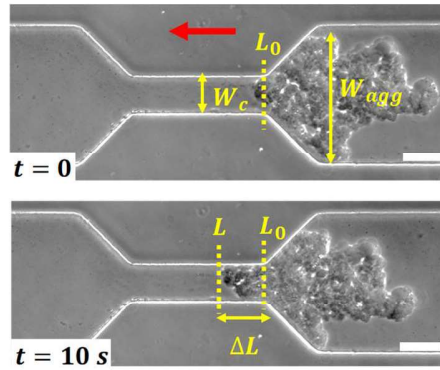
Fig. 31. Aggregate flowing through a constriction with width W_c at a constant pressure for a time interval of 10 s. The red arrow indicates the direction of the flow.
