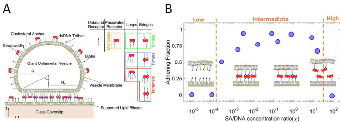
Fig. 6. A. Giant unilamellar vesicle (GUV) interacting with a supported lipid bilayer (SLB) through streptavidin-biotin bridges. B. Adhering fraction of GUVs as a function of the streptavidin/DNA concentration ratio X . In the text DNA is referred to as biotin, since every DNA molecule has a biotin at its tip. From [30].
