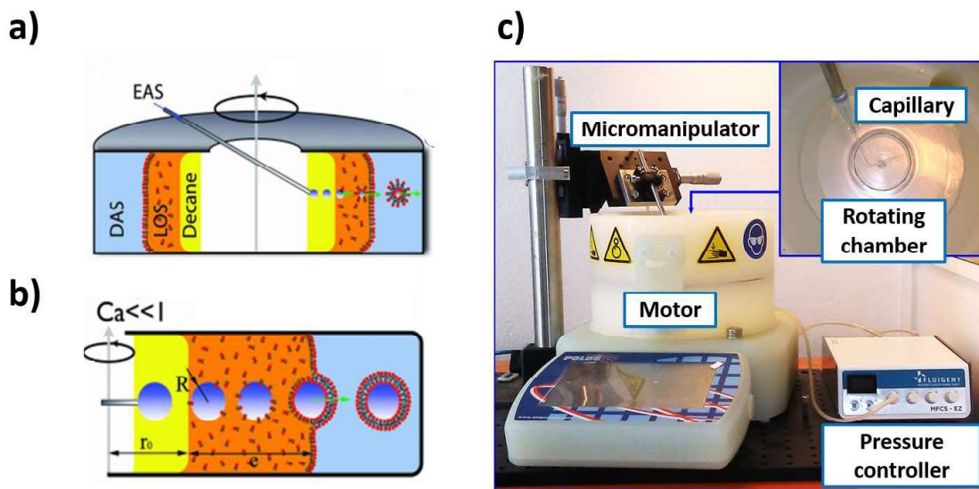
Fig. 19. A. Schematic view of a cDICE chamber displaying its different phases. B. Interface crossing by the EAS droplet through the CP, LOS and DAS. Adapted from [55]. C. Photography of the cDICE device with its different parts.
