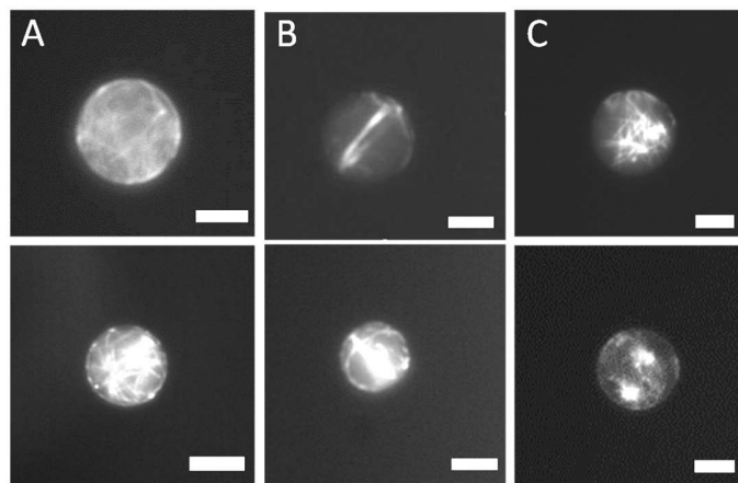
Fig. 46. Image displaying three types of microtubule distribution within the vesicles. The mean vesicle diameter was 15 \pm 3 \mu\text{m} . A. Network-like structure, B. Ring-like structure, C. Clumped filaments. Exposition time 1.5 s. Scale bar 10 \mu\text{m} .
