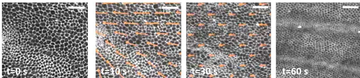
Fig. 1. Snapshots displaying the flow field of cells on the wing of Drosophila melanogaster during morphogenesis over a time lapse of 60 s. Cells are initially in a stationary state (0 s) and upon receiving a chemical input, they start reorienting and reorganizing (10 s). Cells flow and migrate (30 s) until they finally reach their final configuration, forming the characteristic microscopic structures of a wing (60 s). The arrows indicate the direction of the flow field. At t = 30 s, it is possible to see how cells stretch and deform as they flow. The translation, reorientation and separation of cells enable the formation of the different patterns forming the Drosophila melanogaster wing. Scale bar 50 \mu\text{m} . Adapted from [5].
