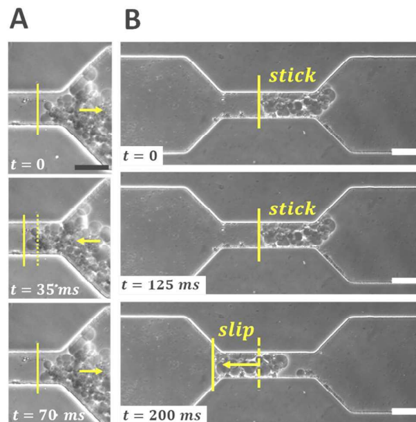
Fig. 38. Aggregates displaying two types of stop-and-go motion: A. Periodic oscillations and B. Stick and slip. The dotted lines represent the starting position of the front of the aggregate, and the filled lines the displacement of the aggregate front. The arrows represent the direction in which the aggregate moves. Scale bar 50\ \mu\text{m} .
