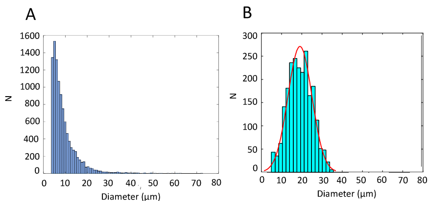
Fig. 18. A. Size distribution of electroformed vesicles, with a mean diameter of 9 \pm 6 \mu\text{m} and a sample size of N=10000 . B. Size distribution of cDICE vesicles, which follows a normal distribution with \mu=19 \mu\text{m} and \sigma=6 \mu\text{m} . Sample size N=2500 . The parameters used for cDICE vesicles are \omega=350 \text{ rad/s} , d_i = 9 \mu\text{m} . The number of vesicles N differs significantly in both cases, since the yield of electroformed vesicles is much higher than that offered by cDICE.
