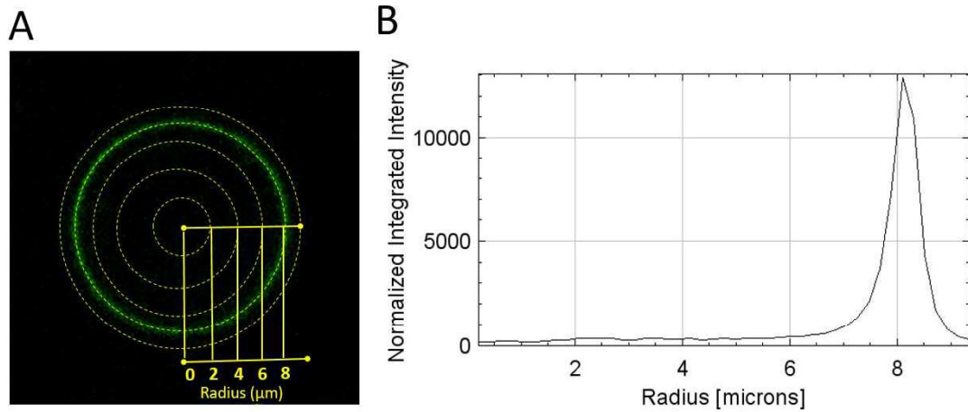
Fig. 30. A. Radial profile analysis with ImageJ in a transversal cut of a vesicle, imaged by confocal microscopy. B. Normalized integrated pixel intensity as a function of the vesicle radii. Each point of the graph corresponds to the sum of intensities of the pixels at a certain distance from the center, indicated by the yellow discontinuous lines in Figure A. All values are normalized by the perimeter of the circle.
