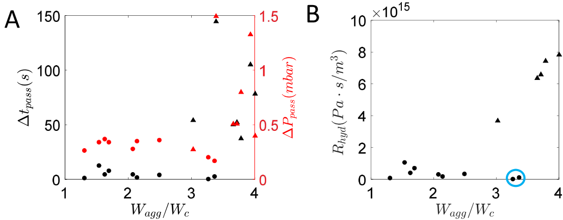
Fig. 41. A. Time of passage \Delta t_{pass} as a function of the aggregate size. B. Hydraulic resistance of the aggregates as a function of the aggregate size W_{agg}/W_c . Dots correspond to the experiments performed at constant pressure and the triangles to the experiments performed at increasing pressure steps.
