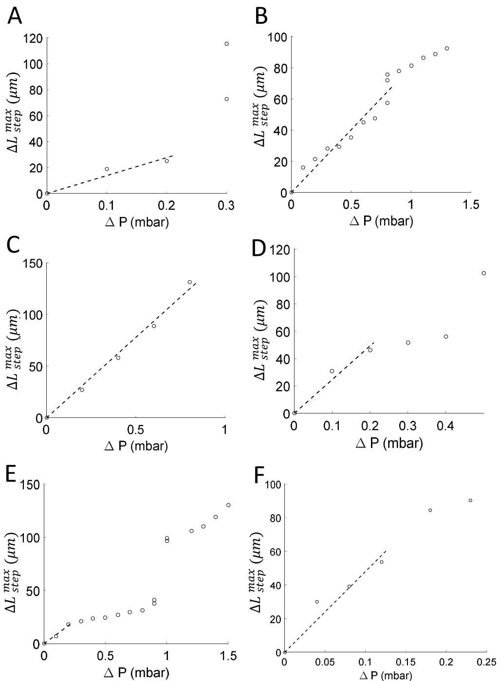
Fig. 45. Graphs displaying the maximal deformation of the aggregate for each step as a function of the applied pressure. For some steps, two values of \Delta L_{step}^{max} can be found, which correspond to intermediate deformations. The slope of the linear fit and the R-square values are, from A to F: 139 \pm (75) \mu\text{m}/\text{mbar} ; R-square=0.9119, 81 \pm (11) \mu\text{m}/\text{mbar} ; R-square=0.9052, 156 \pm (75) \mu\text{m}/\text{mbar} ; R-square= 0.9903, 246 \pm (13) \mu\text{m}/\text{mbar} ; R-square= 0.9547, 86 \pm (26) \mu\text{m}/\text{mbar} ; R-square= 0.9779, 481 \pm (141) \mu\text{m}/\text{mbar} ; R-square= 0.9144.
