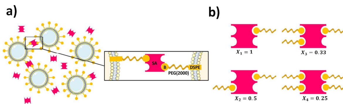
Fig. 4. A. Scheme of the biotin-functionalized vesicle aggregation with streptavidin (SA). The inset shows the synthetic construct made of DSPE, PEG and biotin (B) composing the vesicle membranes. Streptavidin molecules are added in solution. B. Graphical representation of X for one streptavidin molecule and its possible configurations depending on the number of biotins interacting with it. X_1 = 1 streptavidin/1 biotin molecule, X_2 = 1 streptavidin/2 biotin molecules, X_3 = 1 streptavidin/3 biotin molecules, X_4 = 1 streptavidin/4 biotin molecules.
