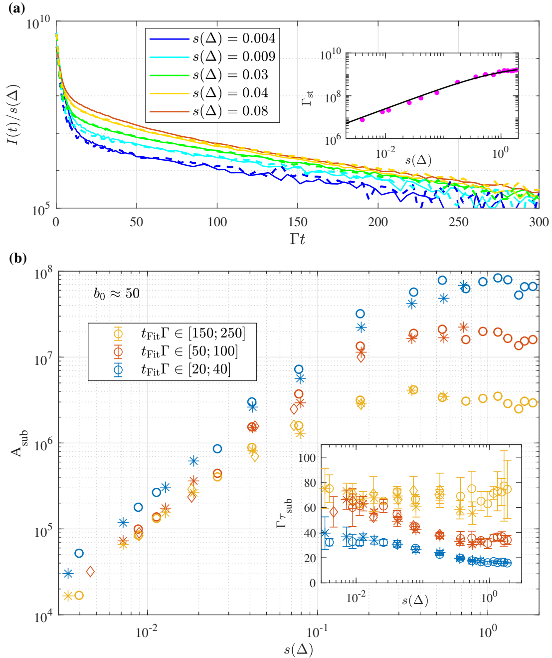
Figure I.11: (a) Temporal dynamics of the scattered intensity after the switch-off of the driving field (at t = 0 ), for different saturation parameters s(\Delta) as well as for \Delta = -2\Gamma (solid line) and \Delta = -4\Gamma (dashed line). The decay curves for both detunings collapse, which indicates that the temporal dynamics is independent of the detuning. The intensity curves are normalized by s . Even after this normalization, the amplitude of the slow decay (corresponding to the long-lived collective modes) increases with s , which illustrates well the super-linear growth of the long-lived mode populations. Inset: Steady-state scattering rate \Gamma_{st} as a function of the saturation parameter s for b_0 \approx 50 and \Delta = -2\Gamma . The measured \Gamma_{st} is represented by full circles, while the solid line corresponds to the fit function \Gamma_{st} \propto s/(s+1) . (b) Subradiant amplitude A_{sub} as a function of s(\Delta) for detunings \Delta = -2\Gamma ( \circ symbol), \Delta = -4\Gamma ( * symbol) and \Delta = -8\Gamma ( \diamond symbol) as well as for different fit intervals t_{Fit} represented by different colors as indicated on the legend. The inset shows the corresponding lifetimes \tau_{sub} . A_{sub} and \tau_{sub} were obtained by fitting I(t) = A_{sub} \exp(-t/\tau_{sub}) to the non-normalized decay curves (which are for example shown on Fig. I.7(a)) over a given time window t_{Fit} . The on-resonance optical thickness is b_0 \approx 50 for the results shown on both (a-b) panels.
