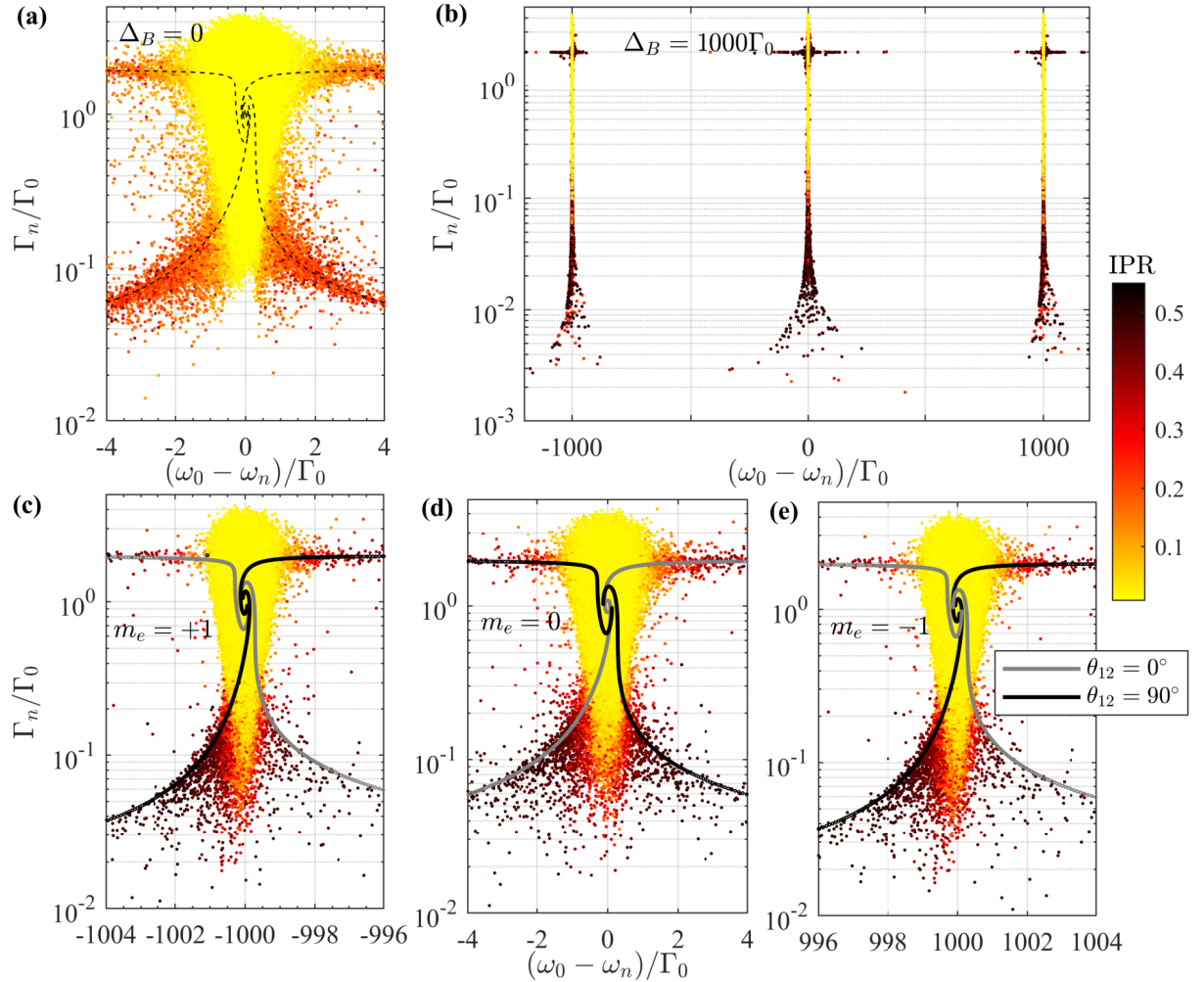
Figure III.10: Eigenvalue distribution obtained by diagonalizing the \bar{G} matrix given by Eq. (III.32) for a cylindrical atomic sample of size k_0L = 21.5 and uniform density \rho\lambda^3 = 5 in the case of degenerate excited state (no magnetic field is applied; \Delta_B = 0 ) (a) and in the case of atoms subjected to a strong magnetic field that produces a Zeeman shift \Delta_B = 1000\Gamma_0 (b-e). When the strong magnetic field is applied, the eigenvalues are well split into three groups centered around \omega_0 - \omega_n = -m_e\Delta_B , thus each group corresponding to a transition to a given m_e substate (b). Panels (c-e) are the close-ups of panel (b) on an eigenvalue group corresponding to m_e = +1 (c), m_e = 0 (d) and m_e = -1 (e). The dashed black lines on panel (a) corresponds to the analytical solution of subradiant and superradiant pair eigenvalues given by Eqs. (II.21) and (II.22). When the strong magnetic field is applied, the eigenvalues associated to the close pairs of atoms are as well split into three groups corresponding to a given transition m_e = 0, \pm 1 . Contrary to the case of degenerate atoms, in the case of applied magnetic field, the pairs eigenvalues depend on the angle \theta_{12} between the axis along which the atomic pairs are positioned and the axis given by the direction of applied magnetic field \hat{z} . The gray and black solid lines on panels (c-e) correspond to the pairs eigenvalues for \theta_{12} = 0^\circ and \theta_{12} = 90^\circ , respectively, obtained by diagonalizing the \bar{G} matrix [Eq. III.32] for N = 2 atoms and their varying separation distance with \theta_{12} = 0^\circ and \theta_{12} = 90^\circ . For all other angles \theta_{12} , the eigenvalues fall in between those two lines. The colorcode corresponds to the inverse participation ratio (IPR). The eigenvalues are plotted for N_r = 300 realizations of atomic positions.
