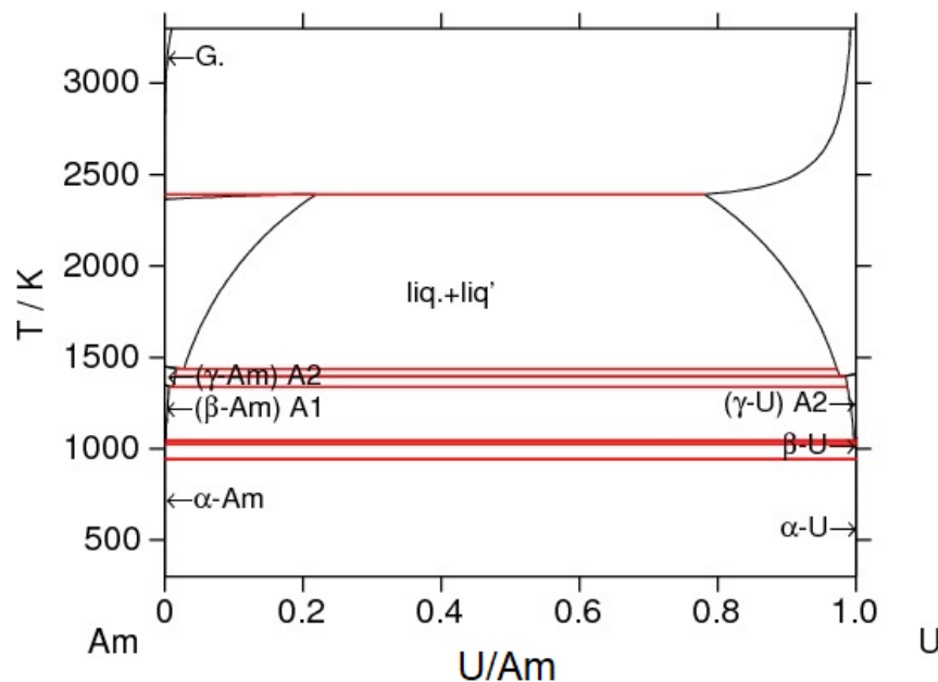
Figure 1 : Calculated U-Am phase diagram [252].
