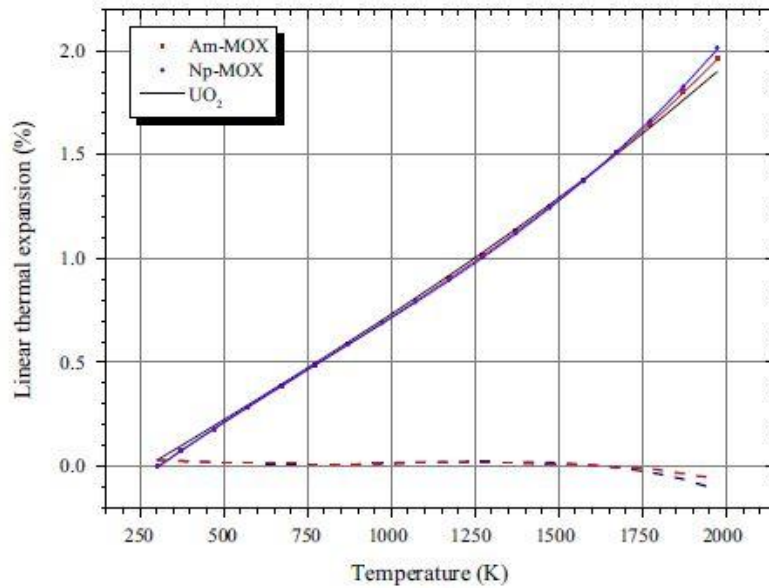
Figure 2-23 : Variation in the thermal expansion of U_{0.74}Pu_{0.22}Am_{0.035}Np_{0.005} as a function of temperature, compared to UO_2 [124].
