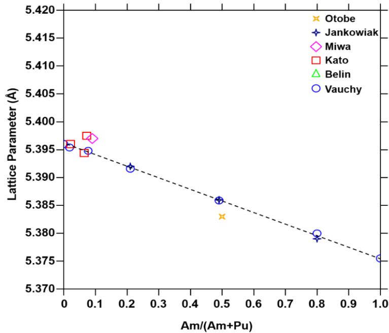
Figure 2-13 : Variation in the lattice parameter of the fluorite structure of Pu_{1-z}Am_zO_2 as a function of the Am content at room temperature (experimental data available in Appendix B from [42], [44], [73], [78], [81], [82]).
