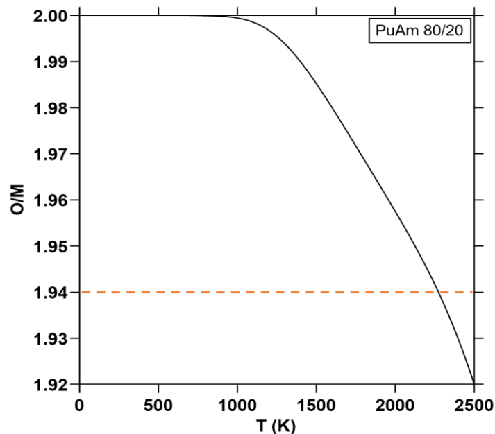
Figure 6-19: Variation of the O/M ratio as a function of temperature for the PuAm 80/20 sample in equilibrium with air. The dashed line corresponds to the O/M ratio determined experimentally in Chapter 4 – section 4.1.4.
