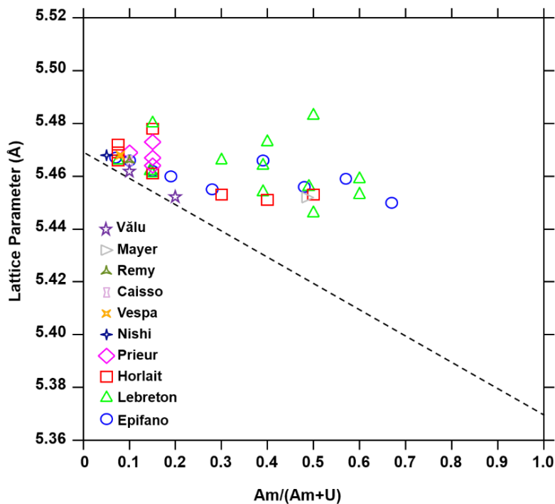
Figure 2-14 : Variations in the lattice parameter of U_{1-z}Am_zO_2 as a function of the Am content at room temperature compared to the available experimental data ([28], [83]–[91]).
