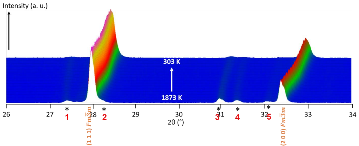
Figure 4-7: Evolution of the diffraction patterns between 26 and 34° 2\theta as a function of the temperature for PuAm 80/20.
