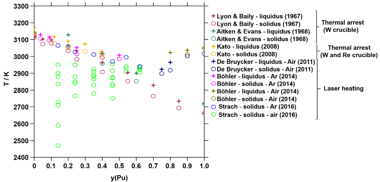
Figure 2-39: Experimental melting data available in the literature for U_{1-y}Pu_yO_{2.00} [24], [174], [176], [180], [181], [184].
