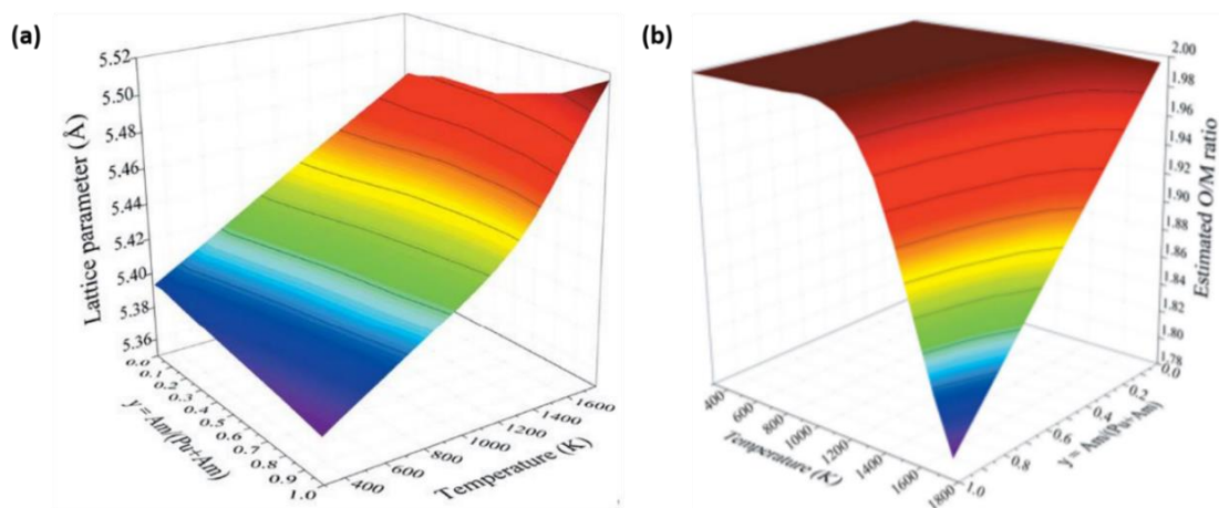
Figure 2-22 : (a) Variation in the lattice parameter of the fluorite structure of \text{Pu}_{1-z}\text{Am}_z\text{O}_{2-x} and (b) of the estimated O/M ratio as a function of temperature and Am content [73].
