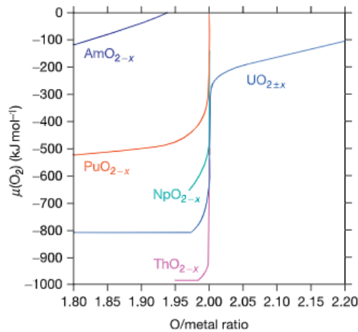
Figure 2-33: Comparison of the oxygen potentials for \text{UO}_{2\pm x} , \text{PuO}_{2-x} and \text{AmO}_{2-x} at 1600 K [131].
