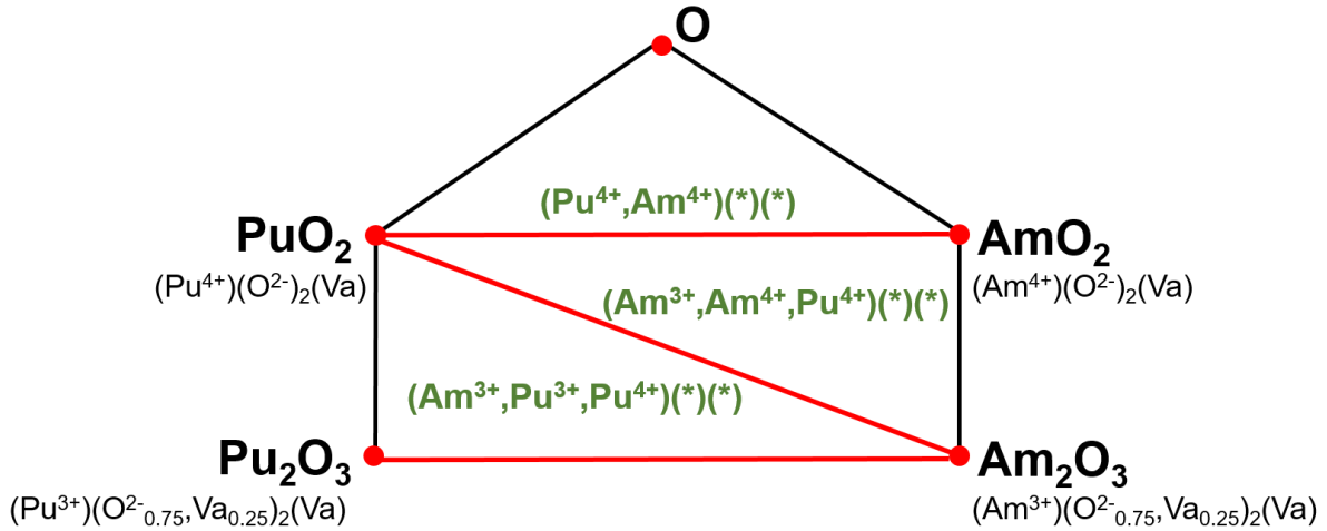
Figure 6-14: Schematic representation of the model of the MO 2-x phase for the Pu-Am-O system.
