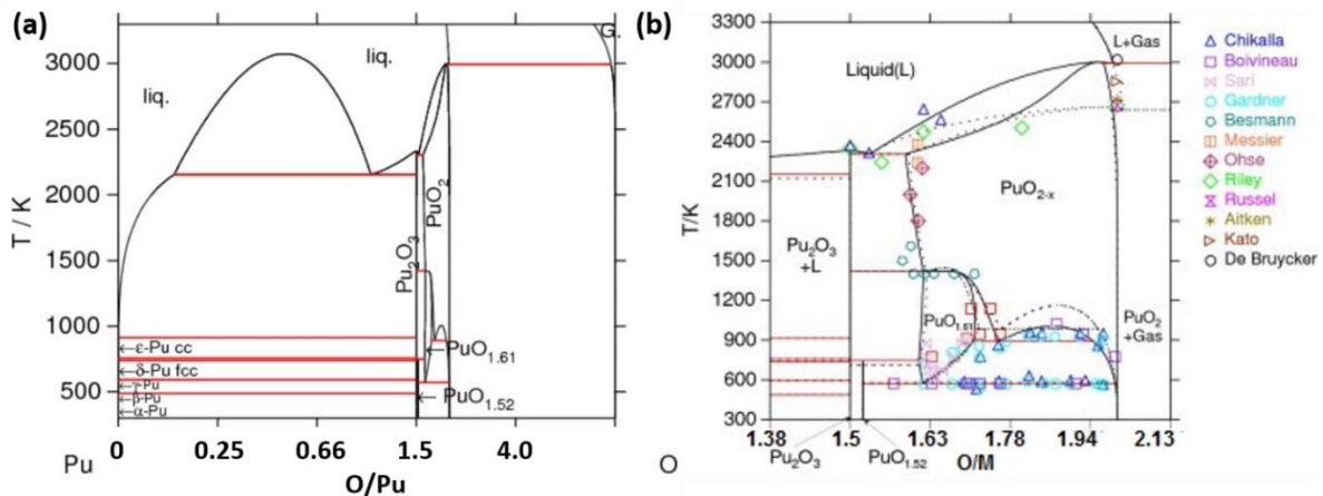
Figure 2-2 : (a) Calculated Pu-O phase diagram, (b) detailed section from 1.38 < \text{O/M} < 2.13 , using the model developed by Guéneau et al. in 2011 [6]. The dashed lines on (b) represent the model of Guéneau et al. of 2008 [23].
