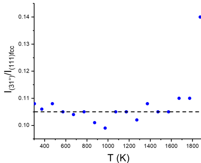
Figure 4-8: Ratio of the intensities between the peak at 31° 2\theta and the (111) reflection of the fcc phase as a function of the temperature for the PuAm 80/20 sample. The dashed line represents the average value.
