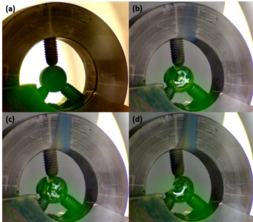
Figure 5-16: PHENIX29 sample (a) before shots, (b) after 1 shot, (c) after 4 shots and (d) after 8 shots.
