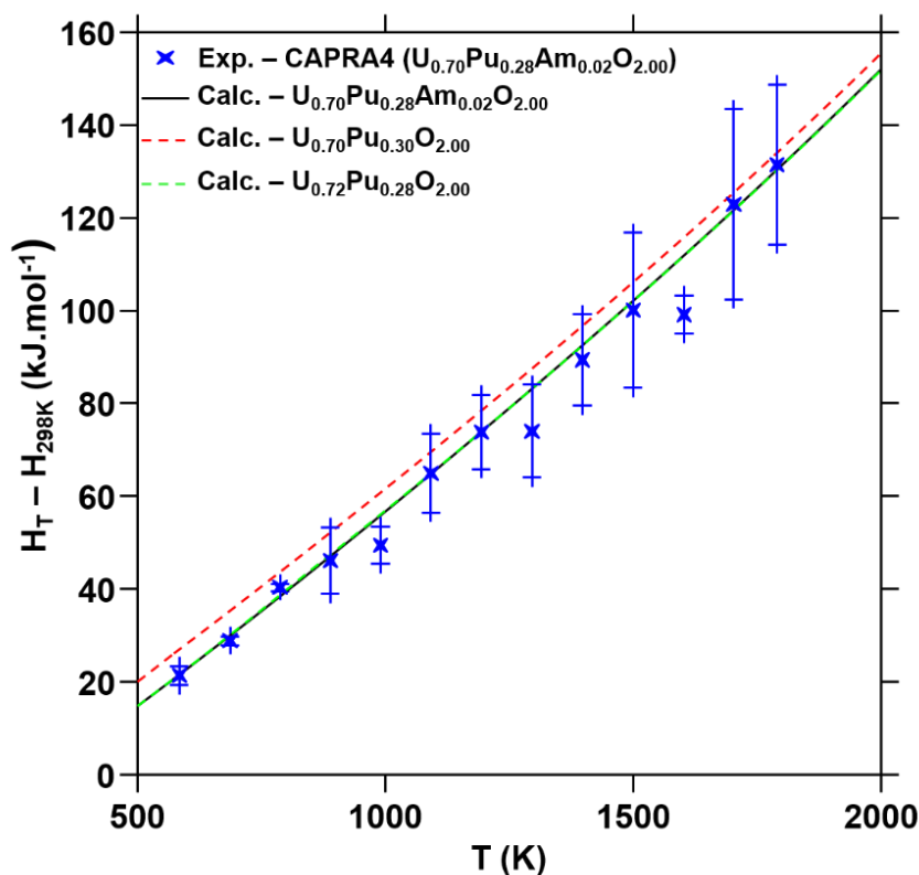
Figure 6-25: Enthalpy increments of the CAPRA4 sample compared to the calculated data for U_{0.70}Pu_{0.28}Am_{0.02}O_{2.00} (black full line), U_{0.70}Pu_{0.30}O_{2.00} (red dashed line) and U_{0.72}Pu_{0.28}O_{2.00} (green dashed line).
