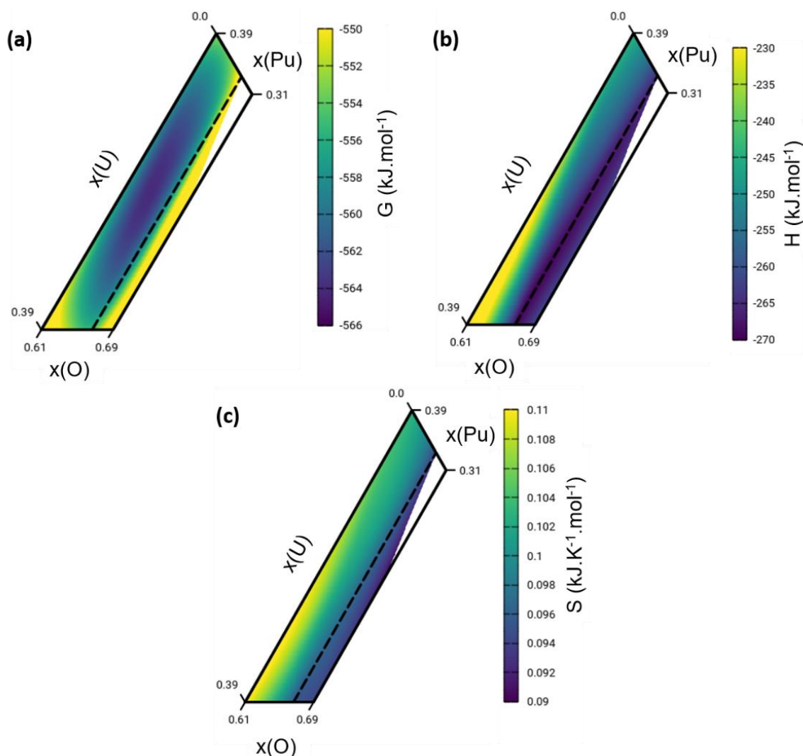
Figure 6-10: 3D map of (a) the Gibbs energy, (b) the enthalpy, (c) the entropy of U_{1-y}Pu_yO_{2\pm x} as a function of the x(O) and x(Pu) at 3000 K (dashed line: UO_2 - PuO_2 composition line).
