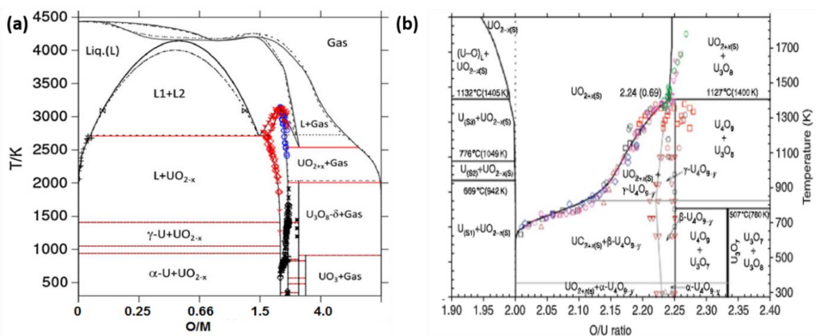
Figure 2-1: (a) Calculated U-O phase diagram from Guéneau et al. [13], (b) detailed section from 1.9 < O/M < 2.4 after Higgs et al. [15], compared to available experimental data. L and G stand for liquid and gas, respectively.
