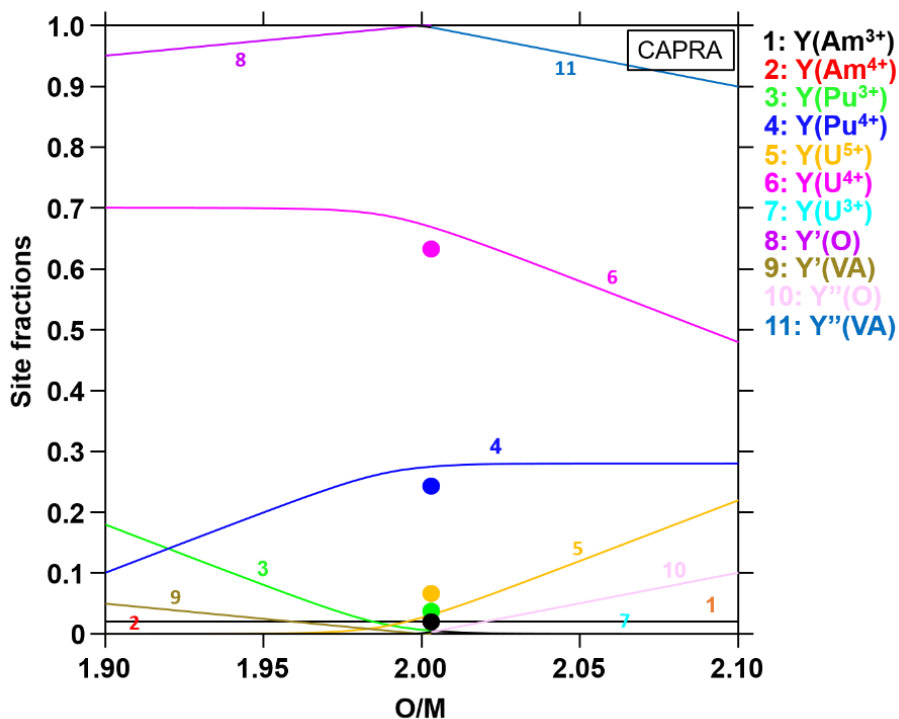
Figure 6-24: Cationic site fractions of the CAPRA4 sample calculated at 1600 K, compared to the experimental data measured by XANES in Chapter 5 – section 5.1.3. The experimental uncertainties correspond to the size of the symbol for the site fractions.
