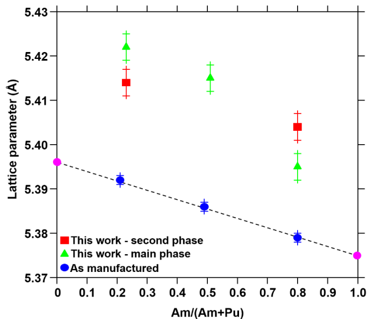
Figure 4-4: Lattice parameters obtained in this work compared to the one at the manufacturing [197] and the Vegard's law between the pure poles PuO 2 and AmO 2 .
