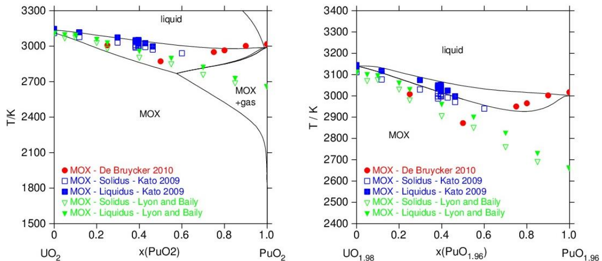
Figure 2-40 : Solidus/liquidus temperatures of \text{U}_{1-y}\text{Pu}_y\text{O}_{2+x} calculated using the CALPHAD model of Guéneau et al. [7], compared to the experimental values of De Bruycker et al. [24], Kato et al. [174] and Lyon and Baily [180].
