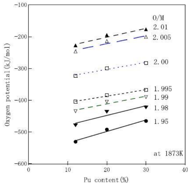
Figure 2-35 : Variation in the oxygen potential of U_{1-y}Pu_yO_{2\pm x} at 1873 K with the plutonium and for different O/M ratios [153].
