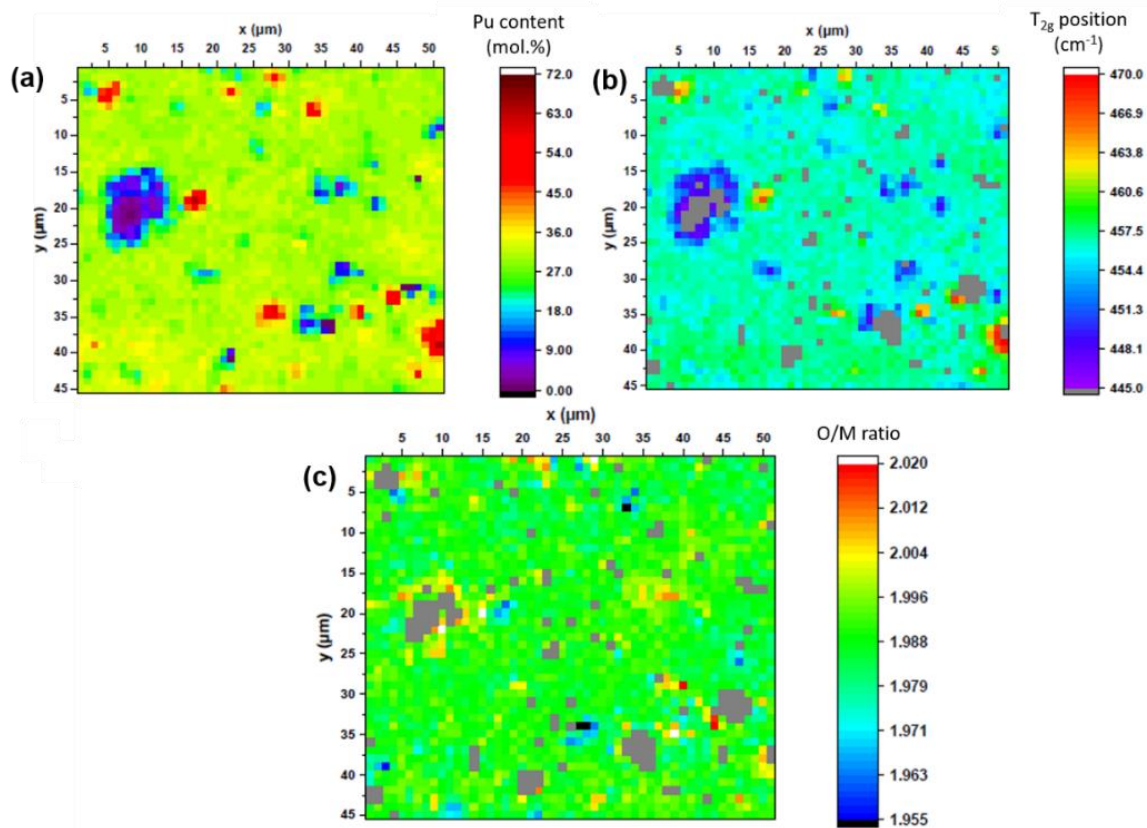
Figure 5-33: (a) Map of the Pu content by EPMA, (b) cartography of the T_{2g} position by Raman spectroscopy and (c) cartography of the O/M ratio obtained by combination of (a) and (b), for the PHENIX29 sample [54]. The grey spots correspond to points removed due to a lack of signal.
