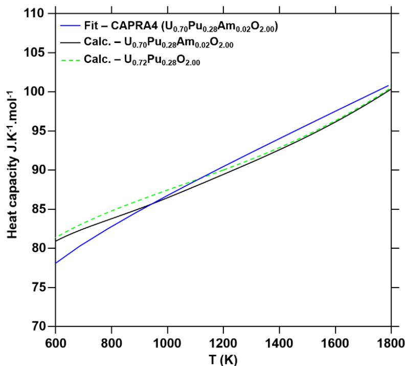
Figure 6-26: Heat capacity of the CAPRA4 sample (blue), compared to the calculated data for U_{0.70}Pu_{0.28}Am_{0.02}O_{2.00} (black full line) and U_{0.72}Pu_{0.28}O_{2.00} (green dashed line).
