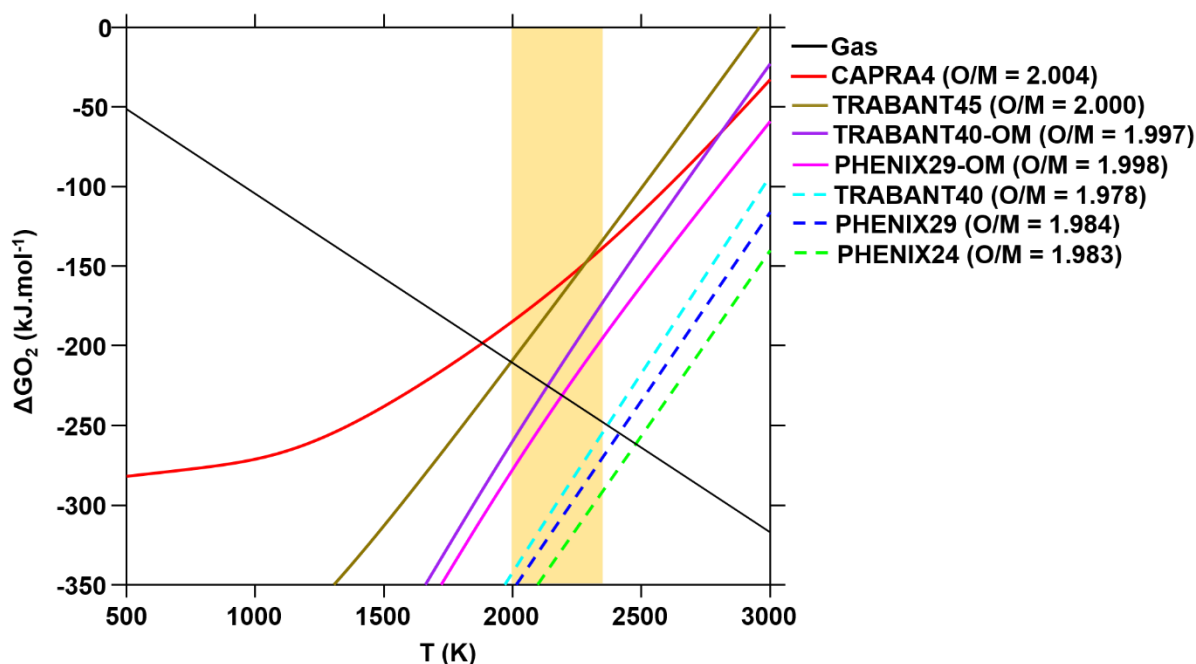
Figure 6-29: Oxygen potentials as a function of temperature for the samples studied by laser heating in Chapter 5, compared to the oxygen potential of the gas (Ar with p_{O_2} = 3.10^{-6} atm). The yellow rectangle represents the temperature range where the equilibrium O/M ratio would be reached during cooling.
