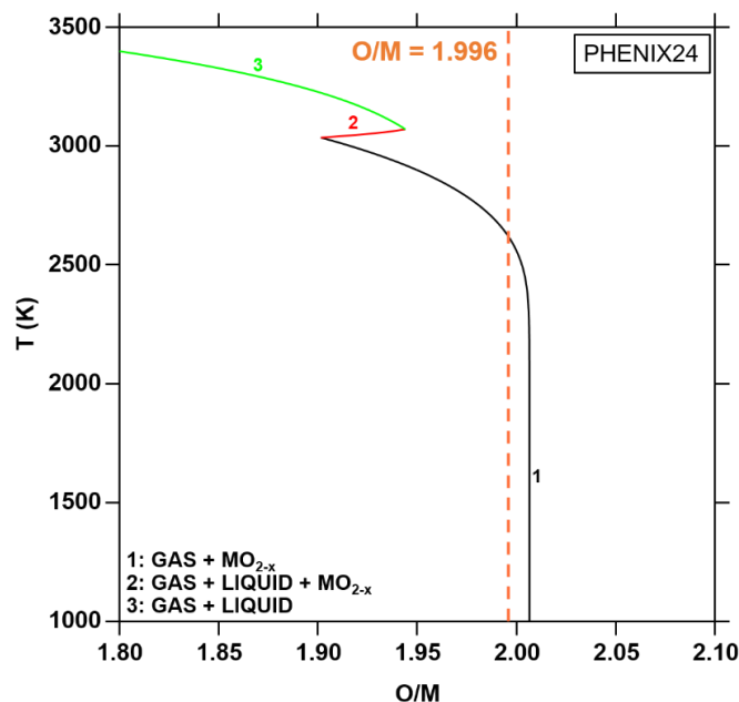
Figure 6-30: Solidification path of the PHENIX24 sample, compared to the final O/M ratio determined in Chapter 5 – section 5.4.2.2. Calculations performed for 1.10^{-4} mol Ar + p_{\text{O}_2} = 3.5 \times 10^{-6} atm and 3.98 \times 10^{-5} mol of molten pool.
