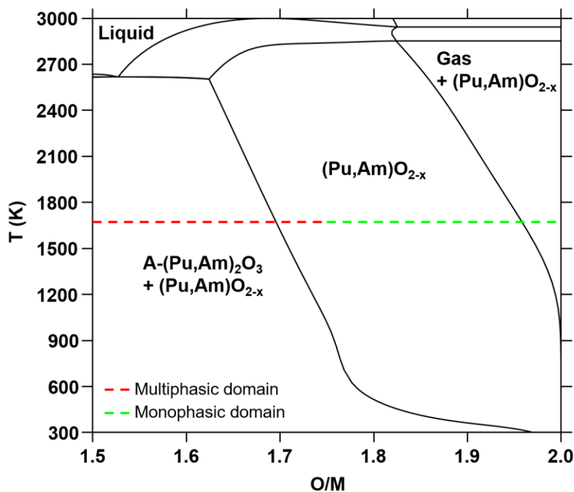
Figure 6-22: Isoleth section calculated for \text{Pu}_{0.77}\text{Am}_{0.23}\text{O}_{2-x} , compared to the domains evidenced by HT-XRD and ATG for the PuAm 80/20 sample.
