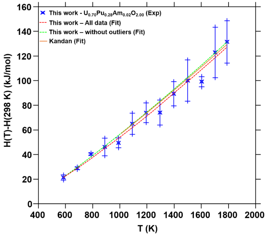
Figure 5-14: Different fits obtained in this work compared to the experimental values and the fit of Kandan et al. [135].
