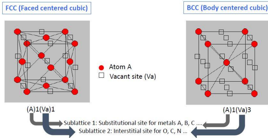
Figure 3-1: Representation of the sublattice model.
