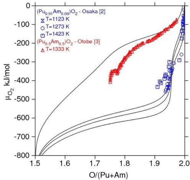
Figure 2-36 : Variation in the oxygen potential of \text{Pu}_{1-z}\text{Am}_z\text{O}_{2-x} as a function of the O/M ratio, the plutonium content and the temperature compared to the experimental values of Osaka et al. [43] and Otobe et al. [44] [26] and the calculated values of Gotcu-Freis et al. [26].
