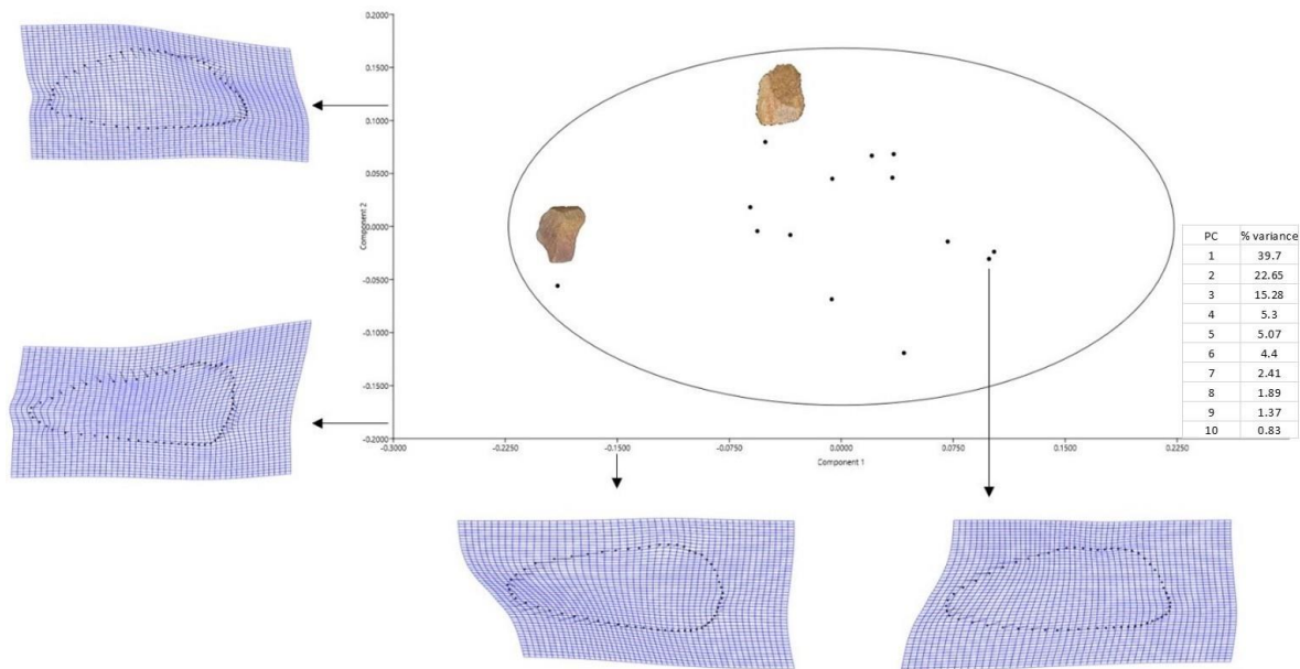
Figure 5. 30 Scatterplot showing the shape distribution along PC 1 and 2 with TpS deformations and the two cleaver blanks from Lakhmapur
