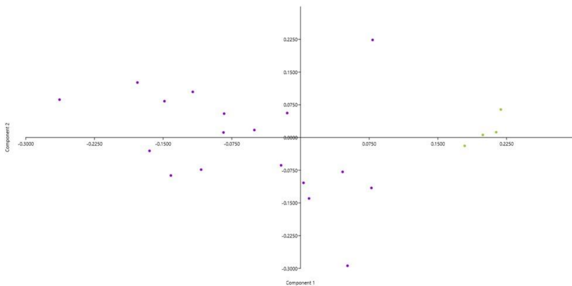
Figure 5. 35 Scatte plot displaying shape variations along PC 1 and 2 of all the cleavers from Attirampakkam (purple dot) and Singadivakkam (light green dot).
