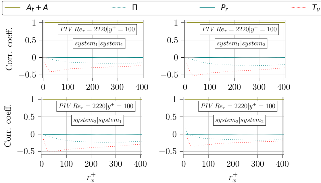
Figure 7.21: Correlation coefficient of KMHM equation terms with A_t + A in streamwise direction separation of PIV at Re_\tau = 2220 by using a combination of two systems ‘1’ and ‘2’ at y^+ = 100
