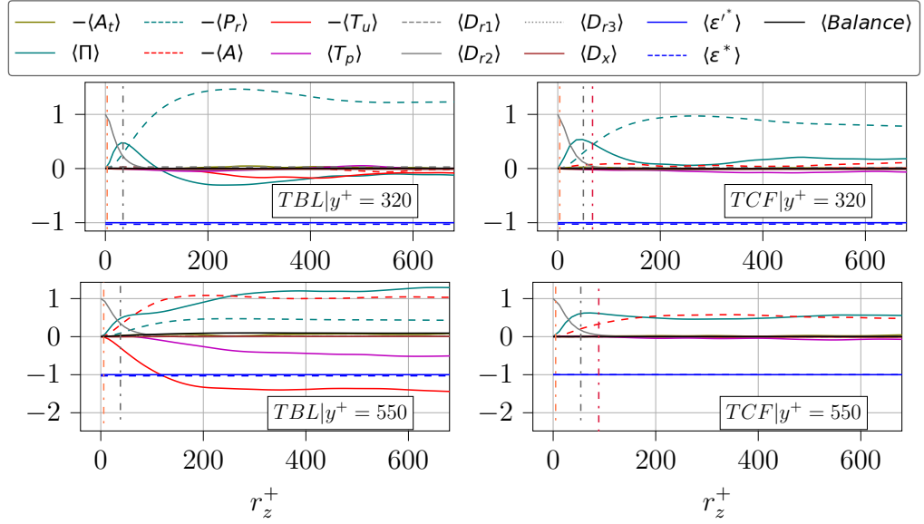
Figure 5.22: Spatio-temporal averaged values of all KHMH equation terms normalised by the absolute value of \langle \epsilon'^* \rangle in the spanwise direction separation in TBL550 (left) and TCF550 (right) at various wall distances. The wall distances and x-axes are normalised by wall-units
