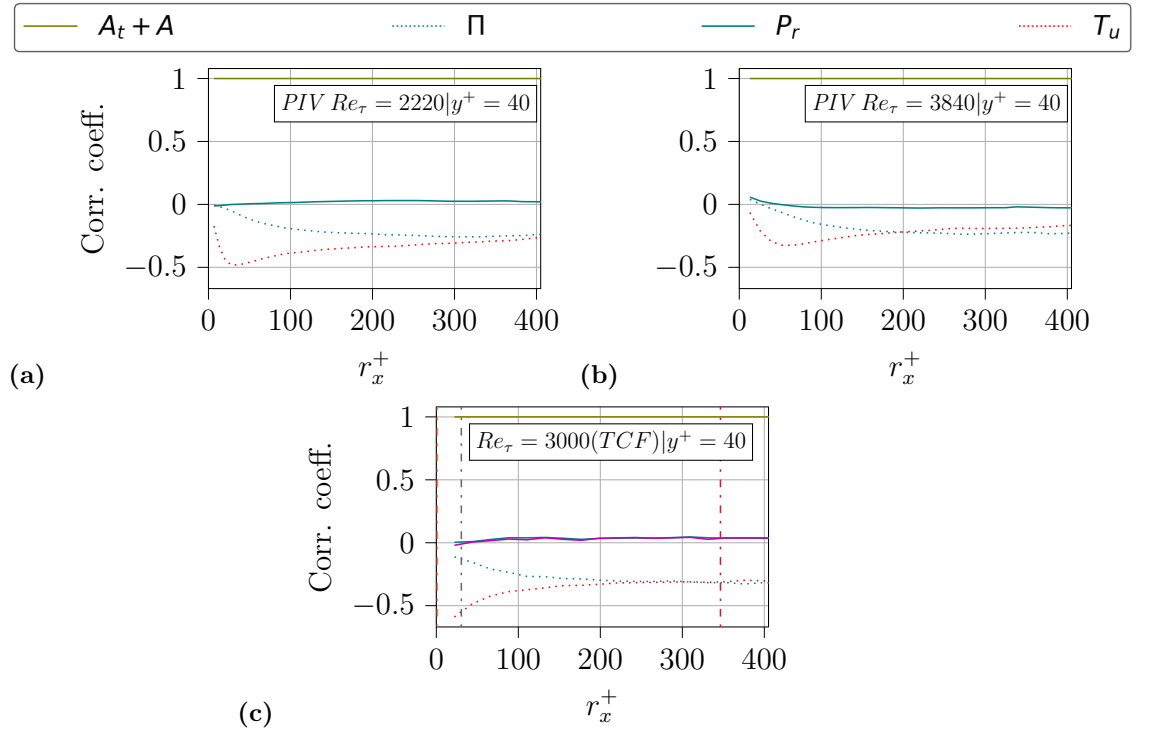
Figure 7.22: Correlation coefficient of the four KMHM terms with A_t + A in streamwise direction separation of PIV at (a) Re_\tau = 2220 , (b) Re_\tau = 3840 and is compared with the results of DNS of TCF at (c) Re_\tau = 3000 at y^+ = 40
