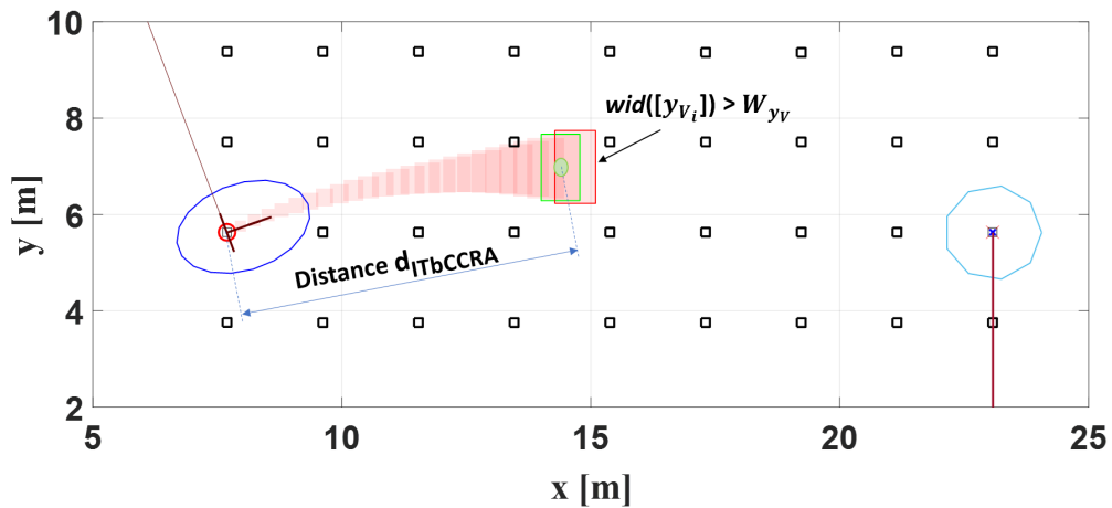
Figure 3.11: d_{ITbCCRA} calculation.
