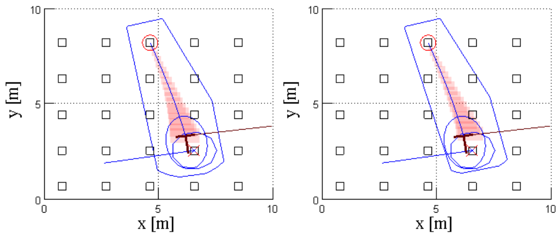
(a) Reachable space and vehicle trajectory without uncertainty injection.
