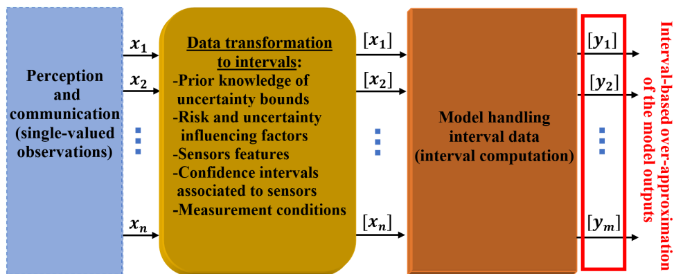
Figure 2.3: Interval process model.
