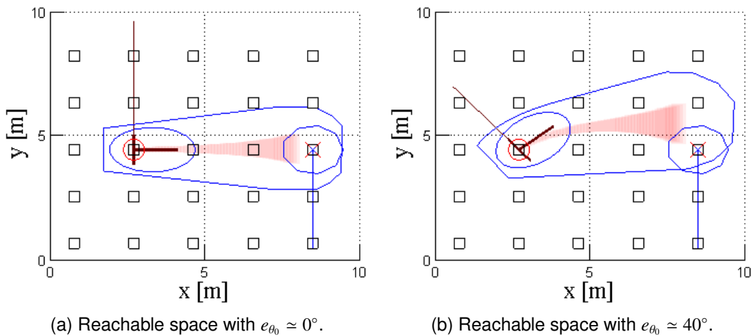
Figure 3.10: Reachable space behavior according to e_{\theta_0} .
