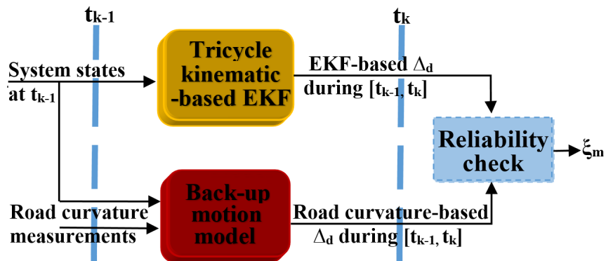
Figure 4.10: Reliability check for EKF modeling performances.
