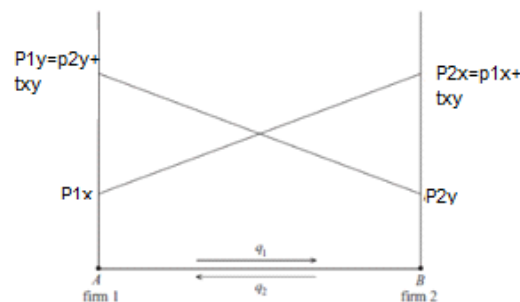
Figure 10: Spatial impossibility theorem
