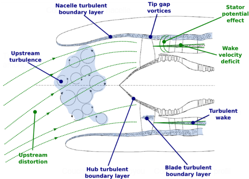
Figure 6: Sketch of the generation mechanisms of fan noise on turbfan engine from Moreau [63].
