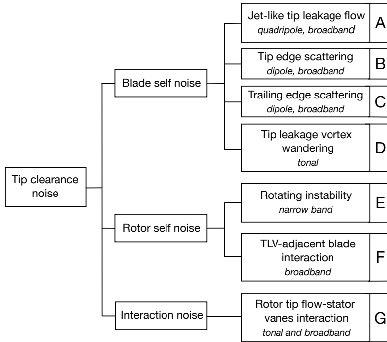
Figure 1.13: Classification of the aerodynamic mechanisms responsible for the generation of the TCN.
