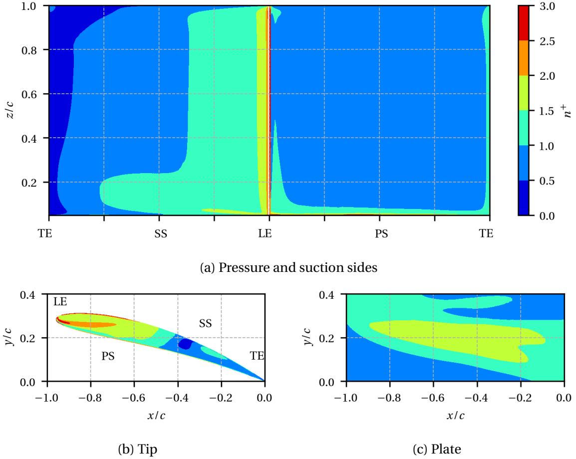
Figure 3.6: Wall resolution n^+ on the airfoil and lower plate for the RANS. PS: Pressure Side, SS: Suction Side, LE: Leading Edge and TE: Trailing Edge.
