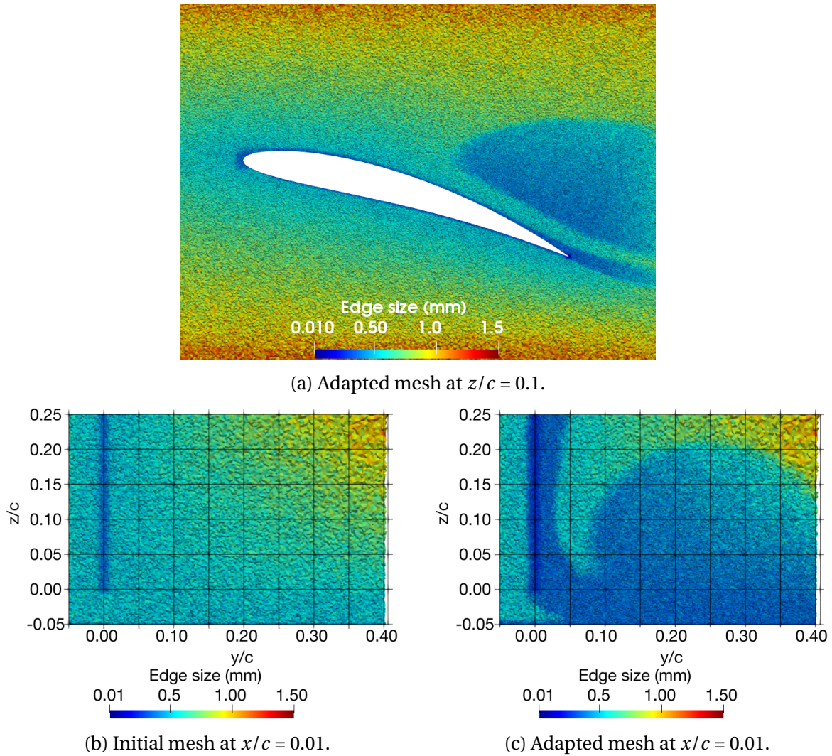
Figure 3.28: Mesh cuts before and after adaptation.
