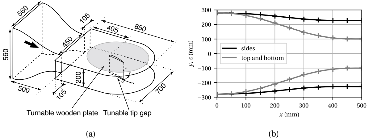
Figure 3.2: (a) Sketch of the single airfoil configuration with dimensions in millimeters adapted from Jacob et al. [46]. (b) Geometry of the nozzle with measurements in plus and extrapolation with hyperbolic tangent function in solid lines.
