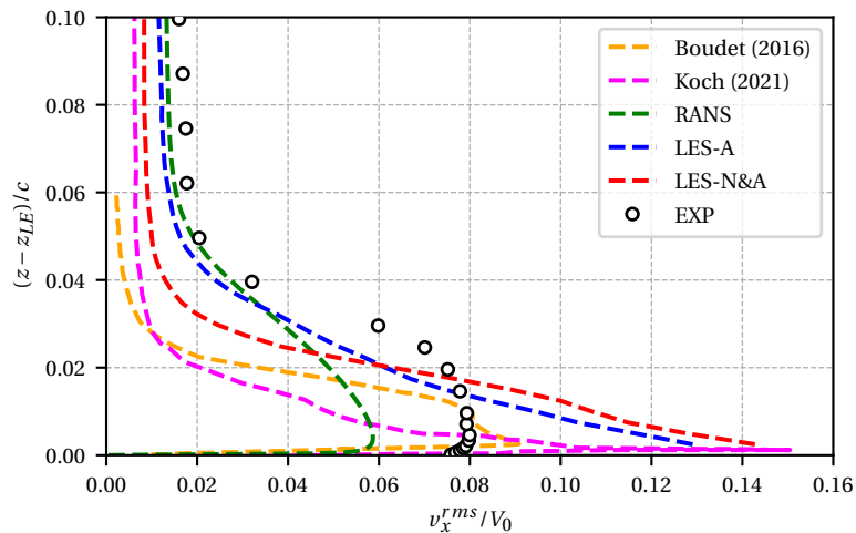
Figure 3.20: Profiles of streamwise velocity fluctuations v_x^{rms} at (x - x_{LE})/c = -0.5 and y/c = 0.14 .
