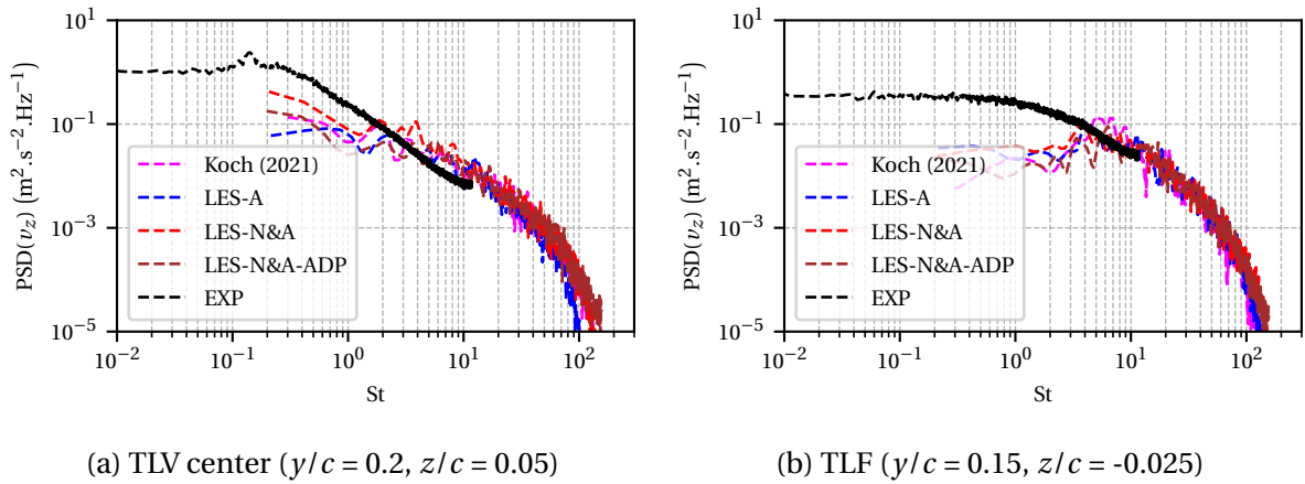
Figure 3.33: PSD of spanwise velocity component v_z .
