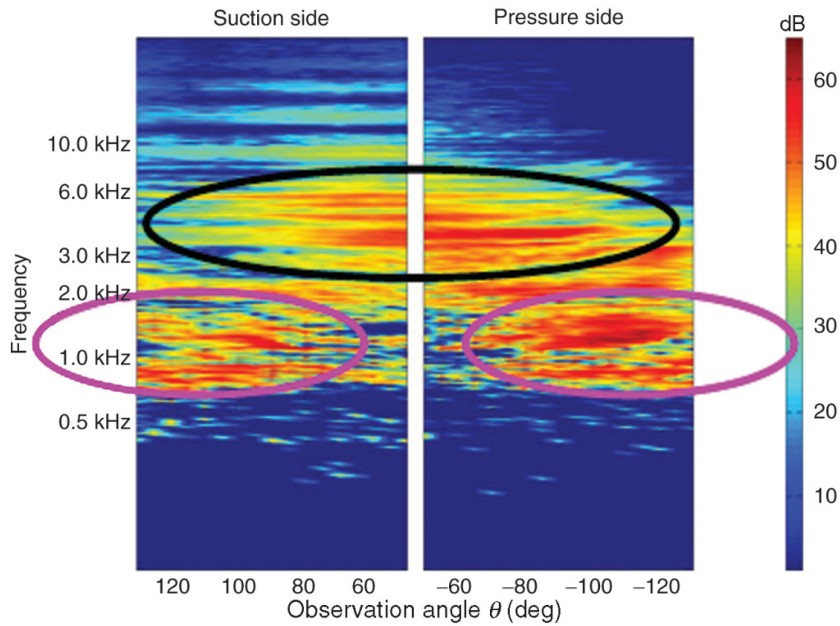
Figure 1.6: Tip clearance contribution to the far field against the observation angle and frequency. The color scale indicates the PSD level in dB-ref 4 \cdot 10^{-10} \text{ Pa}^2/\text{Hz} from Jacob et al. [45].
