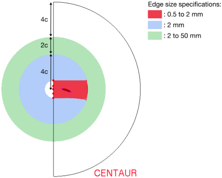
Figure 3.7: Volume mesh sources used to design the LES-A mesh with the meshing software CENTAUR .
