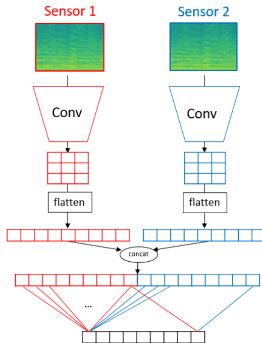
(c) Feature concatenation
