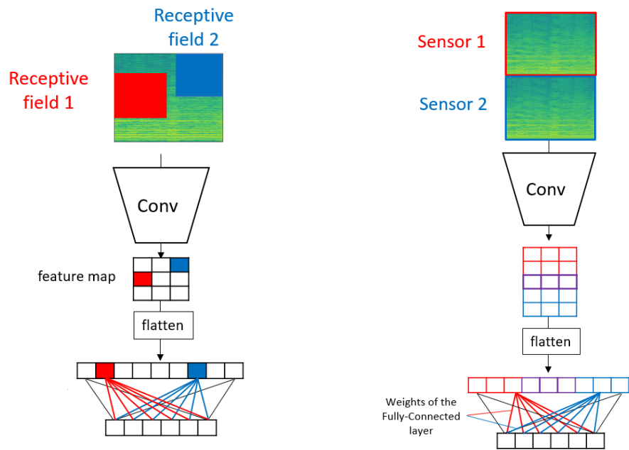
(a) How a neural network learns local features
