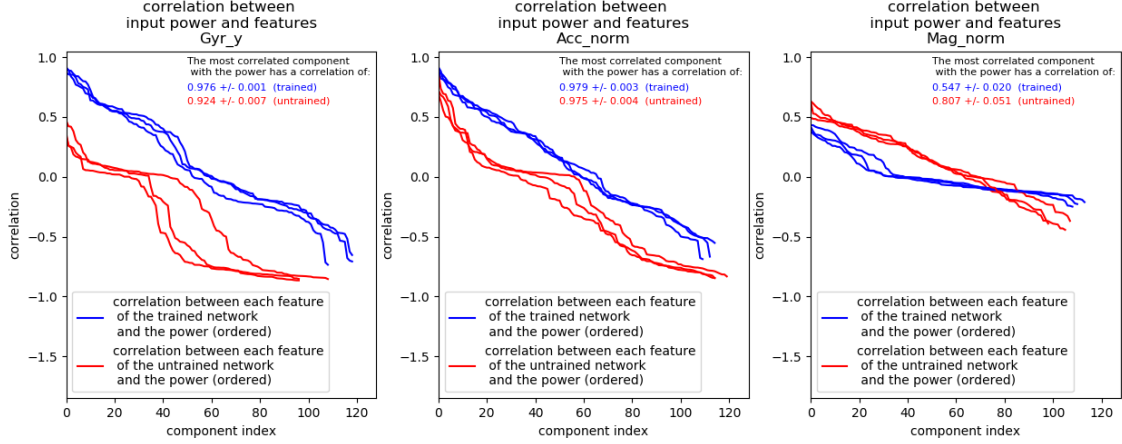
Figure 6.6: the correlation between each of the features and the power of the input signal
