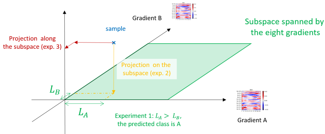
Figure 3.17: the three experiments we will lead to show the network classifies some classes linearly.
