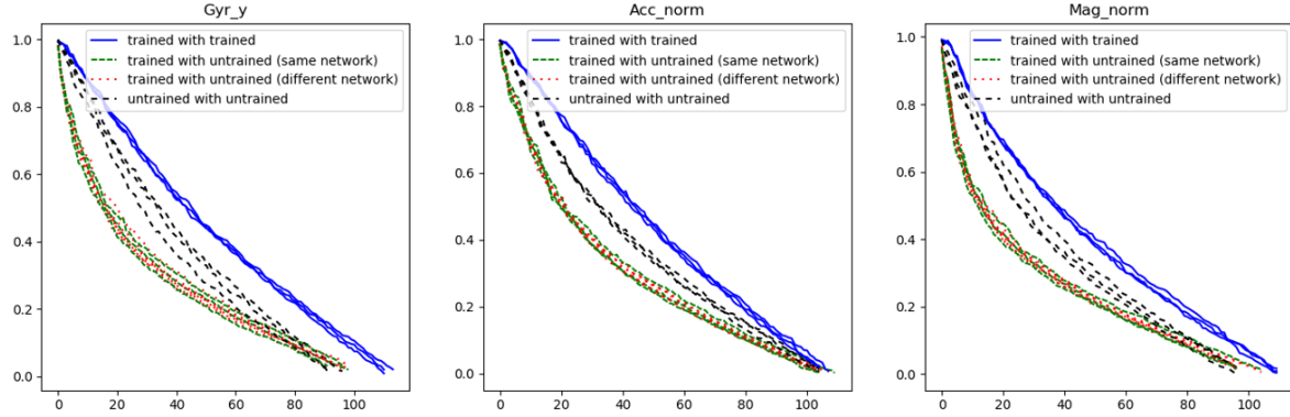
Figure 6.7: The correlation between different versions of trained and untrained networks, with SHL data.
