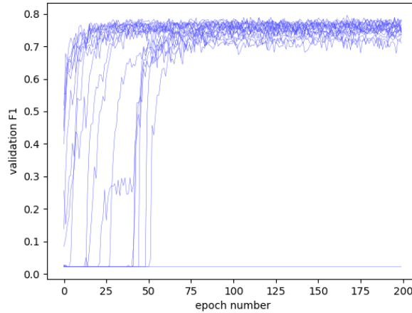
Figure D.1: The validation F1-score of 30 initializations of the same model working with full-size spectrograms of the Ori_w signal
