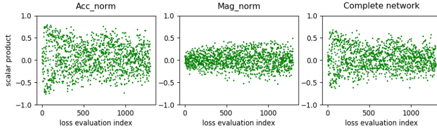
Figure 5.13: The scalar products between the classification and decorrelation losses at every batch, on the two-layer, deep CCA network
