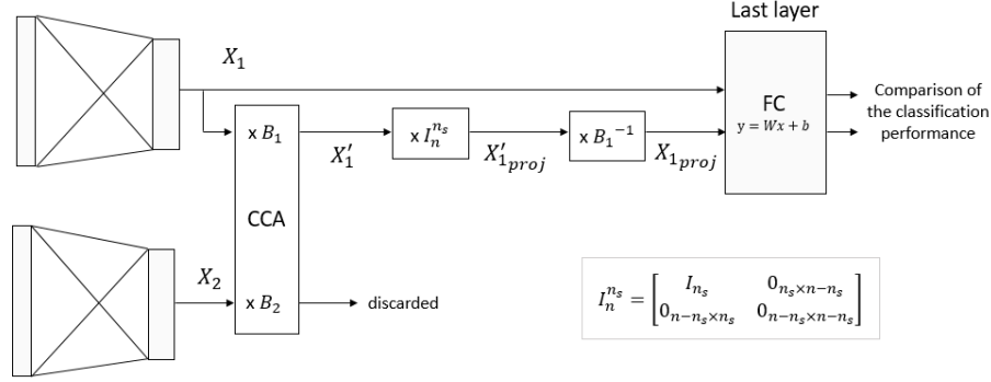
Figure 6.14: The principle of the subspace projection experiment, illustrated with the projection on the most correlated components (red curve in fig. 6.15): P_1 = B_1^{-1} \cdot I_{n_s} \cdot B_1 projects X_1 onto a linear space with dimension n_s . The value of n_s is a parameter we will modify in our experiments.
