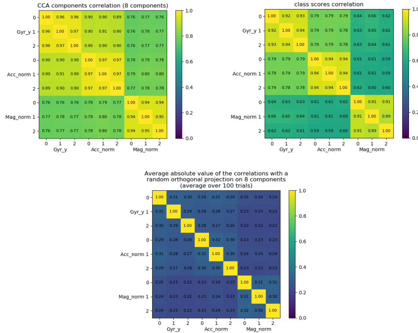
Figure 6.30: The average of the absolute values of the correlations (a) the first 8 CCA components (b) the 8 class logits (c) 8 directions chosen with a random orthogonal projection, with the SHL dataset. For each sensor, we create three different initializations of a network using the sensor. As expected by the intuition, the accelerometer and gyrometer feature and predictions are closer to each other than they are close to the magnetometer.
