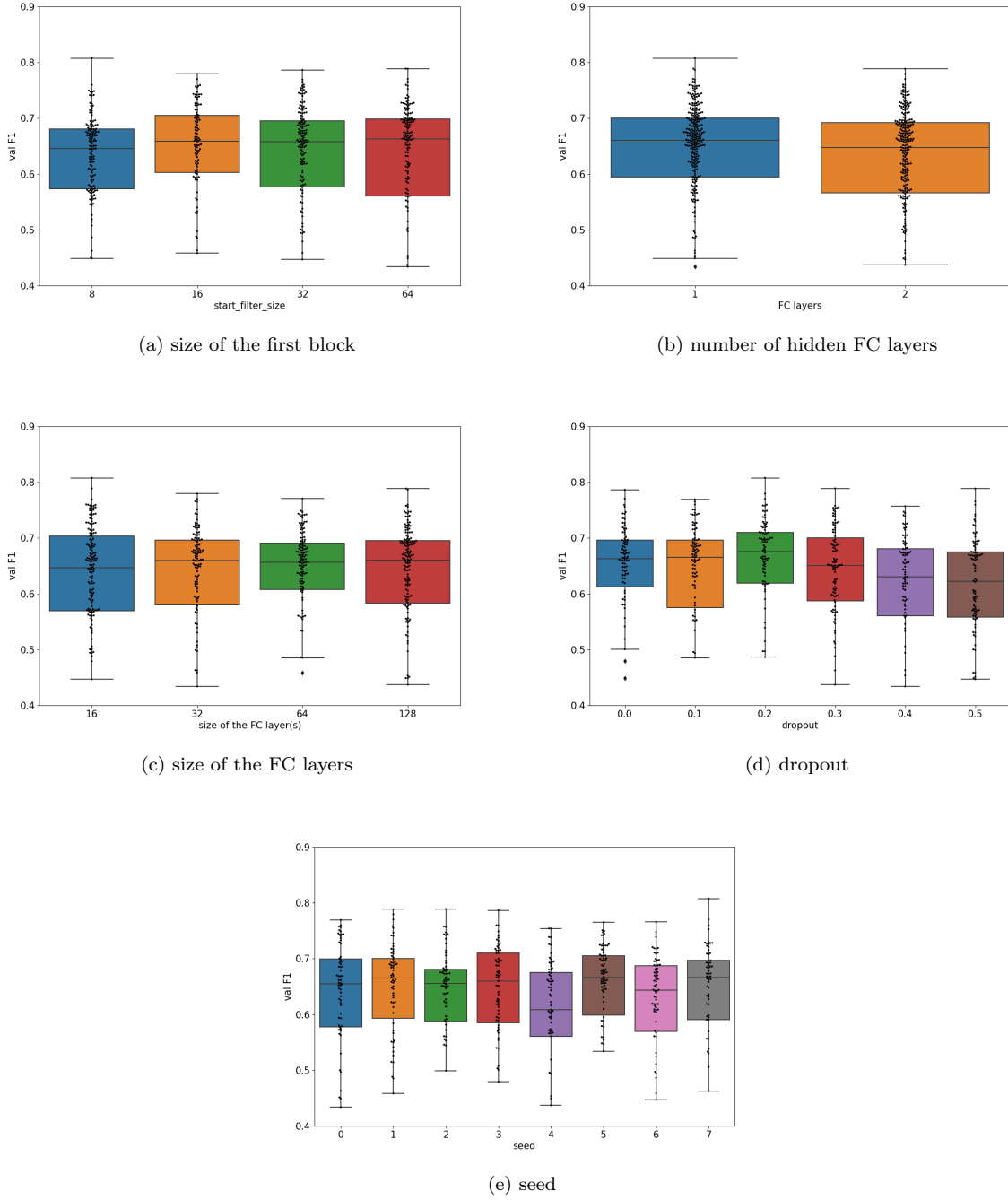
Figure C.3: The swarm plots representing the influence of all hyperparameters from random search. Each black dot represents one neural network.
