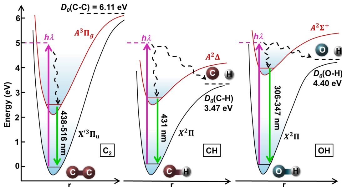
Figure 6.3-7 Diagram of transition processes of reactive radicles, C 2 , CH and OH, under the KrF excimer laser excitations.
