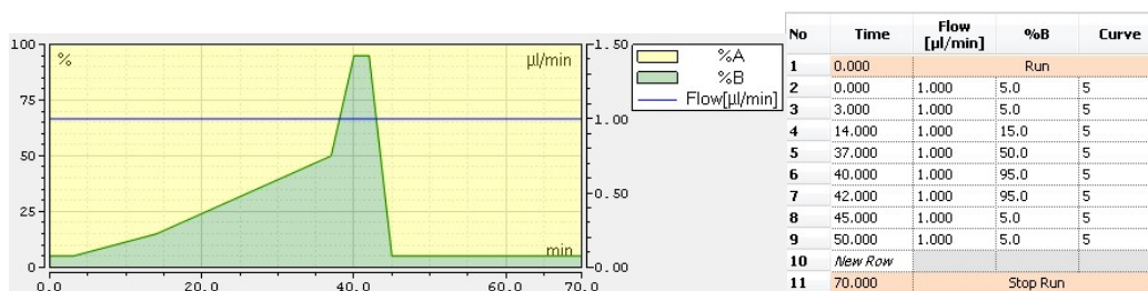
Figure III-5 70-minute gradient curve and flow rate.
