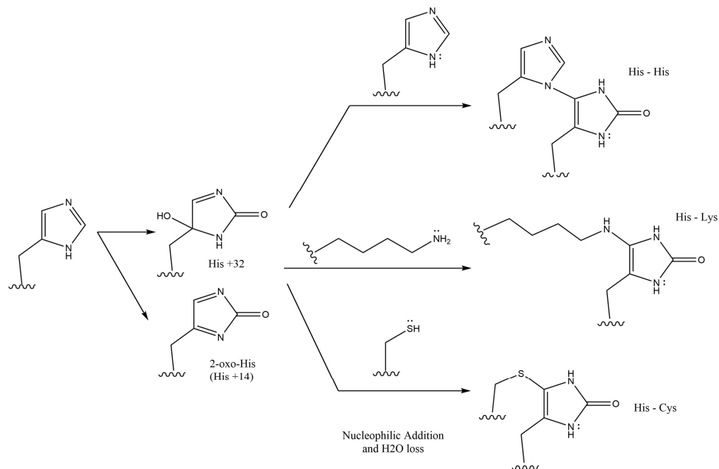
Figure IV-13 Proposed mechanisms of formation of His-His, His-Lys and His-Cys cross-links. Figure elaborated from Hägglund et al., 2018 with ChemPrime.
