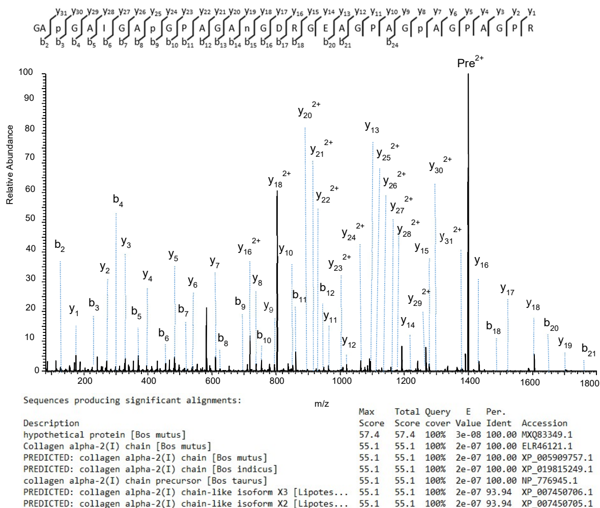
Figure V-6 MS/MS of the doubly charged precursor ion at m/z 1399.1604 attributed to the peptide (674 – 706) of collagen 2(I) from sample S1. The peptide sequence was identified through the full y-fragmentation pattern and b_2 - b_{18} , b_{20} , b_{21} , b_{24} fragment ions. Three hydroxyprolines (P3-P9-P26) and a deamidation (N15) were localised. The alignment of the experimental peptide sequence with all sequenced species present in the NCBI database provided the sequence's attribution uniquely to Bos taurus species.
