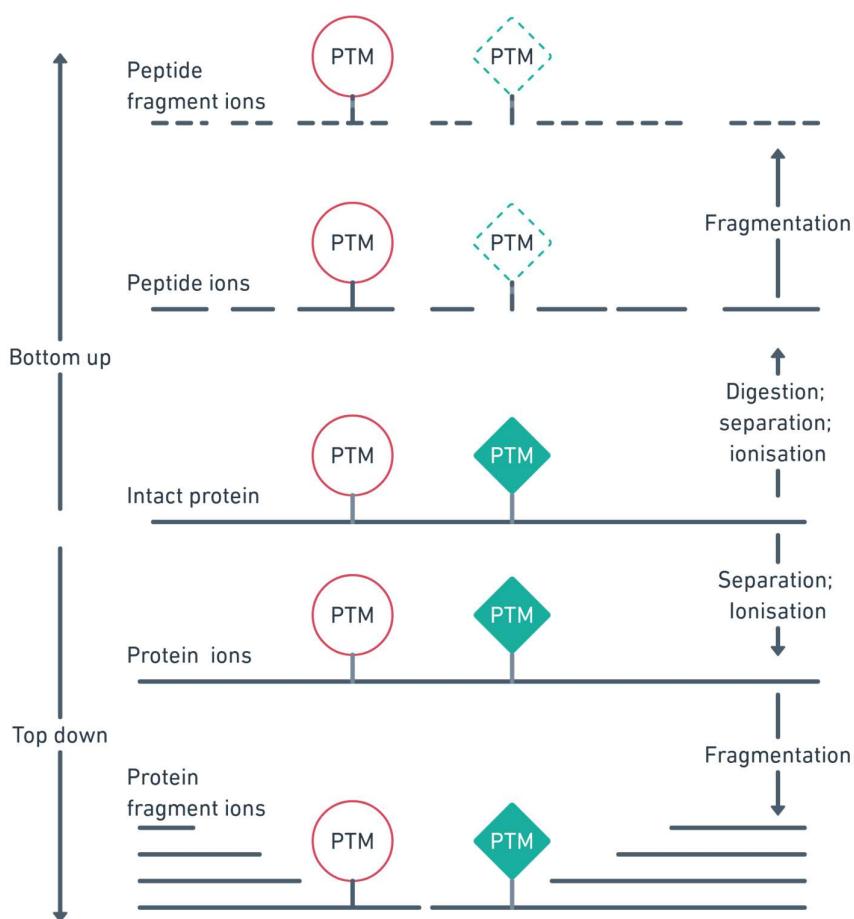
Figure III-1 Schematic representation of top-down vs bottom-up approaches. During the protein digestion into peptides in the BUP, some PTMs might get lost. Contrarily, top-down proteomics guarantees the preservation and identification of all PTMs present in the protein. Figure elaborated from Catherman et al., 2014.
