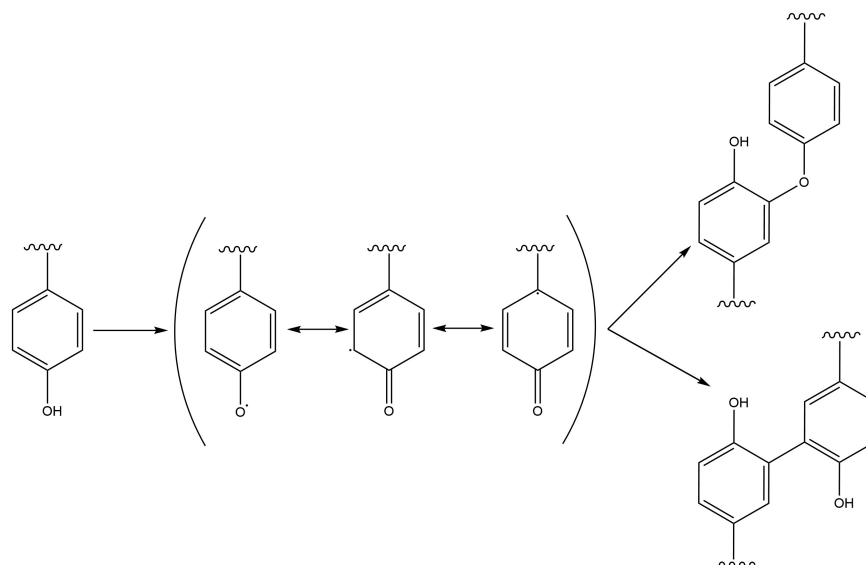
Figure IV-11 Proposed mechanism of Tyr-Tyr cross-links formation (di-tyrosine compound). The bond can involve carbon and oxygen (product at the top) or carbon-carbon (product on the bottom). Figure elaborated from Hägglund et al., 2018 with ChemPrime.
