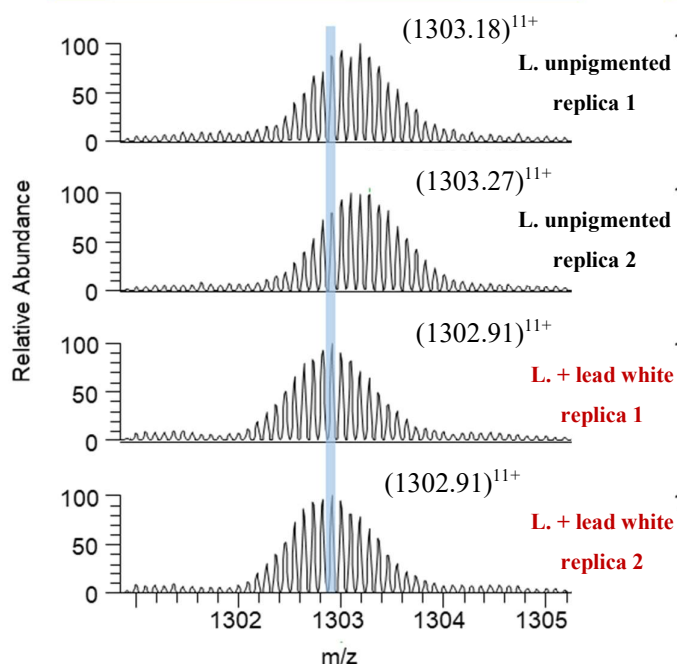
Figure IV-8 Magnification of the peak of 100% detected in lysozyme with and without lead white pigment. The distinction between the average masses of proteoform from both the first and second peak elutions was 3 Da which corresponds to three hydrogens exchange. For each sample, two experimental replicates are shown to prove the repeatability of the experiment.
