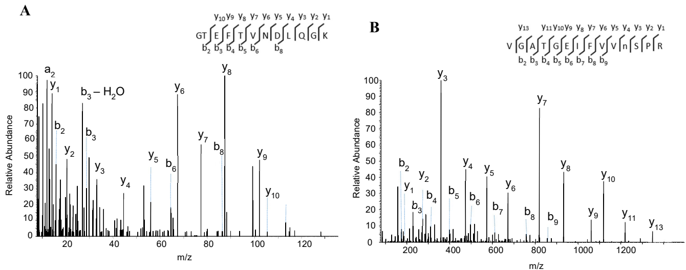
Figure II-6 MS/MS of (A) doubly charged ion at m/z 654.8245 ( \Delta m = -1.0 ppm) attributed to ovotransferrin in the sample US. 22_8c (church on Us Island, 10 th /11 th century). The sequence 120-131 was identified using y_1^+ to y_{10}^+ and b_2^+ to b_8^+ and b_8^+ , b_{12}^+ fragments; (B) doubly charged ion m/z 723.8826 ( \Delta m = 0.1 ppm) attributed to the peptide 642 VGATGEIFVVnSPR 655 of vitellogenin 1 from the sample Se_5_2 (Selib, end of 6 th /7 th century). A clear and almost full fragmentation pattern localised a deamidation on asparagine (N11).
