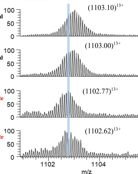
Figure IV-8 Magnification of the peak of 100% detected in lysozyme with and without lead white pigment. The distinction between the average masses of proteoform from both the first and second peak elutions was 3 Da which corresponds to three hydrogens exchange. For each sample, two experimental replicates are shown to prove the repeatability of the experiment.
