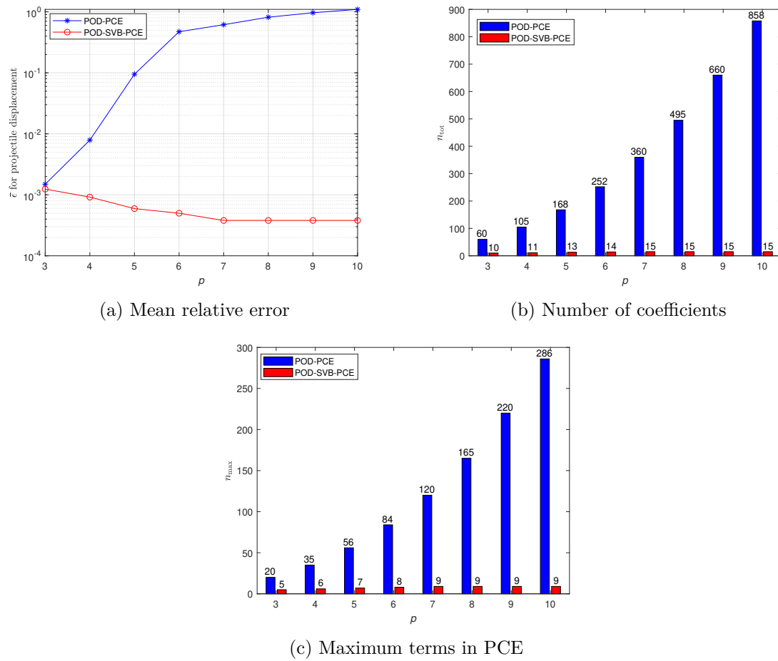
Figure 5.13: Evolution of the mean relative error and the PCE coefficients with the increase of polynomial degree p for the predicted projectile displacement by the POD-PCE and the POD-SVB-PCE models with N = 50
