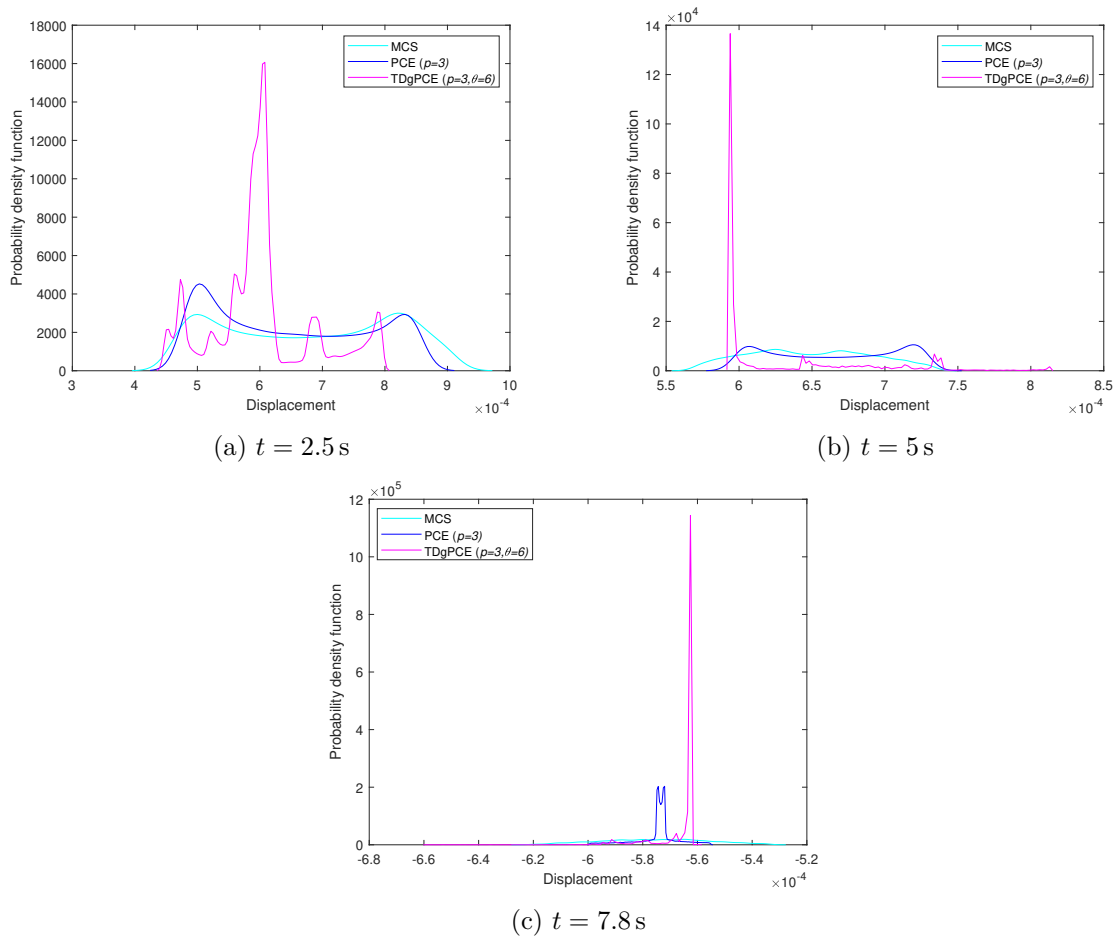
Figure A.7: PDF of displacement at different time instances for \bar{k} = 15000 \text{ N m}^{-1}
