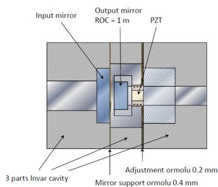
Figure C.1: Micro-cavity design.
