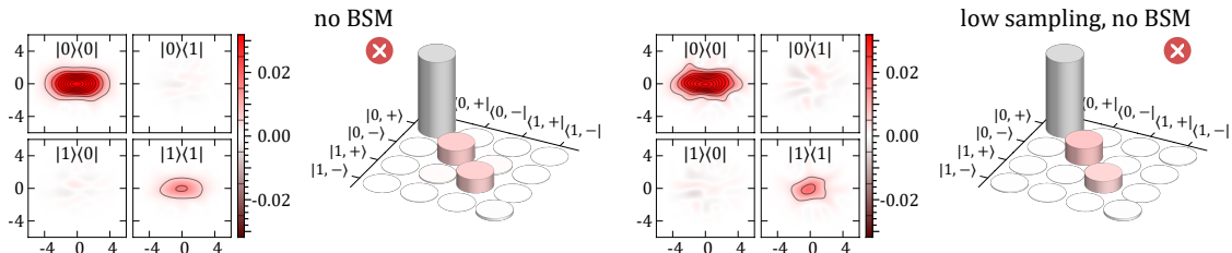
Figure 5.13: Downsampling the reconstructed state. (Left) Output state following no BSM. (Right) Output state following no BSM reconstructed from a downsampled data set matching that of the measured swapped state. The number of tomographic samples for each state reconstruction is 200 000 and 7800 respectively.
