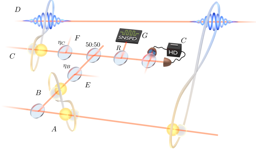
Figure 5.15: Model for the propagation of hybrid entanglement in lossy channels via swapping. The mode B of the DV-DV entanglement is mixed with an environmental mode E on a beamsplitter of reflectivity \eta_B , while the DV mode C of the hybrid entanglement is mixed with the mode F with a reflectivity \eta_C . The lossy modes are mixed on a 50:50 beamsplitter and the Bell-state measurement is performed by sending a fraction R of the light in the mode G to apply the bucket detection \sum_{n \geq 1} |n\rangle \langle n|_G , while homodyne conditioning is applied on mode C .
