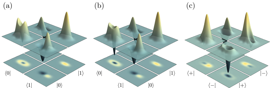
Figure 3.13: Experimental results in the symmetric case. (a) and (b) Wigner function of the reduced density matrices \langle i | \hat{\rho} | j \rangle_{DV} with \{i, j\} \in \{0, 1\} with and without detection losses of 15% in each mode. The components with i \neq j being not hermitian, the corresponding Wigner functions are not necessarily real, but conjugate. The plot gives therefore the real part in the back corner ( i < j ) and the imaginary part in the front corner ( i > j ). (c) Same results in the rotated DV basis \{|+\rangle, |-\rangle\} with |\pm\rangle = (|0\rangle \pm |1\rangle)/\sqrt{2} . The negligible higher photon number terms (the amplitude of which being lower than 1% for each) are not represented.
