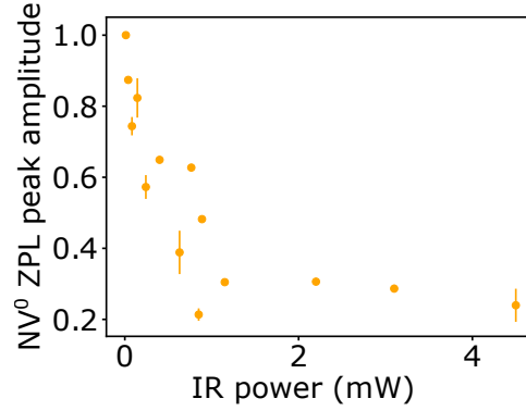
Figure 4.17: \text{NV}^0 ZPL Amplitude in CL with IR laser: the peak amplitude is divided by the current value to highlight the contribution of the IR power. The measurement is performed on a nanodiamond aggregate on a TEM lacey carbon grid kept at 150 K in the VG microscope. The \text{NV}^- CL peak is not seen.
