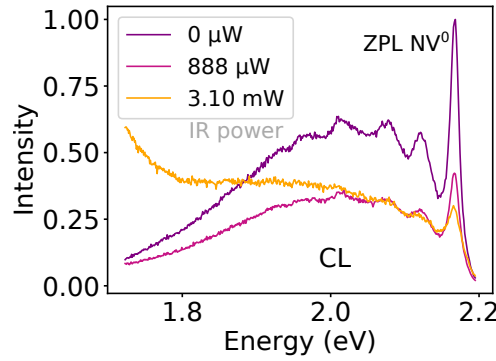
Figure 4.18: \text{NV}^0 CL emission at various IR laser power: the CL intensity decreases, and the ZPL of \text{NV}^0 becomes wider with increasing laser power.
