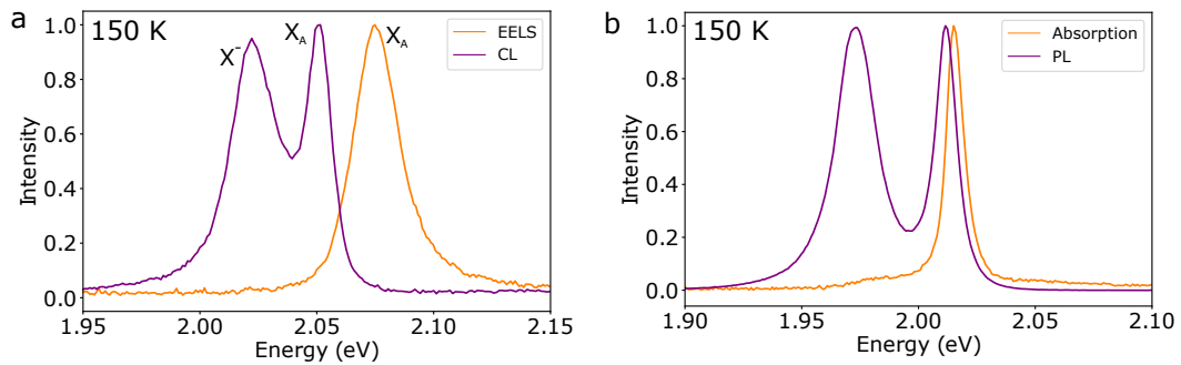
Figure 5.5: Comparison between spectra: (a) from electron excitation (b) from pure optical excitation. The measurements are done on encapsulated \text{WS}_2 monolayers at 150 K, performed on two different samples. The optical measurements curves (PL and absorption) were reproduced from [38] with permission.
