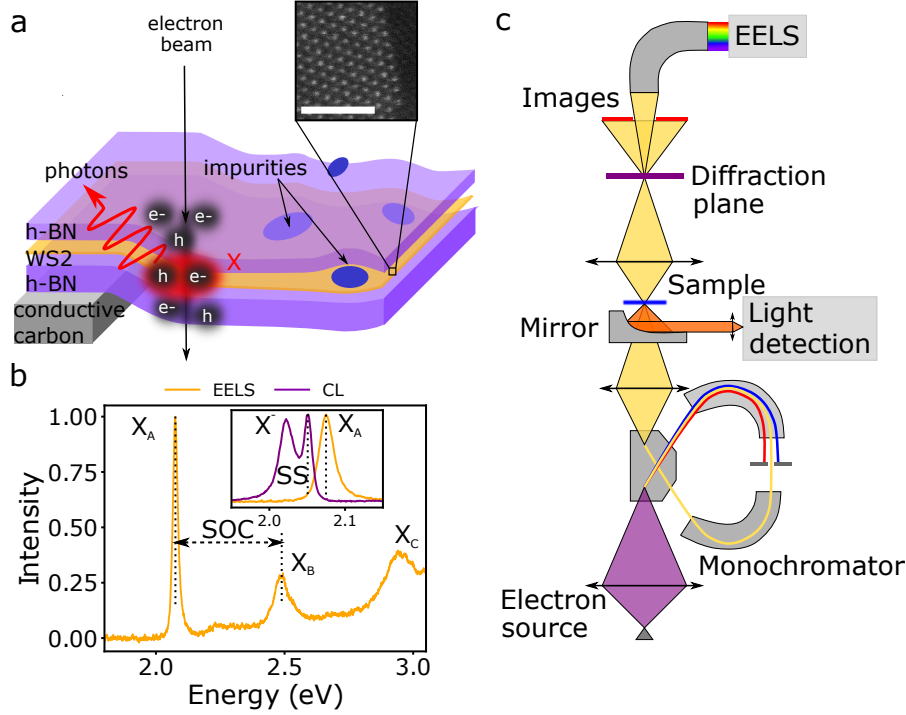
Figure 1.2: CL and EELS of a TMD monolayer: (a) Scheme of the TMD (WS 2 ) monolayer (orange) encapsulated in h-BN (purple), with the X A emission in red. The inset shows an atomically-resolved HAADF image of an edge in the encapsulated TMD monolayer (scale bar is 2 nm). (b) Typical EELS spectrum (orange curve) with the peak labels associated to different excitonic transitions excitons (X A , X B , X C ). A typical CL emission is shown on the inset (purple curve), where both X A and X A - are visible. The energy difference between the absorption (EELS) and emission (CL) of X A is the Stokes shift (SS), and that between X A and X B in the spin-orbit coupling (SOC). (c) Scheme of the STEM microscope used for the experiment. The monochromator allows for high energy resolution low-loss EELS absorption measurements. The light emitted from the sample upon electron excitation (CL) is collected by a parabolic mirror (NA= 0.5) and directed to an optical spectrometer. On the same setup diffraction patterns and images at different collection angles can also be measured in parallel to spectroscopic information. The measurements were performed with the sample kept at 150 K using a liquid nitrogen cooled sample holder.
