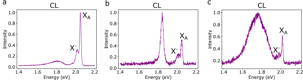
Figure 6.1: Examples of low-emission spectra in CL in the \text{WS}_2/\text{h-BN} heterostructure: spectra extracted from three different areas of a sample, displaying various spectral features at lower energy than X_A and X^- . The measurements are performed at 150 K.
