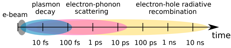
Figure 2.2: Scheme of the time-scale succession of events leading to CL: the electron beam excitation (e-beam, grey) is considered instantaneous. The plasmon decay (blue) occurs typically in the fs time-scale, followed by the electron-phonon scattering (pink), which occurs in the ps time-scale. Finally, the electron-hole recombination occurs typically in the ns time-scale.
