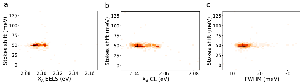
Figure 5.16: 2D histograms of the Stokes shift: (a) with the X_A energy in EELS, (b) the X_A energy in CL, (c) the FWHM of X_A in CL.
