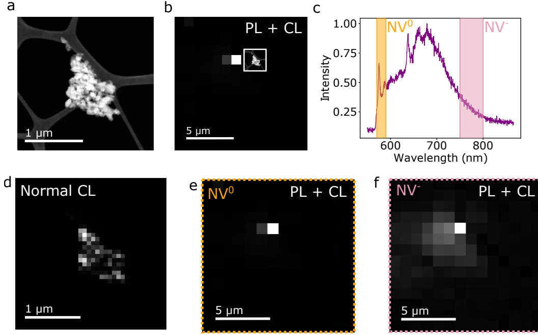
Figure 3.9: Mechanical hyperspectral acquisition, simultaneous measurement of PL and CL: (a) HAADF image of the FND aggregate with a size of the order of 1 \mu\text{m} , (b) mechanical hyperspectral image, with the ADF of the FND aggregate in inset to compare with the pixel size. (c) Spectrum extracted from the mechanical hyperspectral acquisition, where both the electron beam and the 543 nm laser were superimposed. (d) Usual spectrum image measured, where the electron beam is moved to scan the sample, with high spatial resolution, (e) energy filtered (570-590 nm) and (f) (750-800 nm) raster scan. The size of the pixel is 1 \mu\text{m} , which corresponds to the reproducibility of the sample motion.
