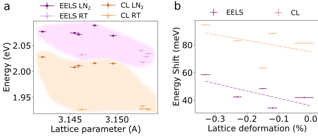
Figure 5.22: X_A energy in EELS and CL at two temperatures: (a) X_A energy as a function of WS_2 lattice parameter. (b) Energy shift \Delta E_{XA} = E_{XA,LN_2} - E_{XA,RT} as a function of relative lattice deformation \Delta a = a_{XA,RT} - a_{XA,LN_2}
