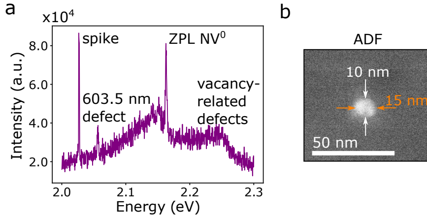
Figure 4.6: CL measurement of the smallest FND: (a) spectrum measured with the electron beam positioned on the FND, the defects emission contributions [60] are labeled on the spectrum, (b) ADF image of the FND.
