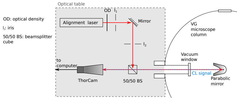
Figure 3.5: Alignment setup in VG: the alignment laser used is a He-Ne 633 nm red laser. The correct superposition of the CL and laser is controlled with a ThorLabs camera, with an objective that allows for the imaging of the mirror. A 50/50 beamsplitter is used to allow for the superposition of both signals.
