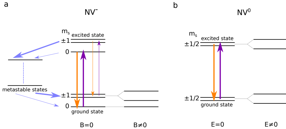
Figure 4.2: Energy structure of NV^0 and NV^- : (a) NV^- energy structure, the ground ( ^3A ) and excited ( ^3E ) triplet states degenerate, and the degeneracy of the m_s = \pm 1 levels can be lifted by Zeeman effect by applying a magnetic field. The m_s = \pm 1 levels are efficiently coupled to the singlet metastable states (top: ^1E and bottom ^1A ), which are non-radiative. Therefore, the optical transition from m_s = 0 level is brighter than that of m_s = \pm 1 . (b) NV^0 energy structure. The ground ( ^2A ) and excited ( ^2E ) states are two times degenerate, and form dipole transitions perpendicular to each other. The degeneracy of the levels can be lifted by Stark effect by applying an electric field [70].
