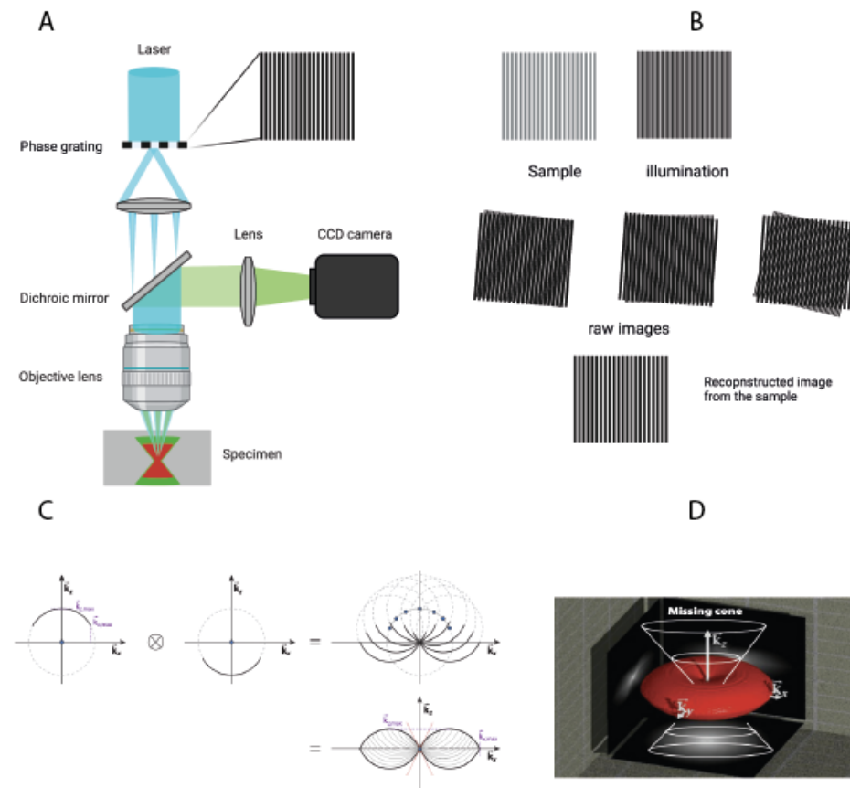
Figure 3.17: The schematic diagram of SIM and its principle. A) Laser light is modulated by a diffraction grating. The diffracted light is focused on the back focal plane of the high NA objective lens to generate a sinusoidal pattern. B) The grating is mechanically rotated to change the angle of the stripe pattern. The superposition of the stripe pattern with the sample creates an effect called Moiré: the overlap of two structures of high spatial frequency can generate a low spatial frequency. C)-D) The rotation of stripe patterns fills the missing cone and finally, a super-resolution image is reconstructed by computational methods, adapted from [118] .
