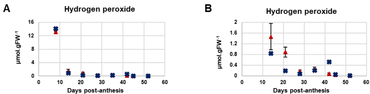
Supplemental fig V.8: Experimental mutant (red) and predicted values (blue) for \text{H}_2\text{O}_2 using median parameter from optimization procedure and after increase ascorbate synthesis (A). Same data but scaled-up (B).
