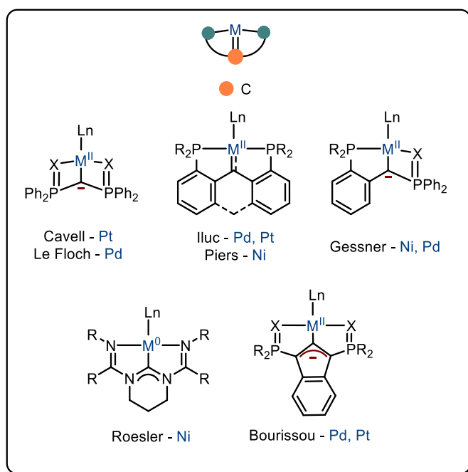
Figure I.3: Group 10 carbene complexes and analogs exhibiting MLC behavior
