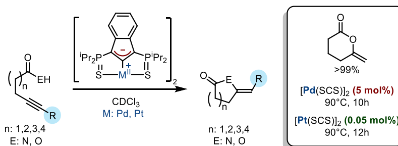
Scheme I.26: Cycloisomerization reactions catalyzed by the SCS-Pt II complex and reactivity comparison
