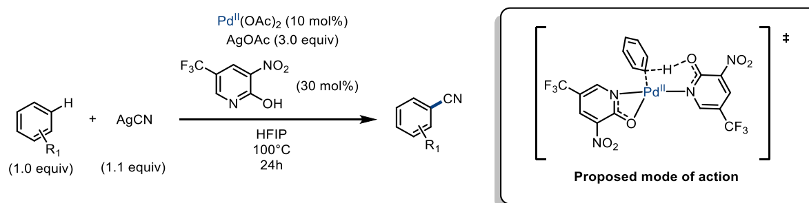
Scheme I.76: Catalytic non-directed cyanation of arenes by ligand assisted CMD
