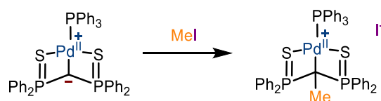
Scheme I.4: Nucleophilic character of Le Floch's Pd II carbene illustrated by reaction with MeI
