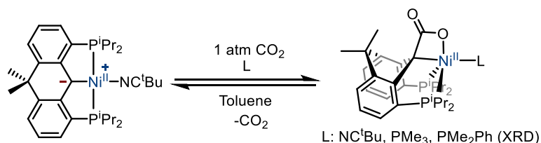
Scheme I.10: CO 2 activation and formation of metallactone with the Ni-Carbene of Piers.
