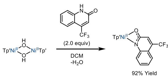
Scheme I.71: Synthetic pathway for the (Tp')-Ni II -quinolone complex reported by Jones
