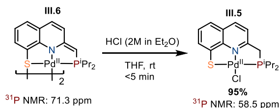
Scheme III.8: Regeneration of III.5 by protonation of the dearomatized dimer III.6 with HCl
