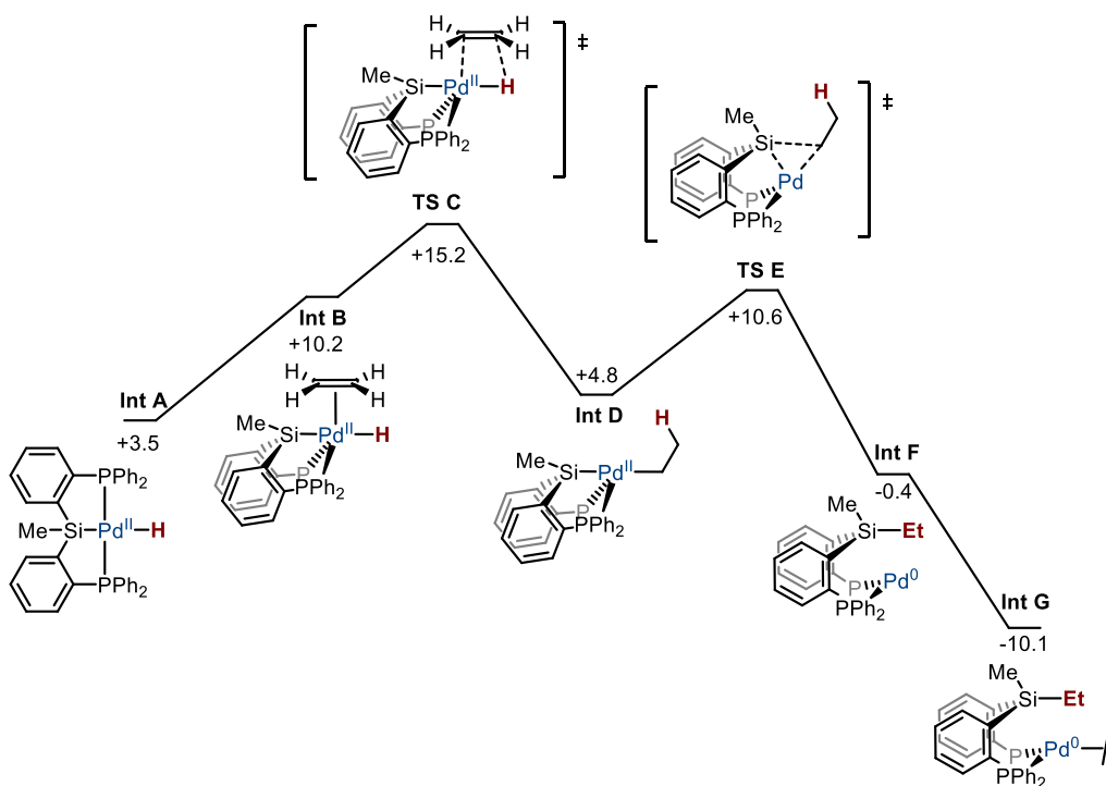
Scheme I.123: Proposed mechanism based on DFT calculations of the Si-mediated reductive elimination of Si-Pd II -Ethyl. (Energies are in kcal.mol -1 )
