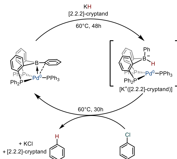
Scheme I.96: Hydro/deutero-dechlorination by the DPB-Pd 0 complex with transient breaking of the M->B interaction allowing for oxidative addition
