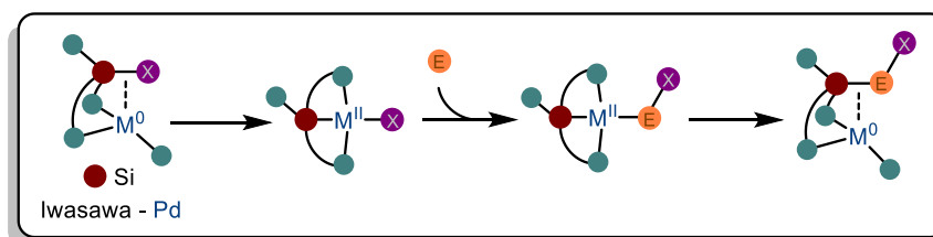
Scheme I.117: Schematic view of the non-innocent behavior of the Si-center in Iwasawa's complex
