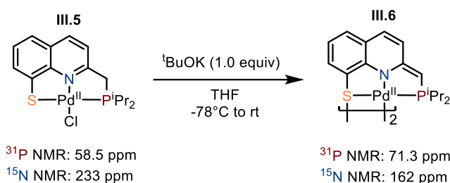
Scheme III.7: Deprotonation of III.5 with tBuOK to yield the well-defined dearomatized dimeric complex III.6
