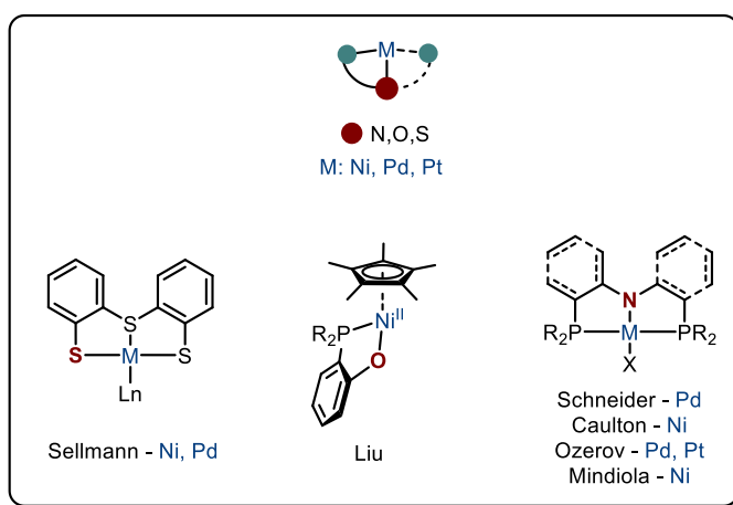
Figure I.11: Group 15-16 heteroatom tethered non-innocent complexes of group 10 metals
