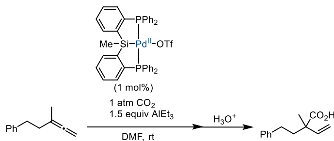
Scheme I.121: Catalytic hydrocarboxylation of allenes using the PSiP-Pd II -OTf complex
