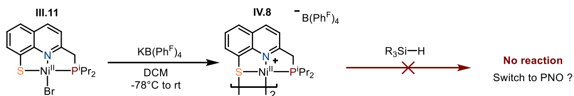
Scheme IV.28: Generation of a cationic PNS-Ni complex and Si-H bond activation
