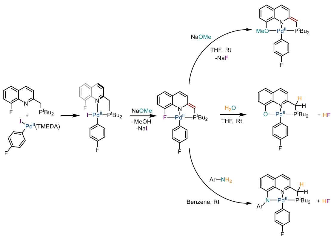
Scheme I.65: Synthesis of the dearomatized PNF-Pd II complex of Vigalok and stoichiometric E-H bond activation and SnAr
