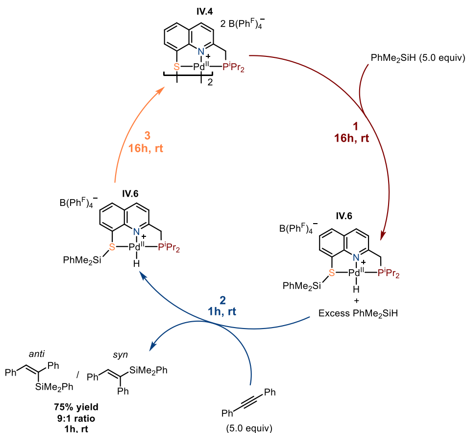
Scheme IV.16: Stoichiometric transfer of silane to Ph-CC-Ph by the complex IV.6 and regeneration of IV.4
