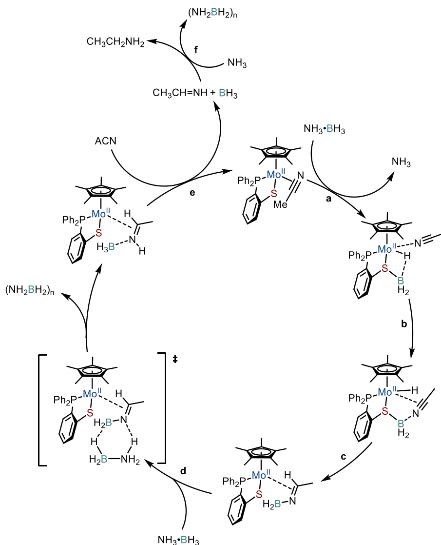
Scheme IV.11: Proposed catalytic cycle for the hydrogenation of nitrile with amine borane catalyzed by the Mo II -S complex of Wang
