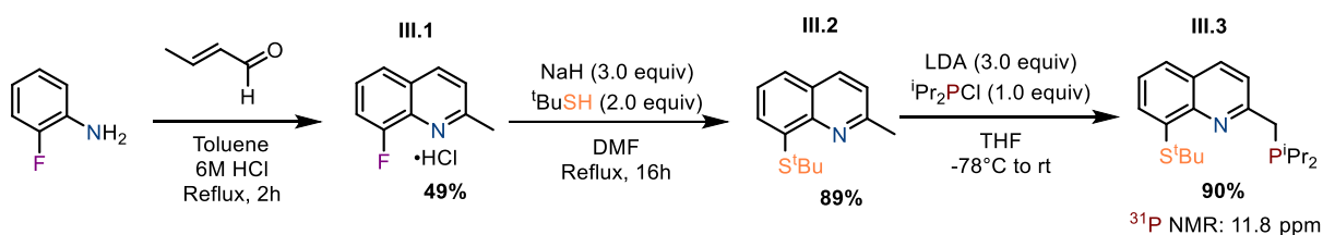
Scheme III.4: Synthetic pathway for the PNS tBu proligand in 3 steps starting from o -fluoroaniline
