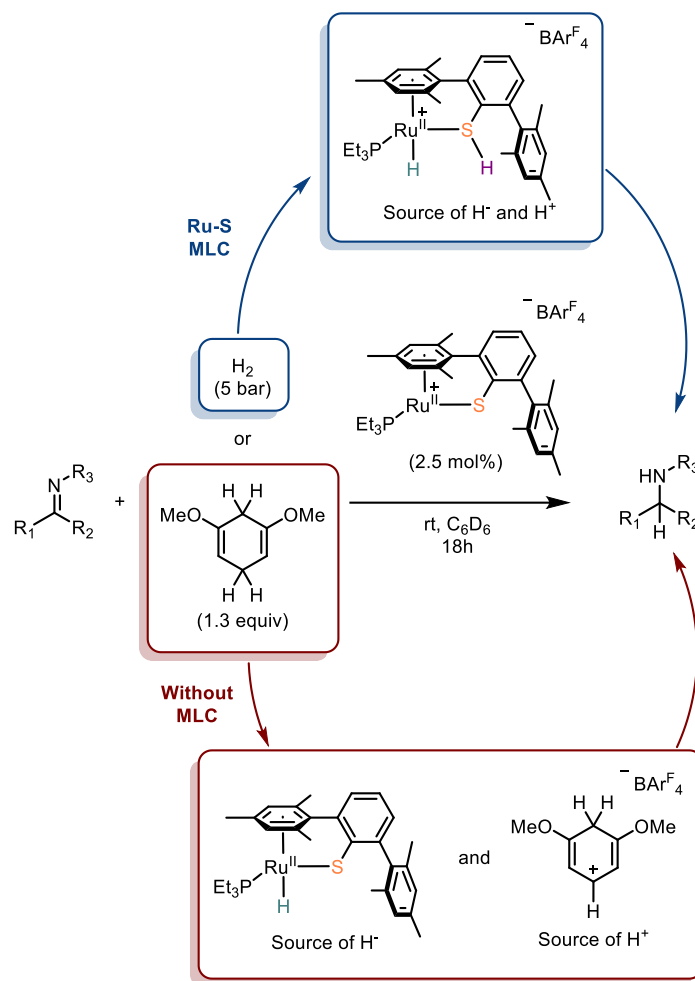
Scheme IV.2: Different mechanisms for the hydrogenation of imines, based on \text{H}_2 activation by MLC (top) or with the \text{DmpS-Ru}^{\text{II}} complex as a Lewis acid (bottom)
