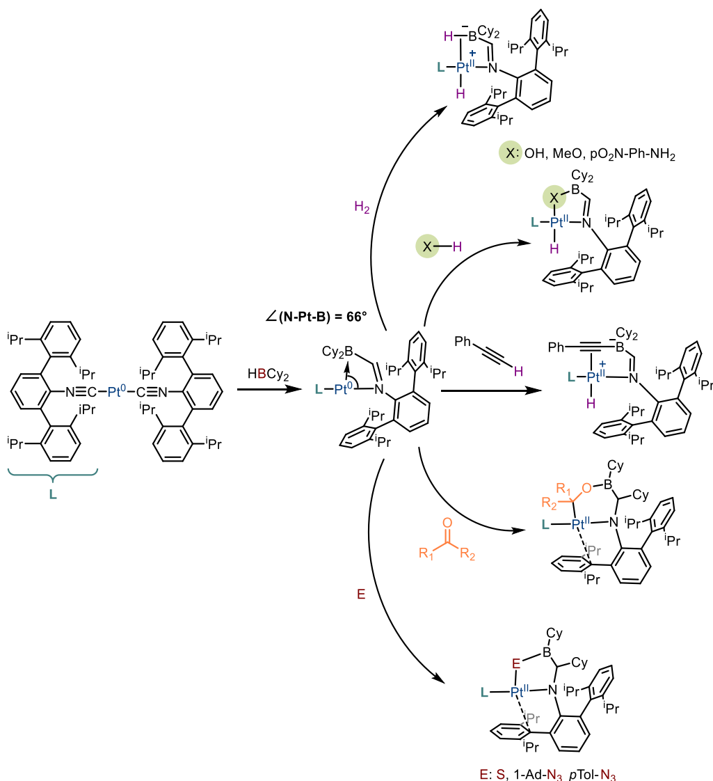
Scheme I.115: Versatile MLC reactivity by ring-strain release of Figueroa's Pt-B complex
