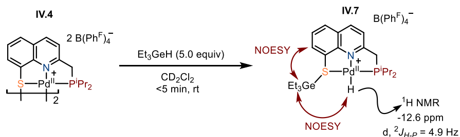
Scheme IV.25: GeH activation through Pd-S cooperativity with the cationic complex IV.4
