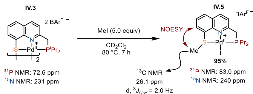
Scheme IV.14: Reaction of the cationic complex IV.3 with MeI and generation of the new IV.5 complex - This reaction was performed prior to the observation of the transmetallation in IV.3
