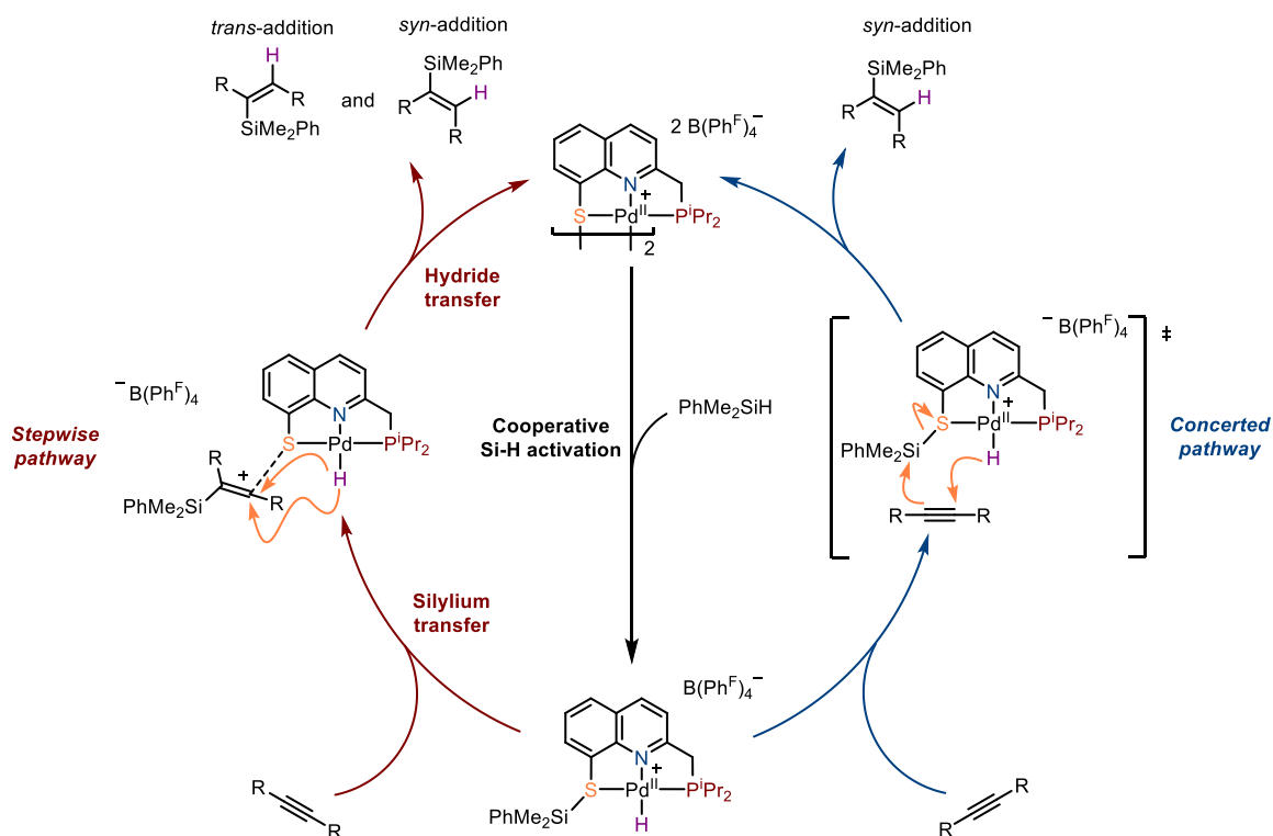
Scheme IV.20: Plausible simplified mechanisms for the hydrosilylation of alkynes by Pd-S cooperativity
