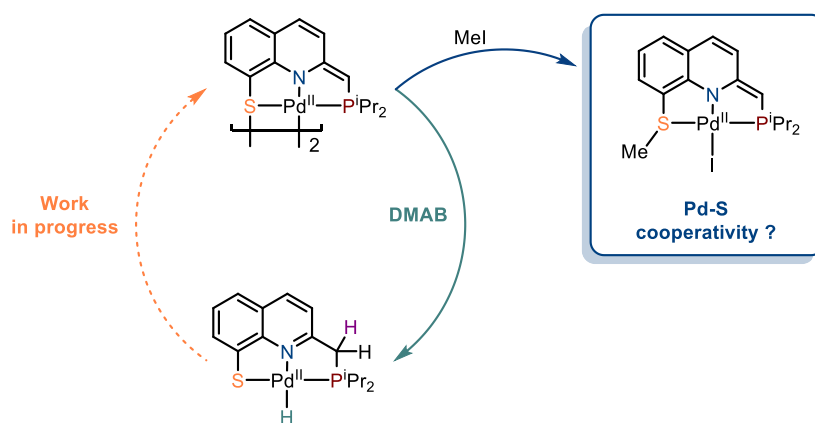
Scheme III.23: Challenges in closing the aromatization/dearomatization cycle and entry point to of Pd-S type cooperativity
