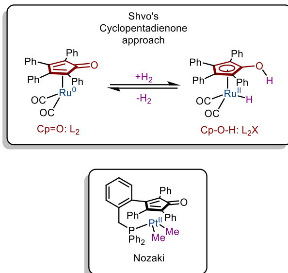
Scheme I.88: Comparison of Shvo's cyclopentadienone complex and Nozaki's approach
