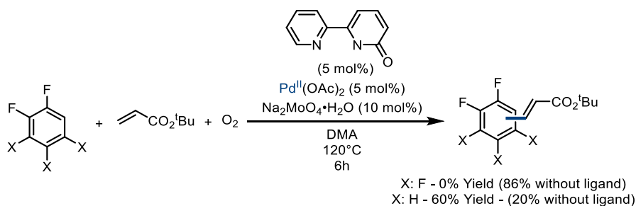
Scheme I.85: Comparison between activated and unactivated arenes in Albéniz's catalytic system with and without ligand
