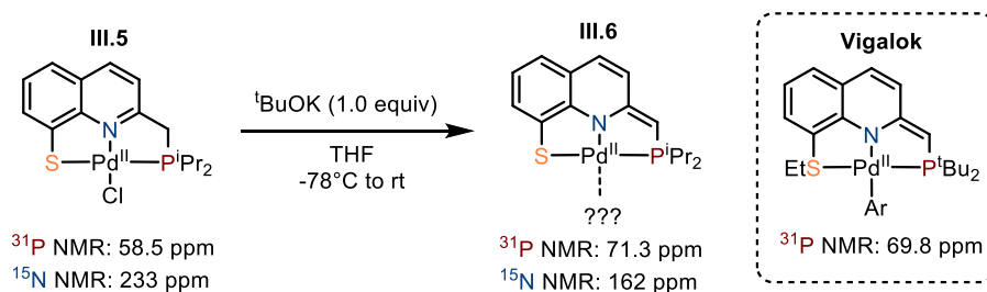
Scheme III.6: Synthesis of the dearomatized complex III.6 by deprotonation
