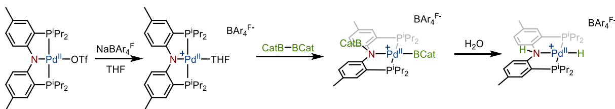
Scheme I.49: B-B bond activation and hydrolysis of Pd II -Boryl complex
