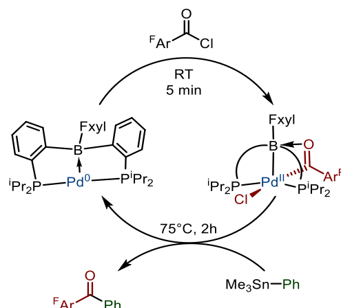
Scheme I.109: Chemo selective Stille-coupling with a beneficial effect of the DPB ligand
