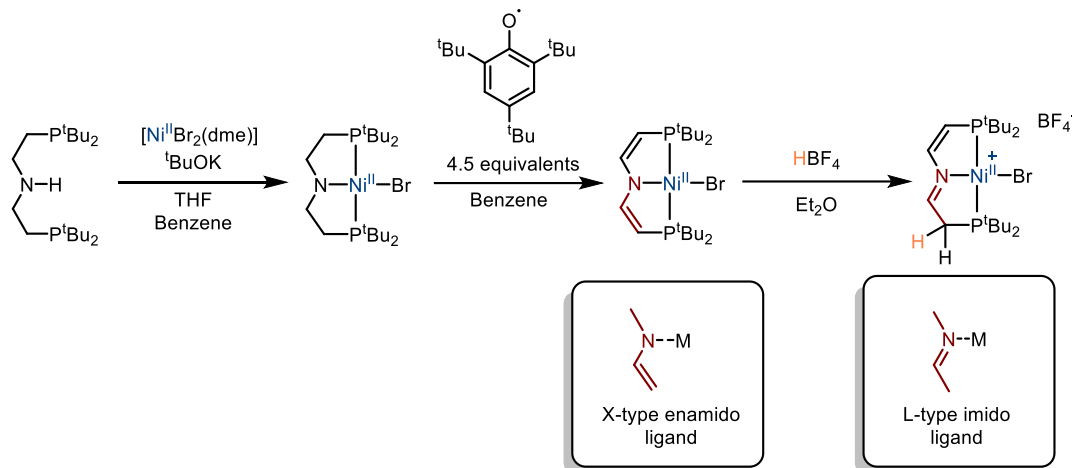
Scheme I.53: PNP-Ni complex of Schneider and reactivity towards acid
