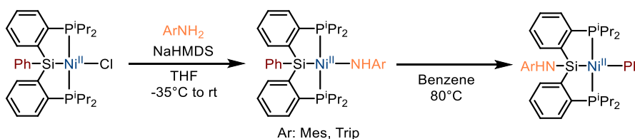
Scheme I.127: Synthesis of PSiP-Ni II -X complex and ligand exchange with silicon
