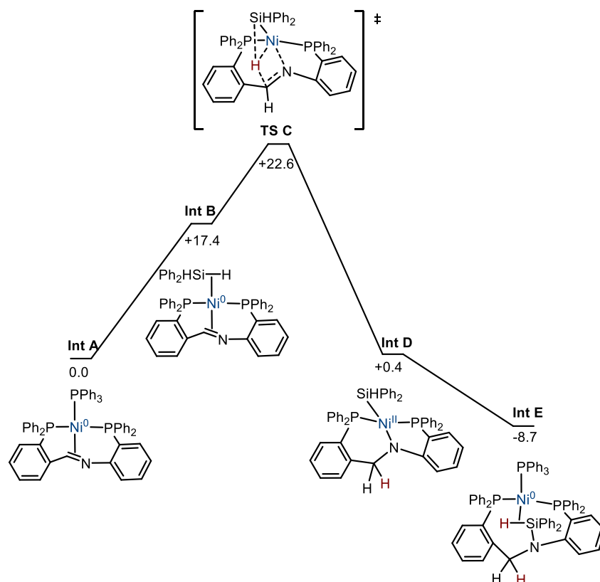
Scheme I.131: Proposed mechanism of the chemically non-innocent Si-H bond activation by the Ni 0 -imine complex based on DFT calculations
