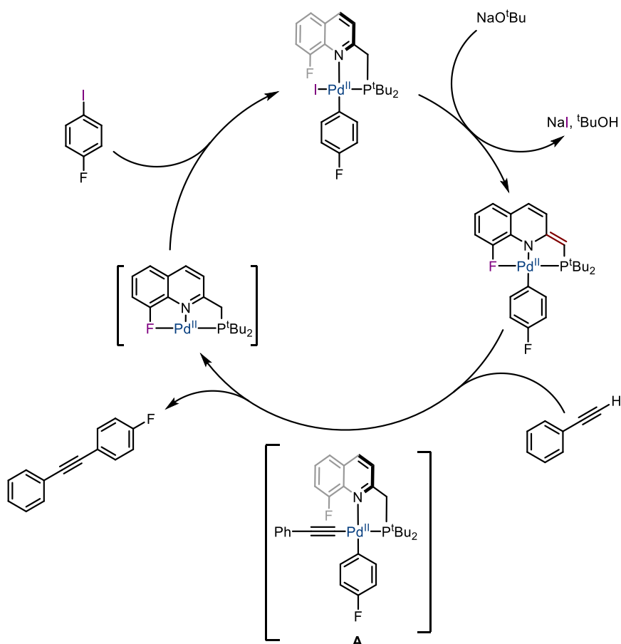
Scheme I.68: Proposed catalytic cycle by Vigalok for the catalytic copper-free Sonogashira-type cross-coupling
