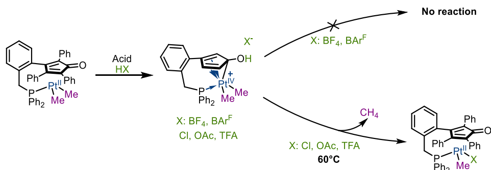
Scheme I.90: Nozaki Pt-C sp3 protonation and protonolysis of C sp3 -Pt bonds with cyclopentadienone Pt II complex
