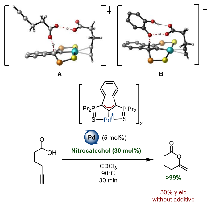
Scheme I.29: A - Calculated transition state of the substrate-assisted deprotonation event; B - Calculated transition state for the catechol-assisted deprotonation; Reactivity comparison with and without proton-shuttling additive
