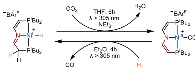
Scheme I.55: Two step reversed water-gas shift reaction
