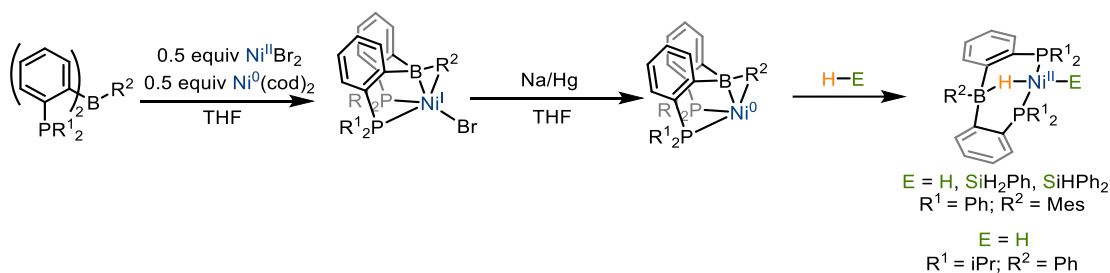
Scheme I.104: Boron-assisted E-H bond activation in DPB-Ni 0 complexes
