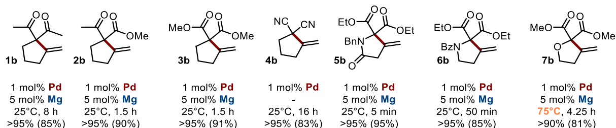
Figure II.4: 5- exo cyclization of terminal alkynes; isolated yields are indicated in brackets
