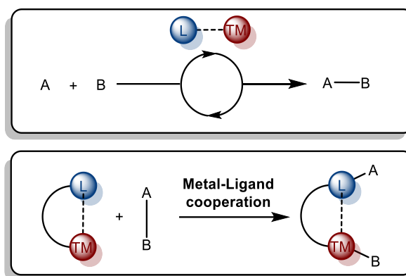
Figure 2: General view of “classical” TM-catalysis and chemical non-innocence in Metal-Ligand cooperativity
