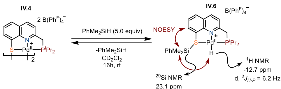
Scheme IV.15: Reversible Si-H activation by the dicationic dimer IV.4 and spectroscopic features
