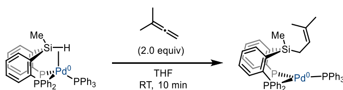
Scheme I.119: Allene insertion into the Si-H bond on the Pd 0 pincer complex of Iwasawa
