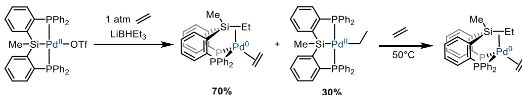
Scheme I.122: Generation of Pd-H and insertion of ethylene with subsequent Si-assisted reductive elimination
