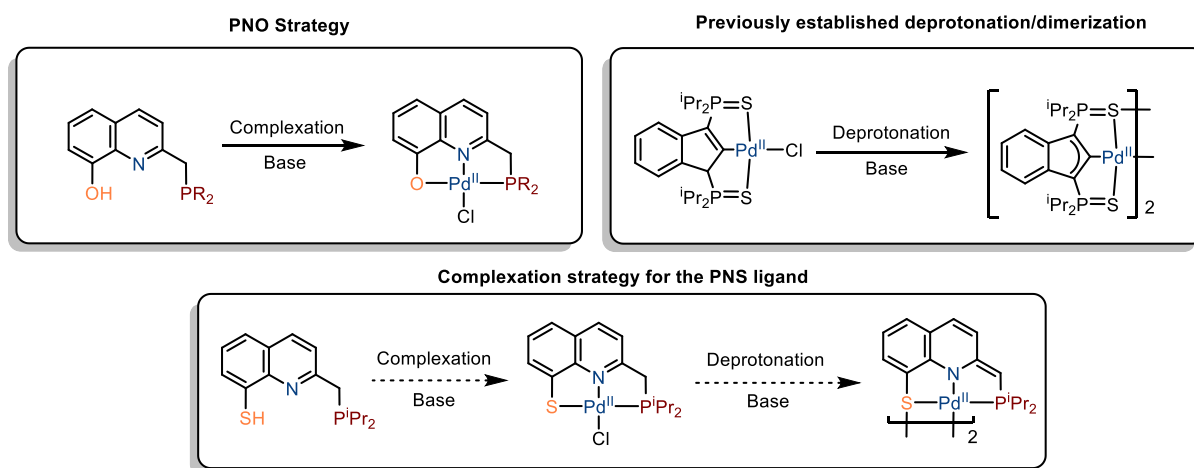
Scheme III.3: New PNS-Pd target complex and potential benefits of switching from oxygen to sulfur
