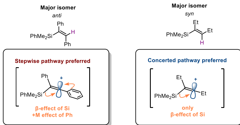
Scheme IV.21: Formation of a carbocation and resulting stabilizing effects in the case of tolane and in the case of hex-3-yne.
