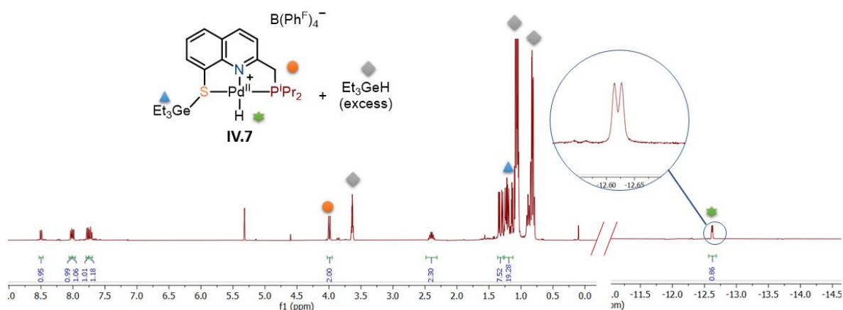
Figure IV.9: ^1\text{H} NMR of IV.7 after reaction of IV.4 with 5.0 equivalents of \text{Et}_3\text{GeH} in \text{CD}_2\text{Cl}_2
