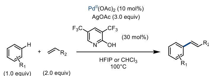
Scheme I.75: Heck-type coupling of arenes with Yu's non-innocent Pd II complex
