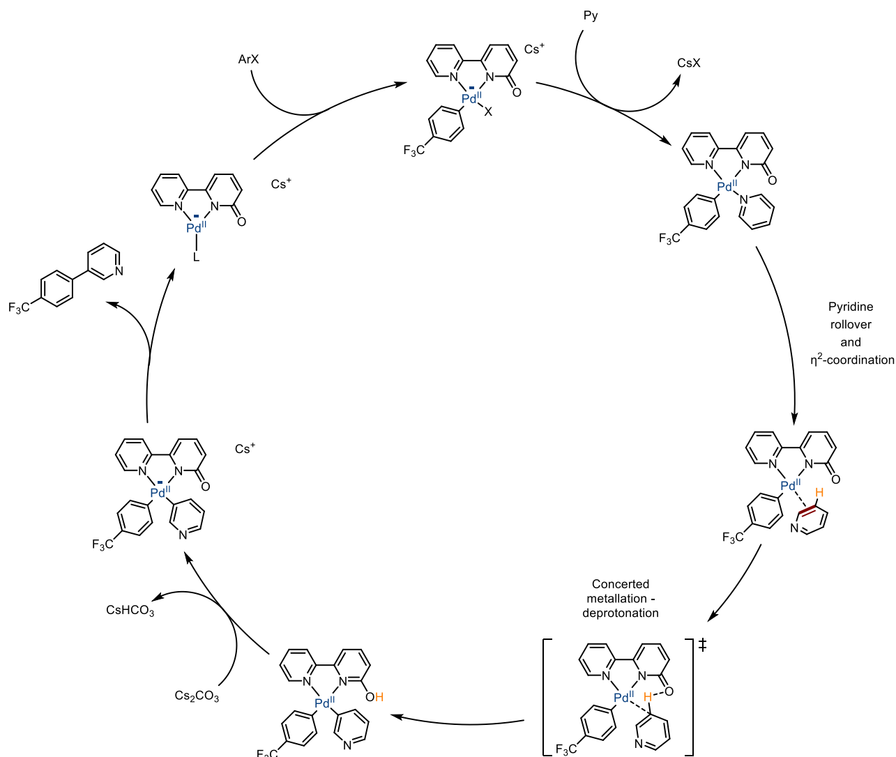
Scheme I.82: Catalytic cycle of the Ar-Py cross coupling reaction described by Albéniz
