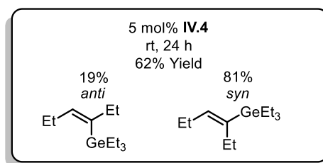
Figure IV.10: Hydrogermylation of symmetric hex-3-yne using IV.4
