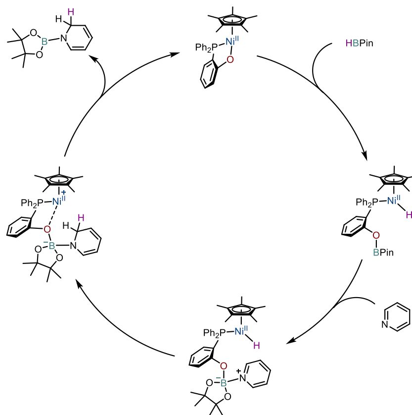
Scheme I.41: Mechanism of the 1,2-hydroboration of pyridines by the Ni-O complex of Liu
