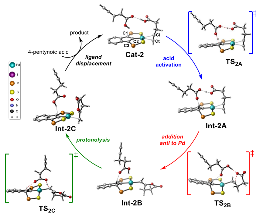
Scheme 1.28: Catalytic cycle of the cycloisomerization of alkynoic acids catalyzed by the chemically non-innocent SCS-Pd complex; Reproduced from Ref [30] with permission from the Royal Society of Chemistry.
