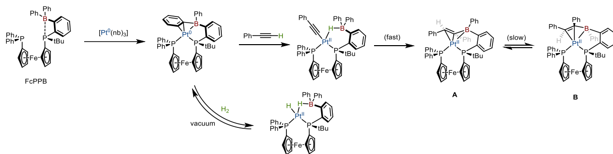
Scheme I.112: H 2 and C-H activation at a FcPPB-Pt 0 complex and Pt II -alkynyl isomerization
