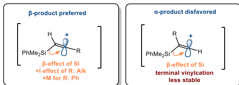
Scheme IV.24: Stabilization of electronic vacancy in the case of the hydrosilylation of aryl and alkyl substituted terminal alkynes
