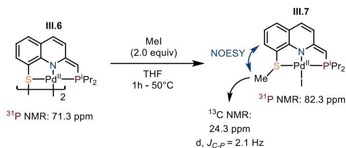
Scheme III.9: Reaction of the dearomatized complex at S with electrophiles
