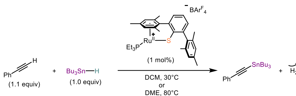
Scheme IV.26: Catalytic dehydrogenative stannylation of terminal alkynes with the DmpS-Ru complex
