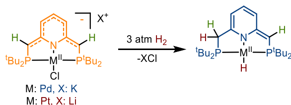
Scheme I.60: H 2 activation by the anionic Pd and Pt PNP complexes
