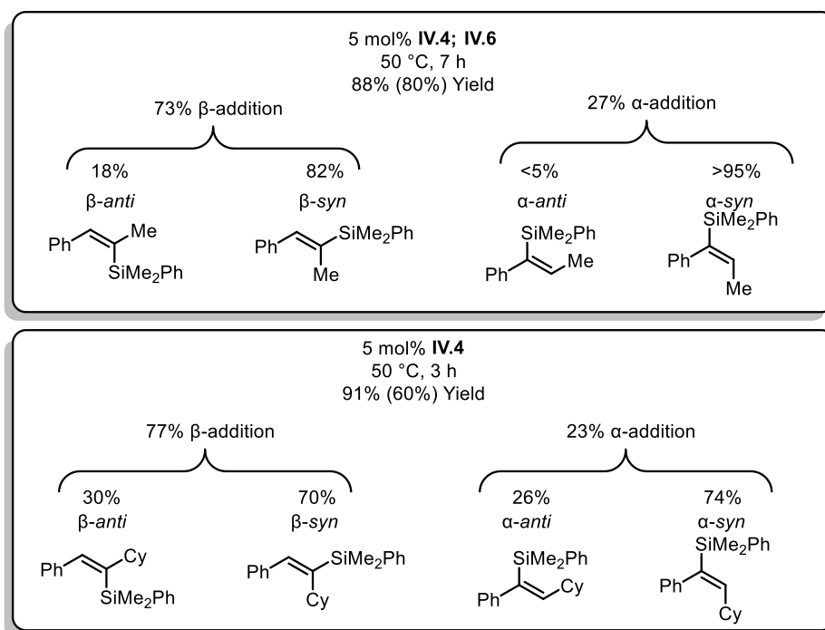
Figure IV.5: Hydrosilylation of dissymmetric internal alkynes with IV.4 or IV.6
