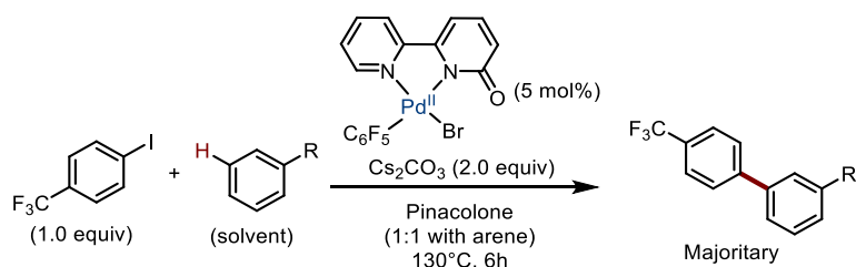
Scheme I.83: Solvent effects in the ligand assisted C-C cross coupling of arenes
