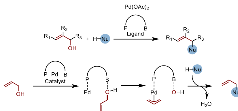
Scheme I.99: Proposed mode of activation of Boron-appended phosphine ligands in Kimura's templated reactions
