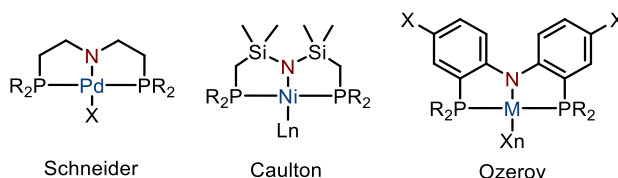
Figure I.12: Evolution of the PNP-scaffold from the initial design of Schneider to the dimethylsilyl-substituted version of Caulton and the diaryl version of Ozerov
