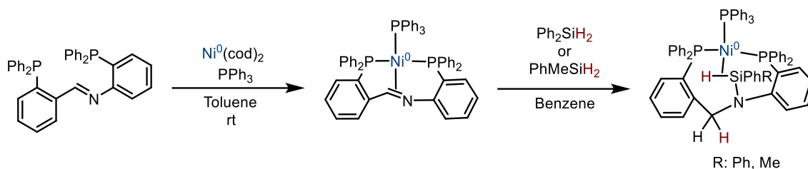
Scheme I.130: Synthesis of the Ni 0 complex and non-innocent character of the imine backbone
