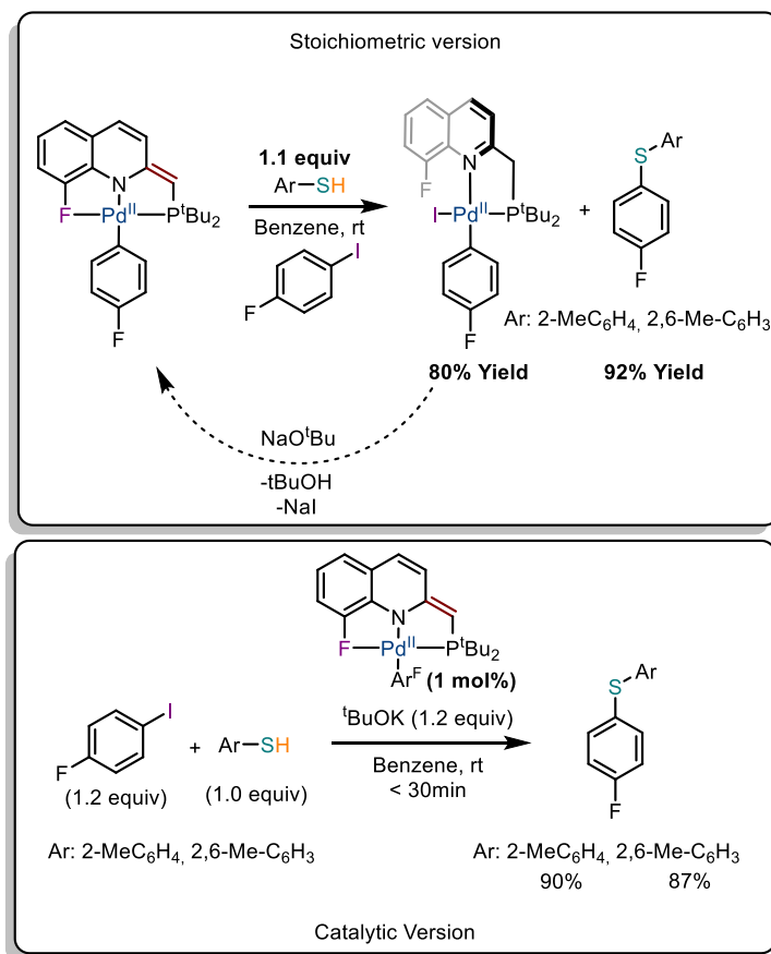
Scheme I.67: Catalytic activity towards S-C cross-coupling of Vigalok's PNF-Pd complex
