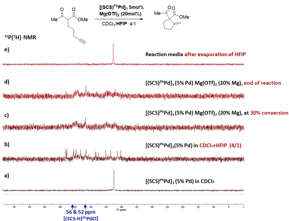
Figure II.10: NMR Monitoring of [(SCS)PhPd] 3 under catalytic reaction conditions
