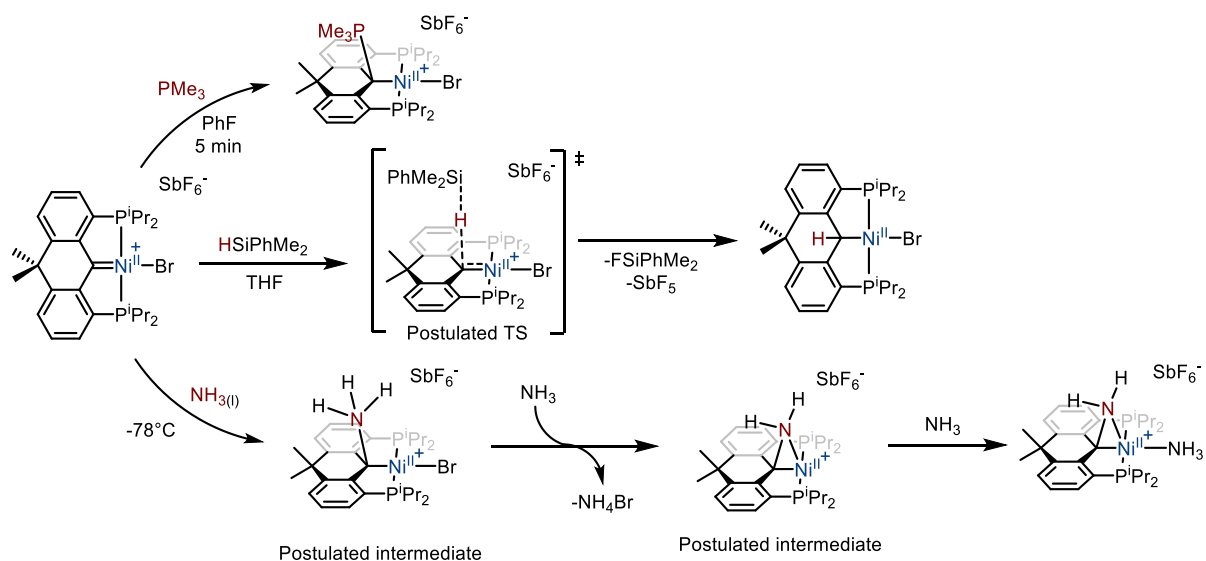
Scheme I.14: Electrophilic character of the 2e^- oxidized Ni-carbene complex developed by Piers
