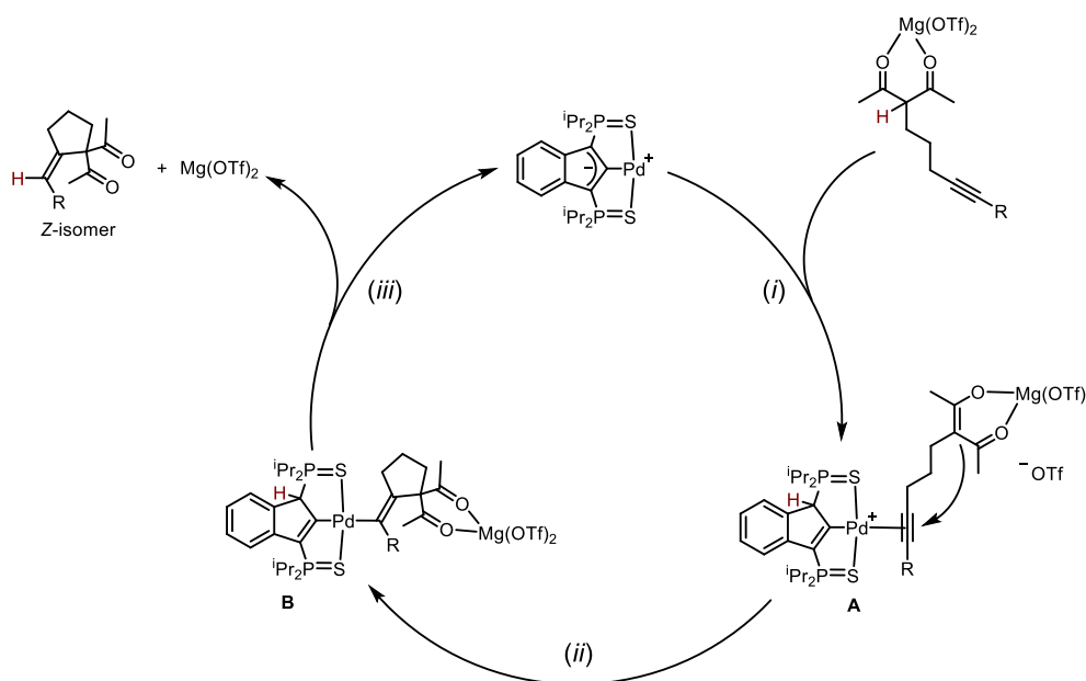
Scheme II.5: Catalytic cycle proposed to account for the Conia-ene reaction catalyzed by the (SCS)Pd complex and \text{Mg}(\text{OTf})_2
