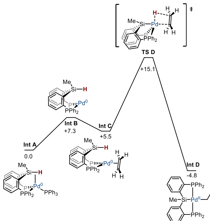
Scheme I.125: Proposed mechanism based on DFT calculations for the silyl-mediated insertion/ \beta -H elimination of ethylene. (Energies are in kcal.mol -1 )
