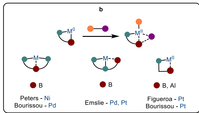
Figure I.23: Overview of the contributions in Lewis-acid assisted oxidative addition reactions
