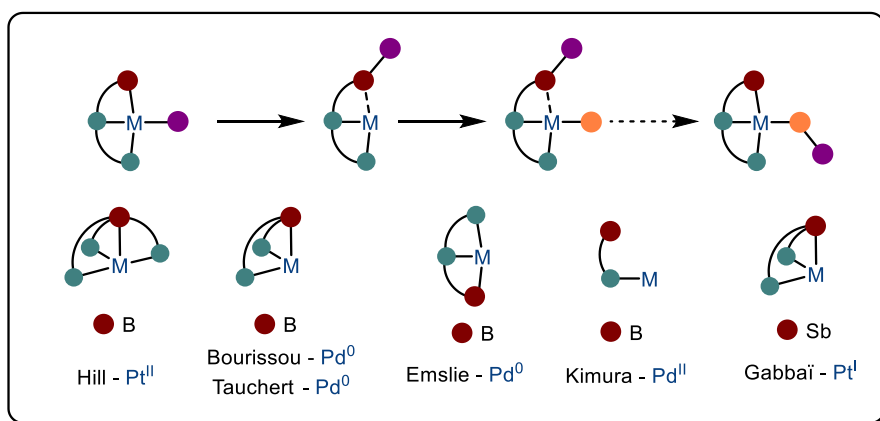
Figure I.22: Overview of the contributions where the Lewis acid acts as a temporary acceptor of functional groups
