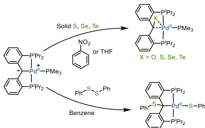
Scheme I.15: Oxidation of Iluc's Pd II -carbene to chalcogenoketones with nitrobenzene and group 16 elements, and oxidation with diphenyldisulfide
