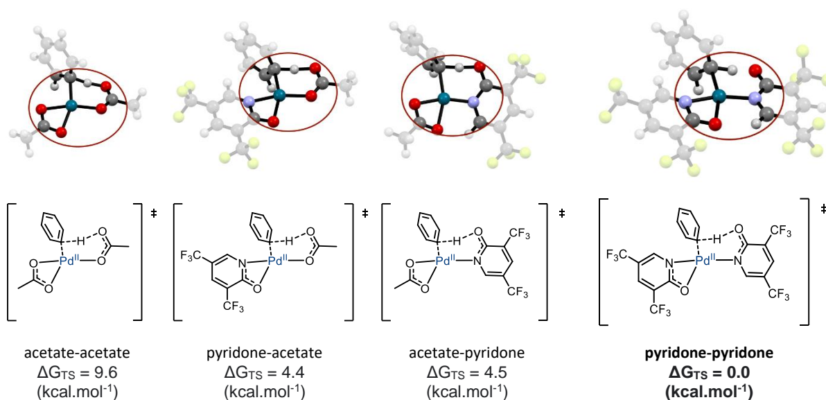
Figure I.18: Calculated DFT transition state and associated energy for the ligand assisted CMD
