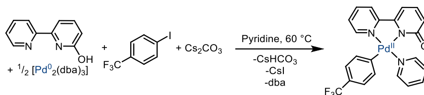
Scheme I.80: Synthesis of the pyridone-Pd complex by Albéniz
