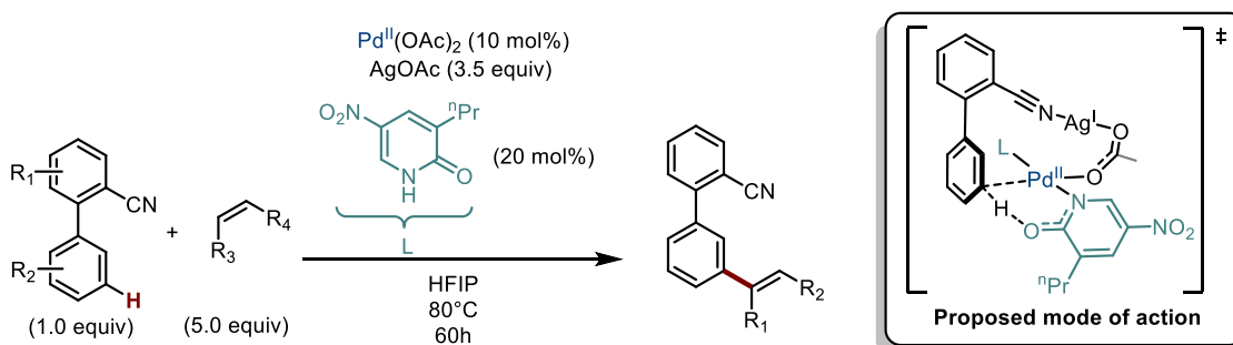
Scheme I.78: Remote meta-selective Heck-type coupling assisted by the transient formation of a non-innocent heterobimetallic complex
