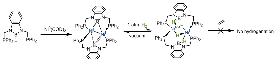
Scheme I.110: Boron assistance in reversible H 2 activation with DPBoryl-Ni complex
