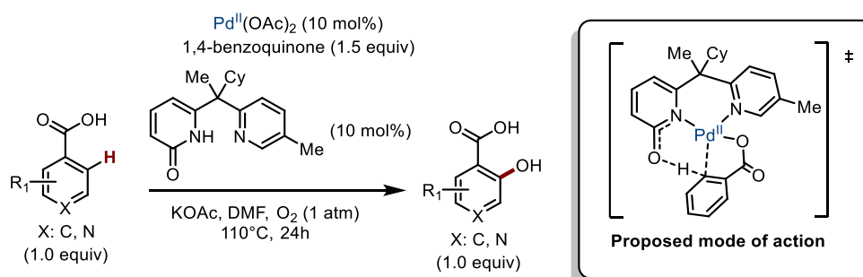
Scheme I.79: Hydroxylation of arenes with a non-innocent bidentate ligand assisting in the C-H activation step
