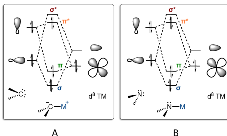
Figure I.13: A - Bonding situation in d 8 -dianion complexes; B - bonding situation in d 8 -amido complexes
