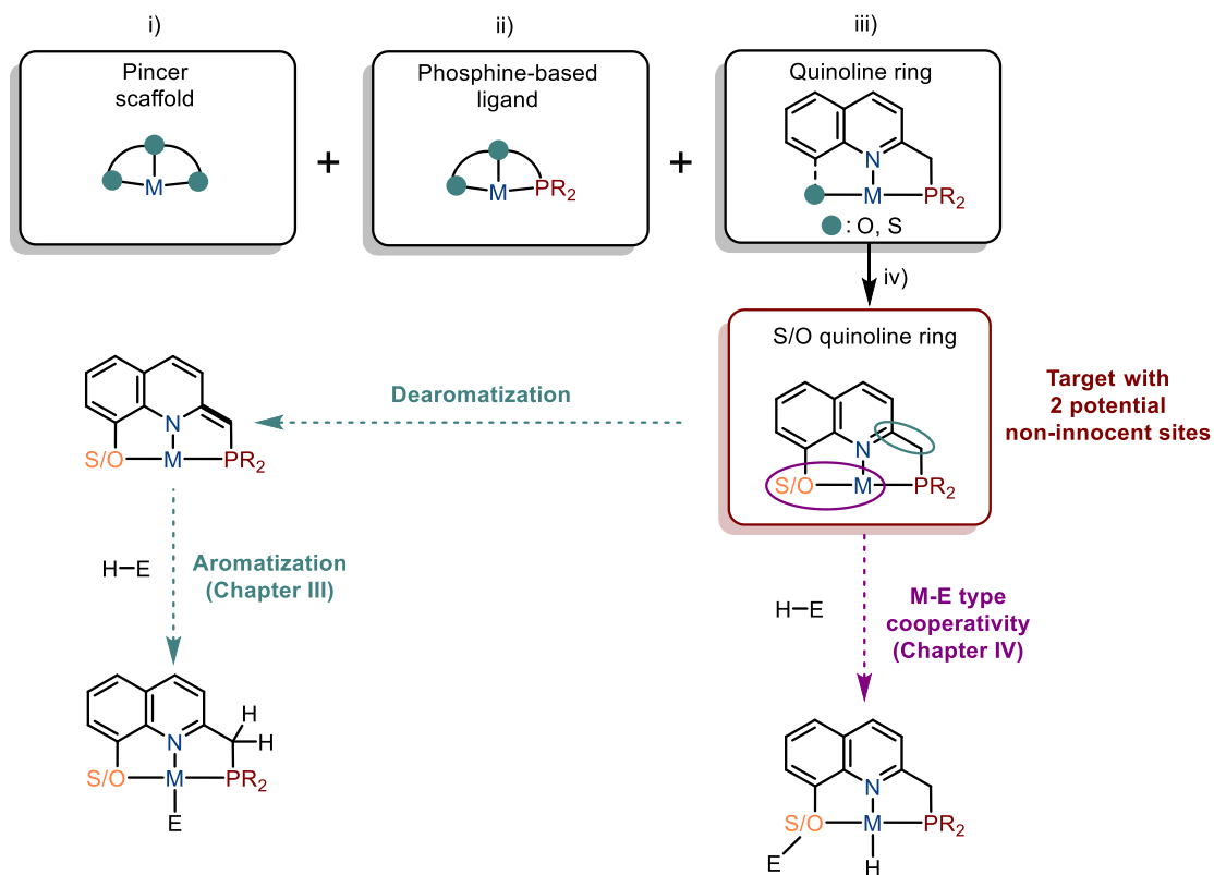
Scheme III.1: Criteria for the ligand design and potential modes of non-innocence
