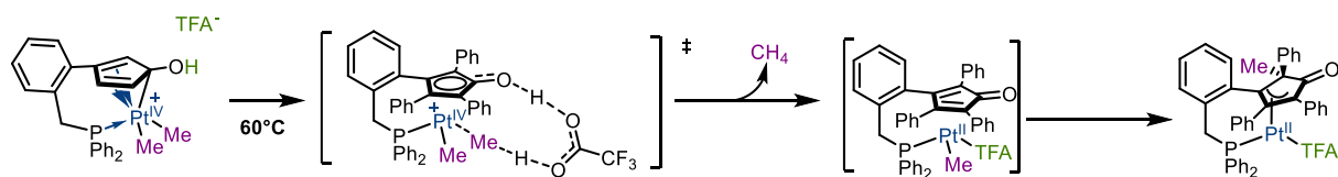
Scheme I.91: Proton-shuttling role of the conjugated base and further reaction of the Pt complex with TFA
