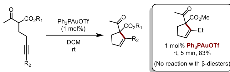
Scheme II.7: Gold catalyzed 5- endo Conia-ene cyclizations of internal alkynes reported by Toste
