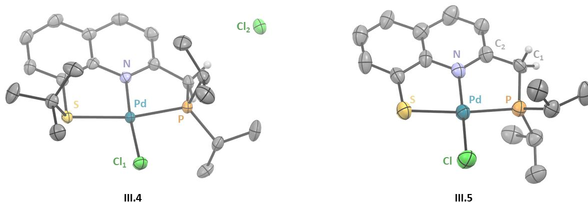
Figure III.2: XRD structure of the cationic PNS tBu -Pd-Cl complex III.4 and the neutral PNS-Pd-Cl III.5 with an outer-sphere chloride; H and DCM molecules were omitted for clarity
