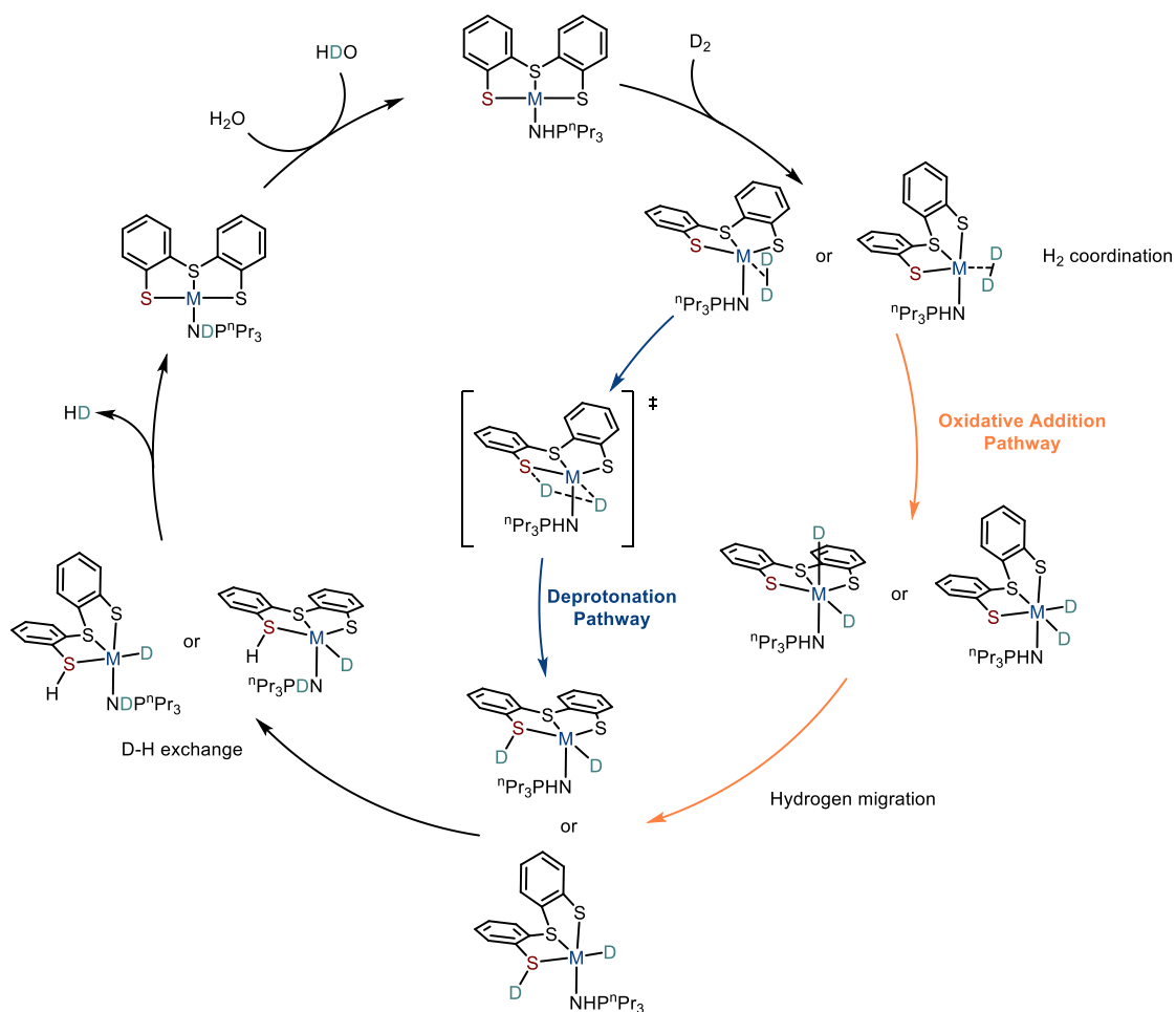
Scheme I.37: Calculated mechanism of H 2 activation by S 3 -Ni/Pd complexes – Orange oxidative addition pathway preferred for Ni II - Blue deprotonation and oxidative addition pathways were found reasonable for Pd II
