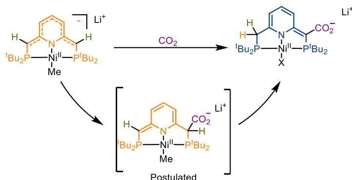
Scheme I.59: CO 2 fixation at the backbone of the anionic Ni II complex
