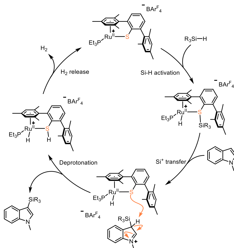
Scheme IV.4: Proposed mechanism for the dehydrogenative silylation of indoles by the cationic DmpS-Ru complex
