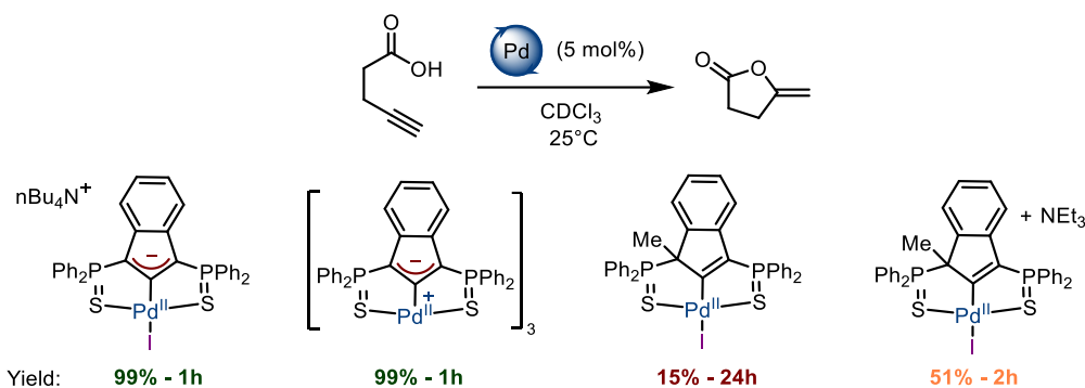
Scheme I.27: Comparison of the catalytic activities for the cycloisomerization of pentynoic acid
