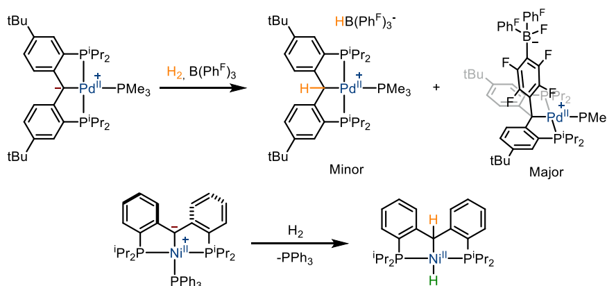
Scheme I.9: Top - \text{H}_2 activation by the association of Pd-carbene and BCF; Bottom - direct \text{H}_2 activation by the Ni-carbene complex
