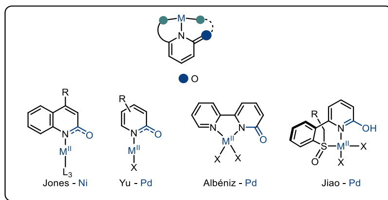
Figure I.17: Major contributions in the field of pyridone/hydroxypyridine cooperativity with group 10 metals
