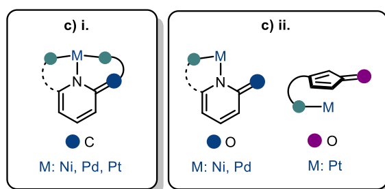
Figure I.14: Two-types of basic site in the aromatization/dearomatization approach
