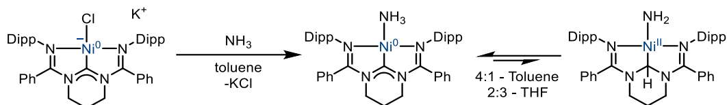
Scheme I.19: NHC-assisted N-H bond activation and solvent dependent equilibrium
