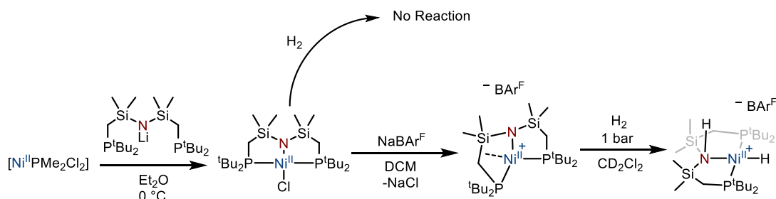
Scheme I.44: Synthesis of PNP- Ni^{II} complex and heterolytic H_2 splitting
