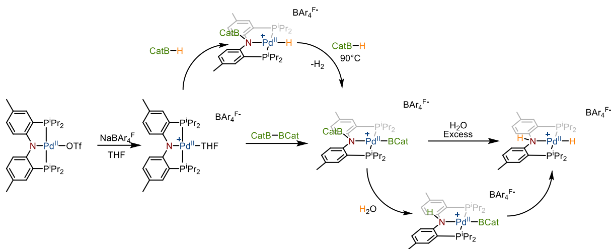
Scheme I.50: Pathway and navigation between the activation and hydrolysis products
