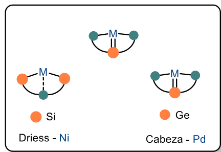
Figure I.8: Overview of the carbene analogs for MLC
