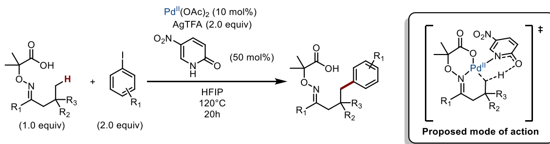
Scheme I.77: Cross-coupling between aryl iodides and \gamma\text{-C}_{\text{sp}^3}\text{-H} , with proposed involvement of MLC in the C-H activation step
