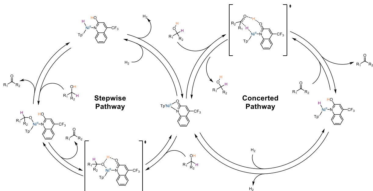
Scheme I.74: Two suggested mechanisms for the hydrogenation/dehydrogenation of alcohols
