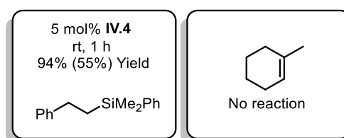
Figure IV.8: Hydrosilylation of alkenes with the cationic Pd complex IV.4
