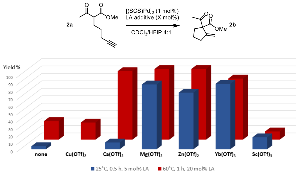
Figure II.2: Evaluation of the catalytic activity of the Pd complex [(\text{SCS})\text{Pd}]_2 in the presence of LA additives
