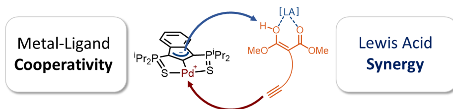
Scheme II.4: Combination of MLC and LA activation of \beta -dicarbonyl compounds
