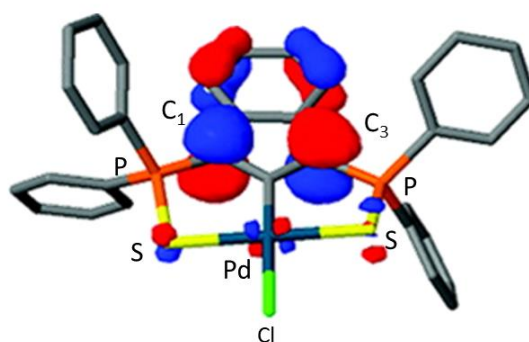
Scheme I.22: Representation of the HOMO showing the delocalized charge at the C1 and C3 positions
