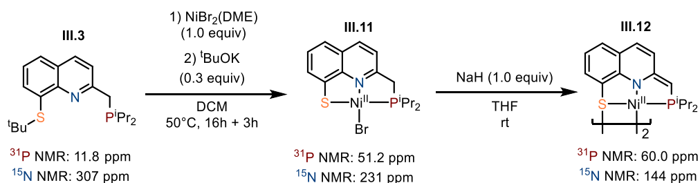
Scheme III.21: Synthesis of the PNS-Ni-Br complex III.11 and deprotonation to generate the dearomatized nickel dimer III.12
