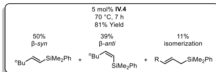
Figure IV.7: Hydrosilylation of hex-1-yne at 70 °C with IV.4
