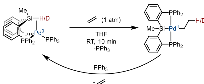
Scheme I.124: SiH-Pd 0 -PPh 3 as a masked form of Pd II -H for ethylene insertion
