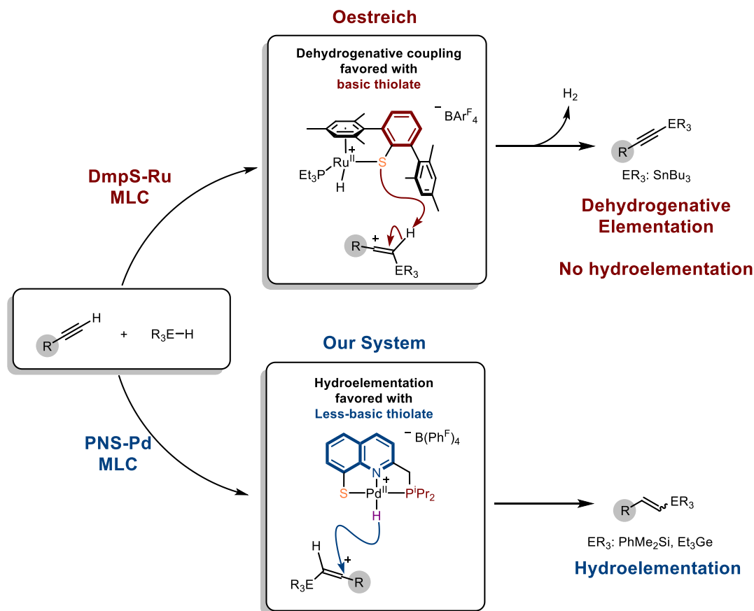
Scheme IV.27: Comparison of the DmpS-Ru system applied to the dehydrogenative stannylation of alkynes by Oestreich and our PNS-Pd system for the catalytic hydroelementation
