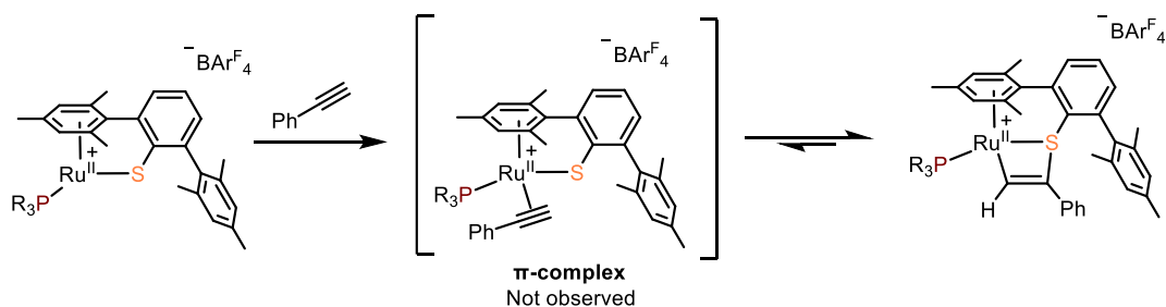
Scheme III.12: Ru-vinyl complex of Ohki upon reaction of phenylacetylene with the cationic Ruthenium-thiolate complex
