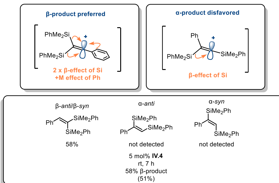
Figure IV.6: Hydrosilylation of the electronically biased internal alkyne Ph-CC-SiMe 2 Ph with IV.4
