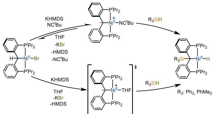
Scheme I.8: Silane activation by Piers' \text{Ni}^{\text{II}}\text{-THF}/\text{Ni}^{\text{II}}\text{-Nitrile} carbene complex
