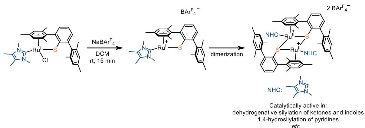
Scheme IV.7: Formation of binuclear Ru-S bridged dimer with an NHC ancillary ligand
