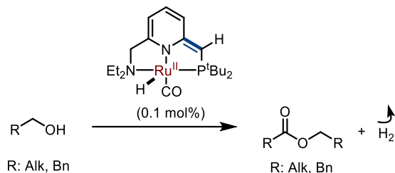
Scheme III.14: Dehydrogenation of alcohols into esters catalyzed by the non-innocent PNN complex of Milstein
