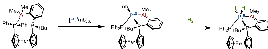
Scheme I.114: PPAI-Pt 0 complex and activation of H 2
