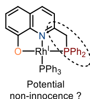
Figure III.1: PNO-Rh I complex of Kakiuchi and potential site for chemical non-innocence
