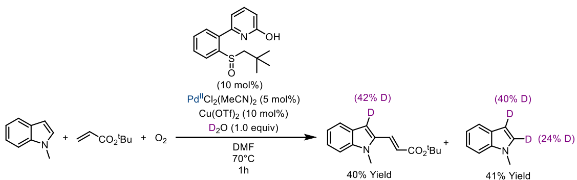
Scheme I.87: D-labeling experiments with D 2 O showing D incorporation at the C 2 and C 3 position: Reaction was performed in presence of D 2 O and stopped at half conversion
