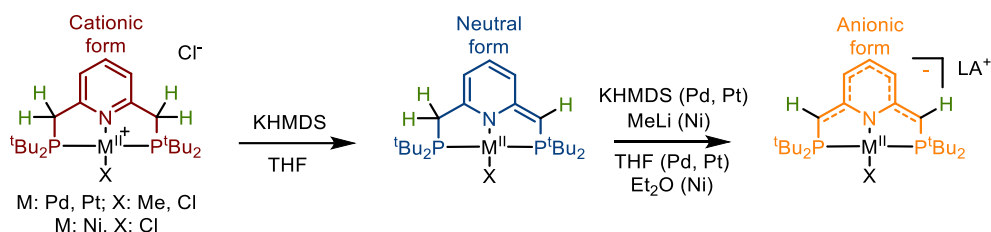
Scheme I.57: Group-10 pincer complexes reported by Milstein in their cationic, neutral, and anionic forms
