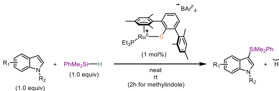
Scheme IV.3: Dehydrogenative silylation of indoles by the cationic \text{DmpS-Ru}^{\text{II}} complex
