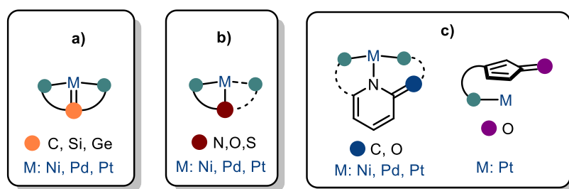
Figure I.2: Overview of the complexes and ligand designs exhibiting cooperativity between a basic-site and a group 10 transition metal.
