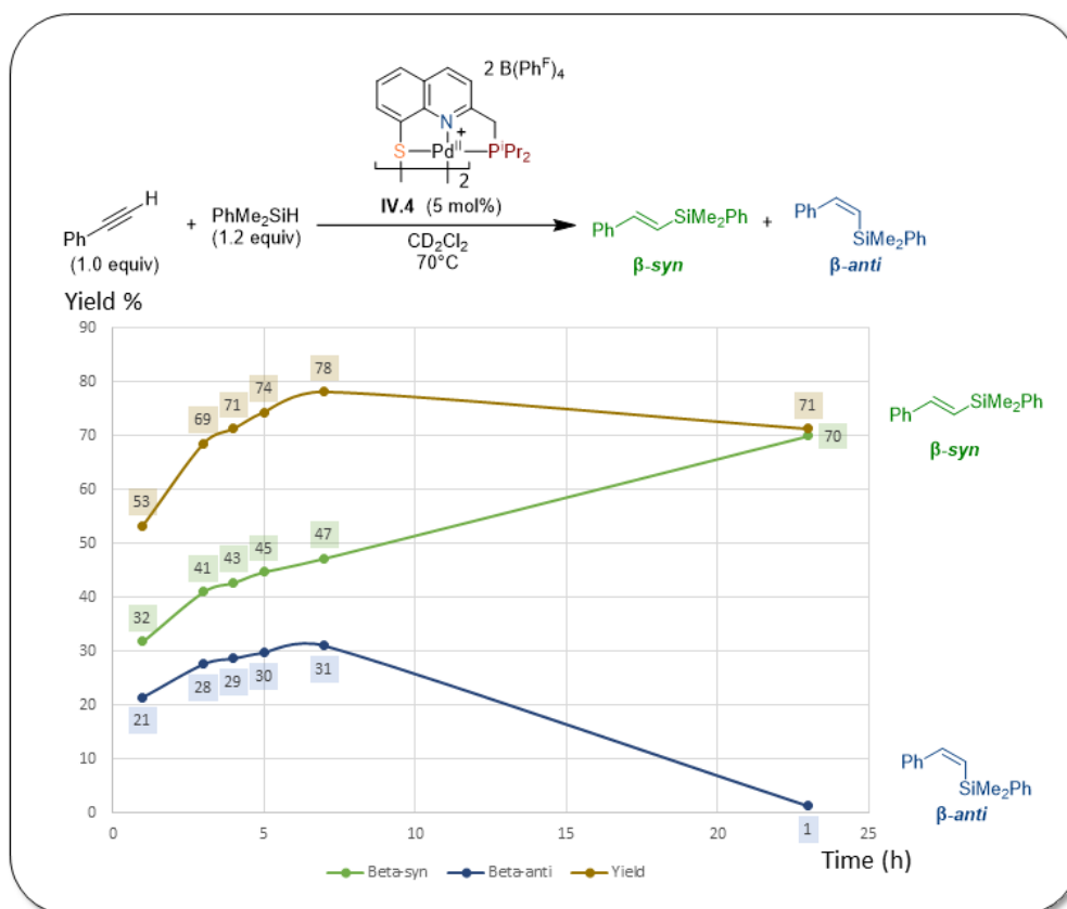
Scheme IV.23: Monitoring over time of the hydrosilylation of phenylacetylene using IV.4
