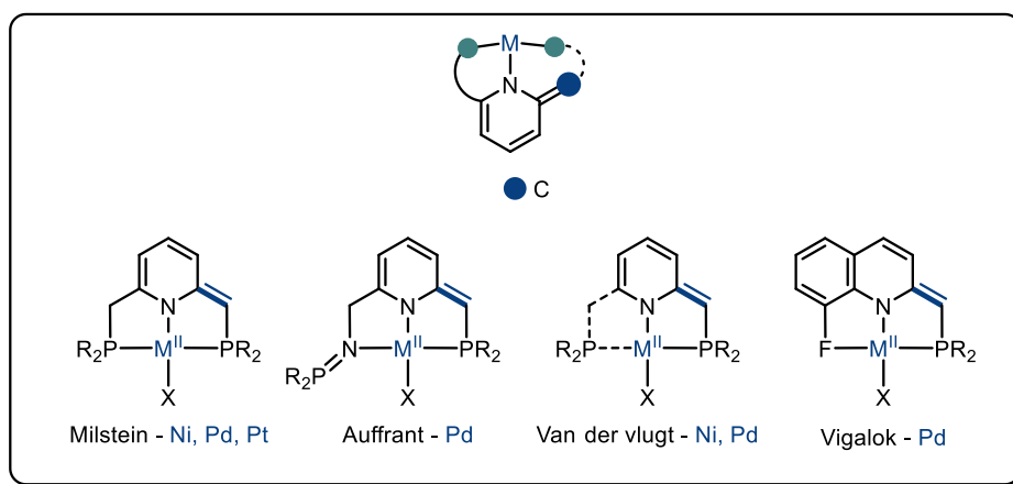
Figure I.15: Main contributions in the aromatization/dearomatization approach with group 10 metal complexes
