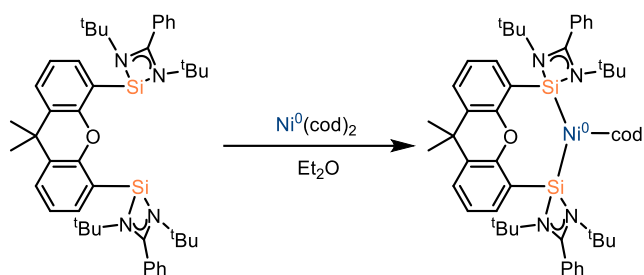
Scheme I.31: Synthesis of the Bis-silylene Ni 0 complex of Driess
