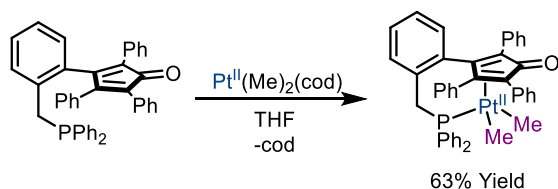
Scheme I.89: Synthesis of the \pi -arene Pt II complex of Nozaki
