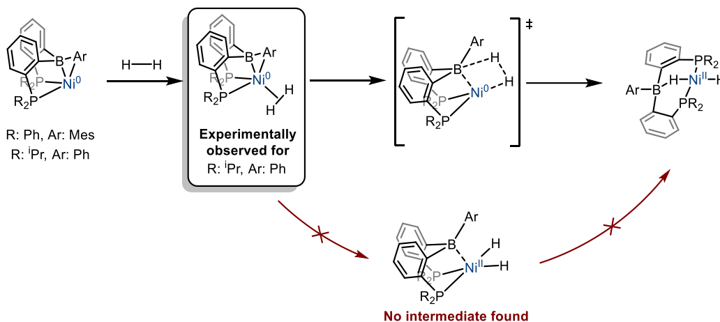
Scheme I.105: Mechanism of boron-assisted H 2 activation in DPB-Ni 0 complexes
