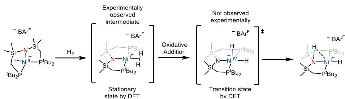
Scheme I.45: Mechanistic pathway for H_2 activation through \sigma -bonded H_2 intermediate
