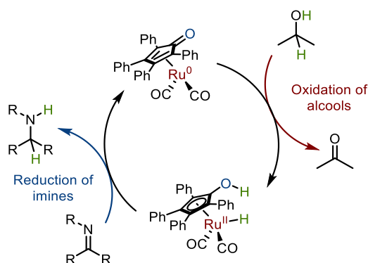
Scheme III.13: Simplified mechanism of the tandem oxidation of alcohol and reduction of imine using Shvo's catalyst
