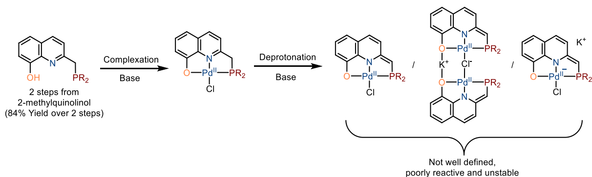
Scheme III.2: Synthesis of a PNO-Pd II complex and initial results towards the generation of dearomatized species
