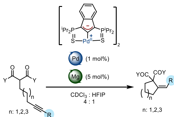
Scheme I.30: Multi-cooperative catalytic system for Conia-ene type cycloisomerization
