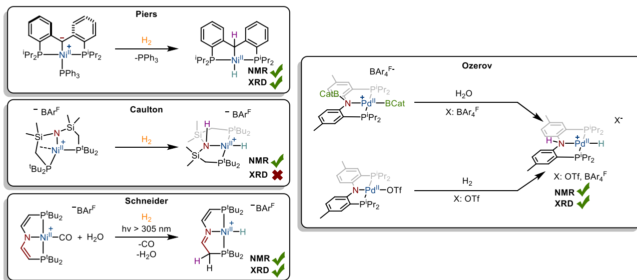
Figure III.10: Examples from the literature of pincer group 10 metal hydrides bearing an acidic proton at the ligand backbone
