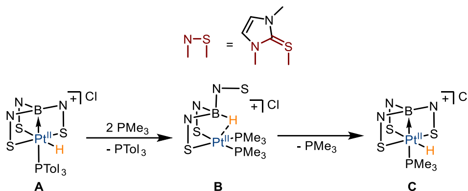
Scheme I.95: Boron as temporary acceptor of hydride for phosphine substitution at metallaboratrane
