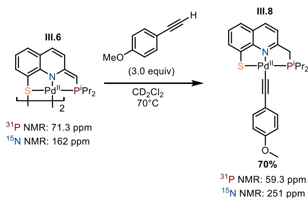
Scheme III.10: C-H activation of alkynes by the dearomatized \text{Pd}^{\text{II}} dimeric complex III.6
