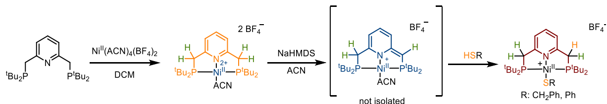
Scheme I.63: S-H bond activation by the dearomatized Ni complex of Van der Vlugt
