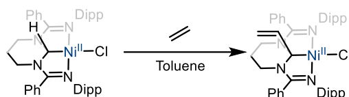
Scheme I.20: Ethylene insertion at the NHC moiety of an NCN-Ni II pincer complex
