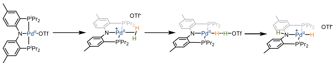
Scheme I.48: Mechanism of heterolytic H 2 activation with proton transfer assisted by an exogenous base
