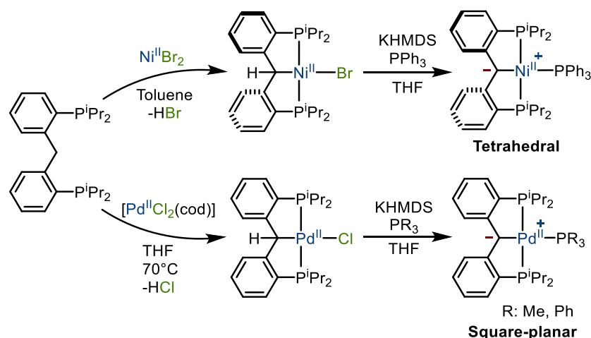
Scheme I.5: Synthesis of PCP Pincer carbene Pd II and Ni II complexes by C-H activation and subsequent deprotonation
