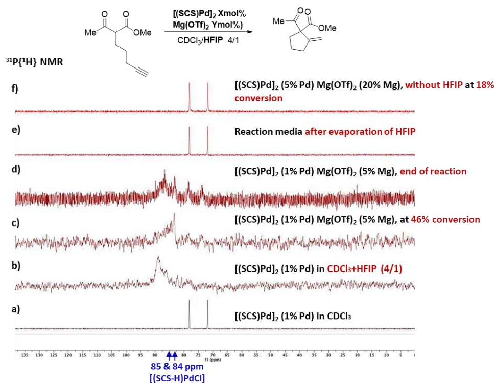
Figure II.9: NMR Monitoring of [(SCS)Pd] 2 under catalytic reaction conditions
