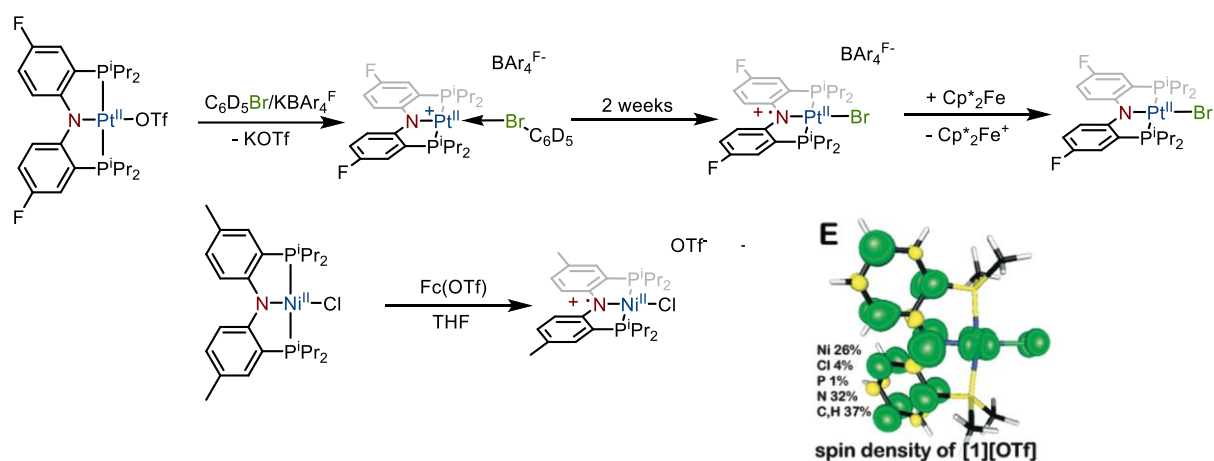
Scheme I.52: Halogen abstraction and radical formation by Ozerov and Mindiola – Spin density of Ni II -Cl complex adapted with permission from J. AM. CHEM. SOC. 2008, 130, 3676-3682. Copyright 2008 American Chemical Society.
