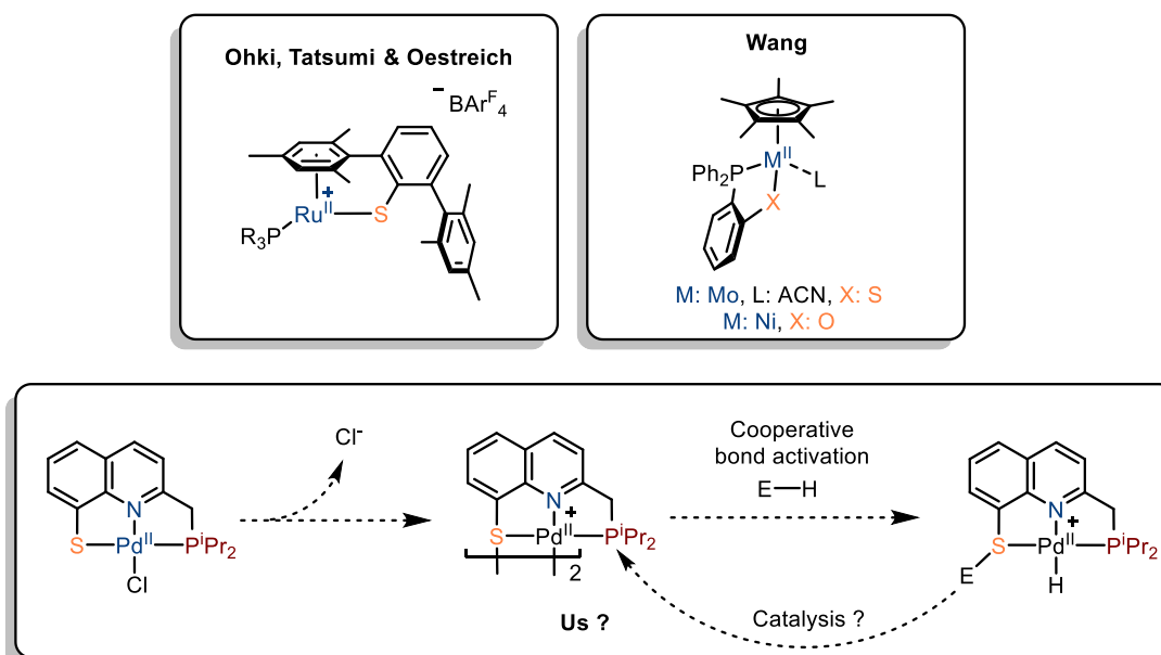
Scheme IV.12: Overview of the presented systems and ligand designs exhibiting M-X cooperativity and potential applications of our quinoline PNS ligand design for Pd-S cooperativity
