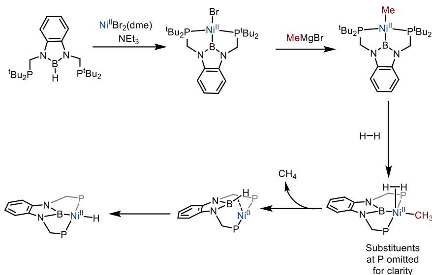
Scheme I.111: Boryl-assisted hydrogenolysis of C(sp 3 ) bond and formation of a Ni II -H complex
