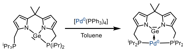
Scheme I.34: T-shaped Pd 0 complex synthesis by Cabeza
