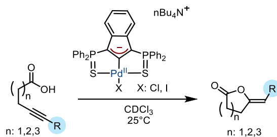
Scheme I.24: Cycloisomerization of alkynoic acids with the non-innocent SCS-Pd II complex
