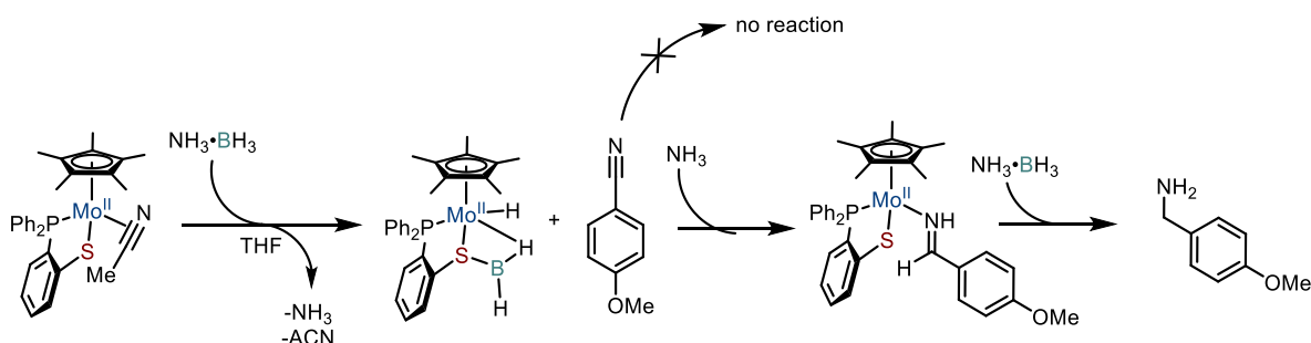
Scheme IV.10: Stoichiometric reaction of the Mo II complex with amine borane and subsequent partial hydrogenation of paramethoxybenzoxonitrile
