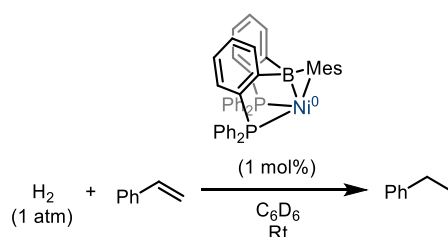
Scheme I.106: Catalytic hydrogenation of styrene by the DPB-Ni 0 complex of Peters
