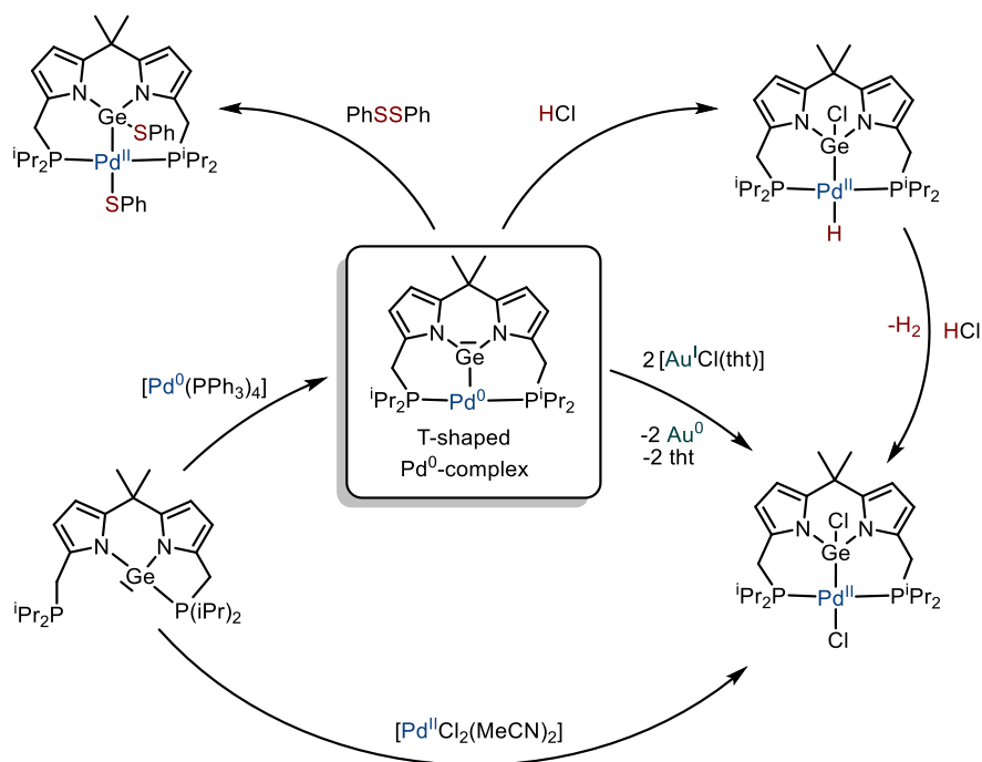
Scheme I.35: Synthesis of Germylene-Pd 0 complex by Cabeza and reactivity
