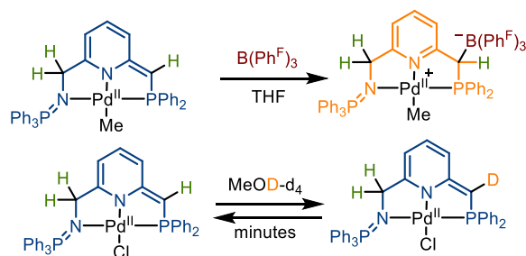
Scheme I.62: Nucleophilic character and reversible O-D bond activation by the dearomatized PNN-Pd complex
