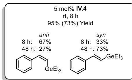
Figure IV.11: Hydrogermylation of phenylacetylene with IV.4
