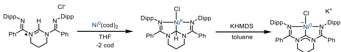
Scheme I.18: Synthesis of an anionic Ni 0 -NHC complex by deprotonation and reduction of the CH-Ni II -Cl
