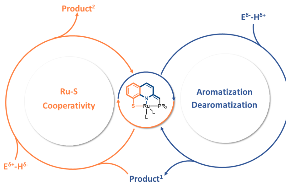
Figure 16: General representation of a tandem/one-pot approach involving the two modes of cooperativity
