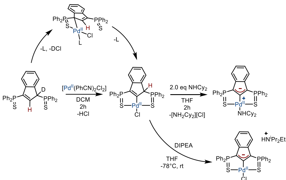
Scheme I.21: Synthesis and coordination mechanism of the SCS-Pd II complex
