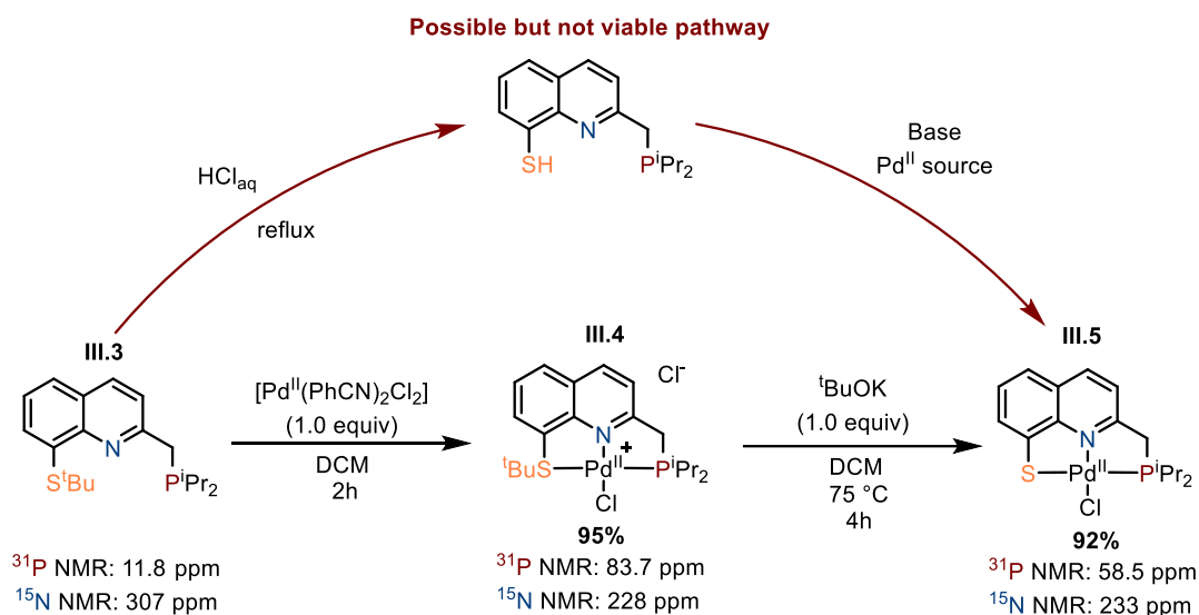
Scheme III.5: Initial synthetic pathway with acidic ^t\text{BuS} deprotection and Pd-assisted synthesis of the \text{PNS-Pd}^{\text{II}}\text{-Cl} complex
