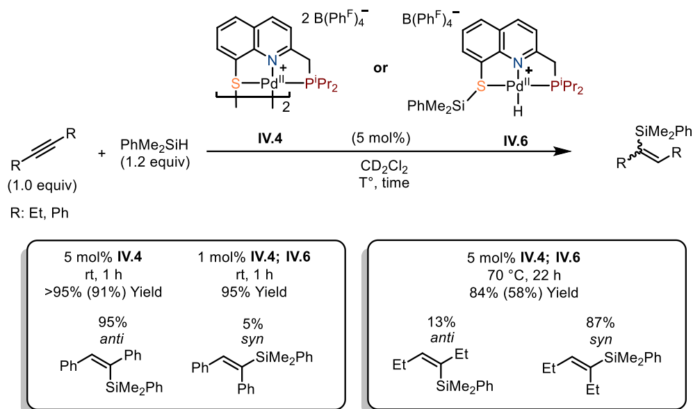
Scheme IV.17: Catalytic hydrosilylation of symmetric internal alkynes using IV.4 or IV.6 ; Isolated yields are given in brackets.
