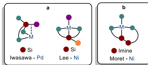
Figure I.25: Overview of the other examples of MLC with group 10 metals
