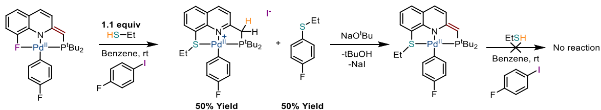
Scheme I.66: Substitution and reductive elimination with alkyl-substituted thiols
