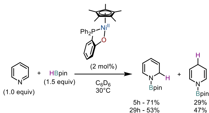
Scheme I.39: Catalytic hydroboration of pyridines with the non-innocent Ni-O complex
