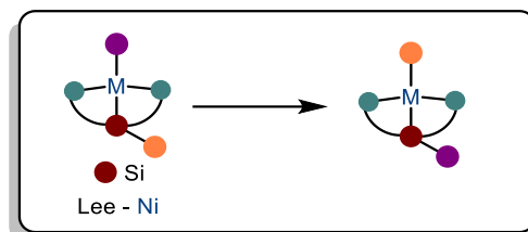
Scheme I.126: Schematic view of the silicon-mediated group exchange at the transition metal by the Ni-complex of Lee
