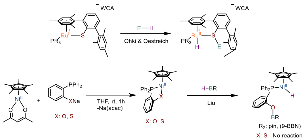
Scheme I.38: Ohki Ru-S complex and Liu's approach with Ni II
