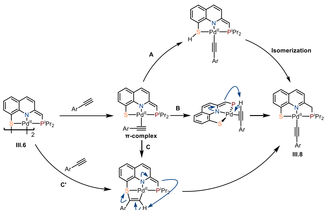
Scheme III.11: Proposed mechanisms for the C-H activation of alkynes by the dearomatized Pd complex III.6
