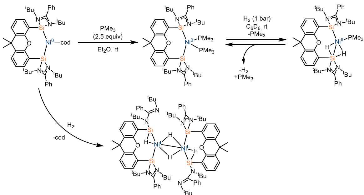
Scheme I.32: Reactivity of Silylene-Ni 0 complexes with H 2 and chemical non-innocence of the silylene fragment
