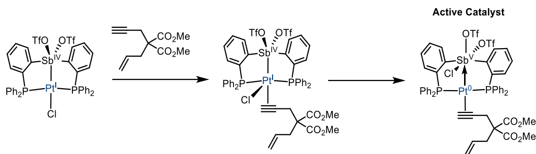
Scheme I.102: Proposed pathway for the self-activation of Figeroa's Pt I complex
