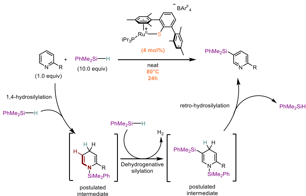
Scheme IV.6: meta -selective dehydrogenative silylation of pyridines reported by Oestreich using the cationic DmpS-Ru II complex
