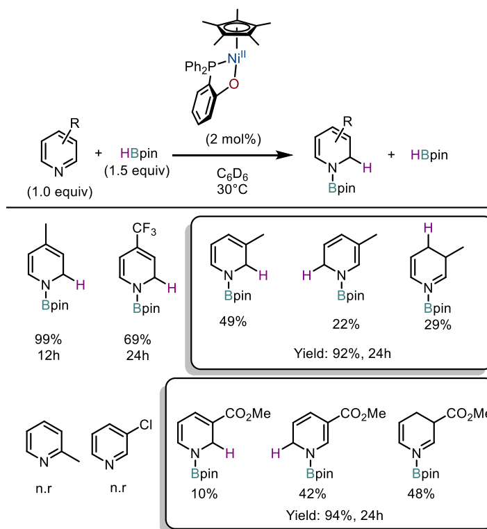
Scheme I.40: Catalytic hydroboration reaction catalyzed by Liu's Ni II complex
