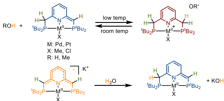
Scheme I.58: E-H bond activation and hydrolysis of PNP-M complexes
