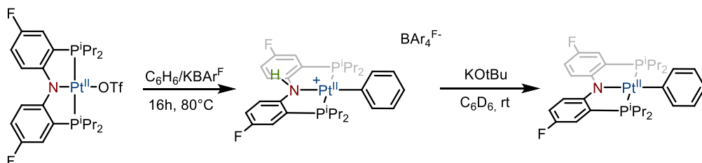
Scheme I.51: C-H activation by MLC trough Pt-N bond by the cationic Pt complex
