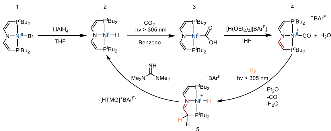
Scheme I.54: Reversed water gas shift reaction with MLC by Schneider
