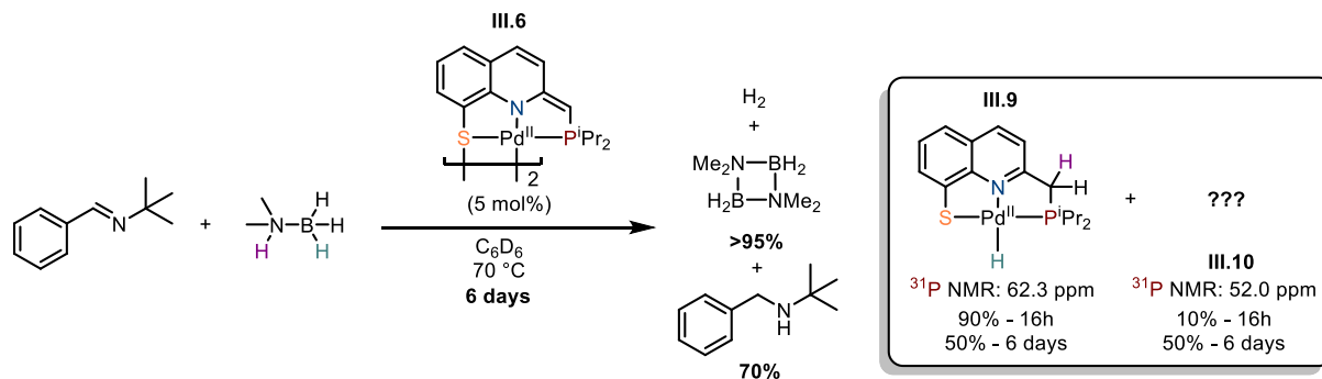
Scheme III.17: Catalytic dehydrogenation of DMAB by the dearomatized complex III.6 in presence of a H 2 acceptor
