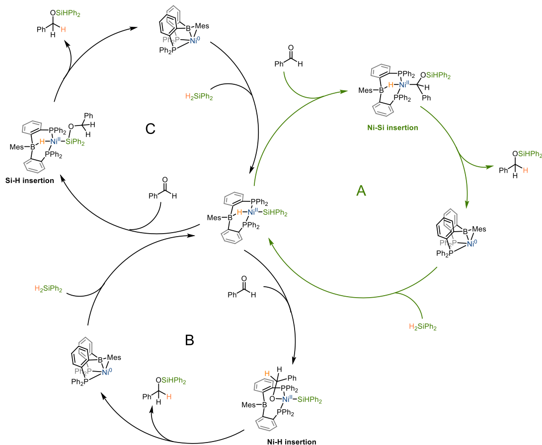
Scheme I.108: Postulated mechanisms of carbonyl hydrosilylation by the DPB-Ni 0 complex of Peters
