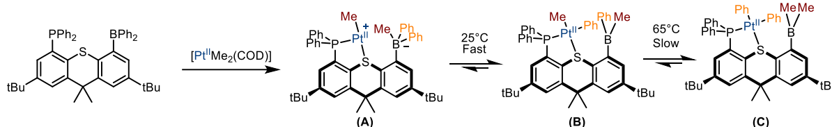
Scheme I.93: Group exchange between \text{Pt}^{\text{II}} and boron in the TXPB- \text{Pt}^{\text{II}} complex of Emslie
