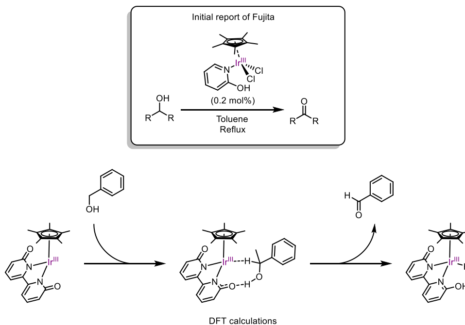
Scheme I.70: Initial report of Fujita with the cooperative dehydrogenation of alcohols.
