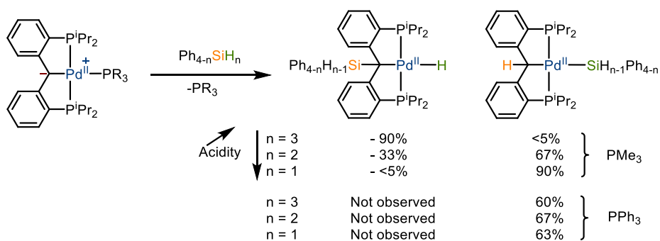
Scheme I.7: Product distribution for Si-H activation depending on the substituents at Si and P
