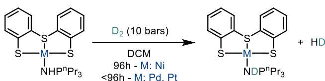
Scheme I.36: D 2 activation by M-S cooperativity
