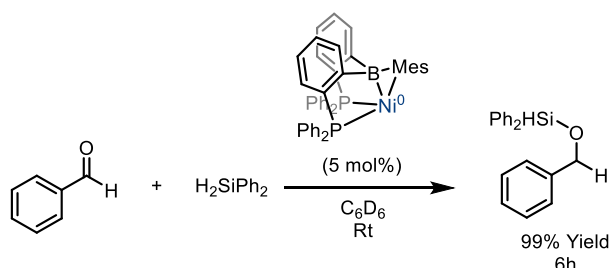
Scheme I.107: Catalytic hydrosilylation of carbonyls by the DPB-Ni 0 complex of Peters
