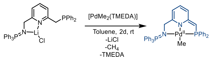
Scheme I.61: in situ generation of the dearomatized PNN-Pd complex of Auffrant
