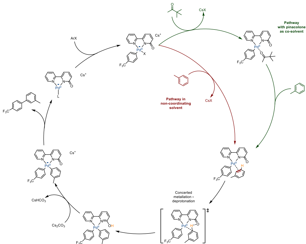
Scheme I.84: Catalytic cycle of the C-C cross-coupling reaction developed by Albéniz with and without pinacolone as co-solvent
