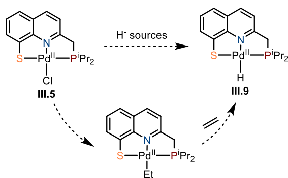
Scheme III.19: Planned synthesis of the Pd-H III.9 with hydride sources
