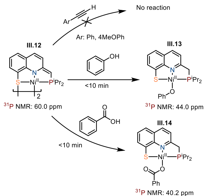
Scheme III.22: C-H activation with the dearomatized Nickel complex III.12
