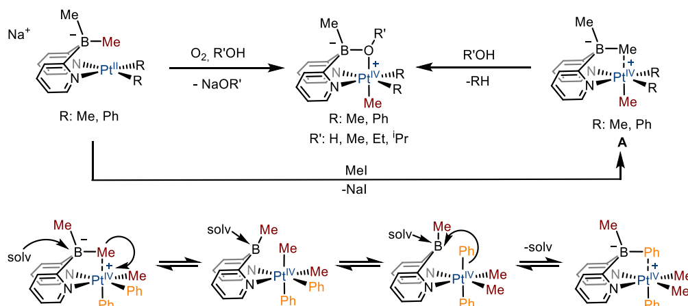
Scheme I.92: First example of group exchange mediated by boron reported by Vedernikov
