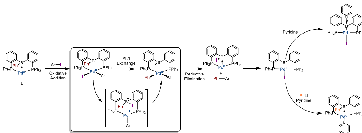
Scheme I.94: Boron-mediated halide abstraction and group transfer in \text{DPB-Pd}^{\text{II}} complex as reported by Tauchert
