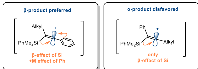
Scheme IV.22: Stabilization in the case of a dissymmetric aryl-alkyl internal alkyne and proposed explanation for the \beta -preference.
