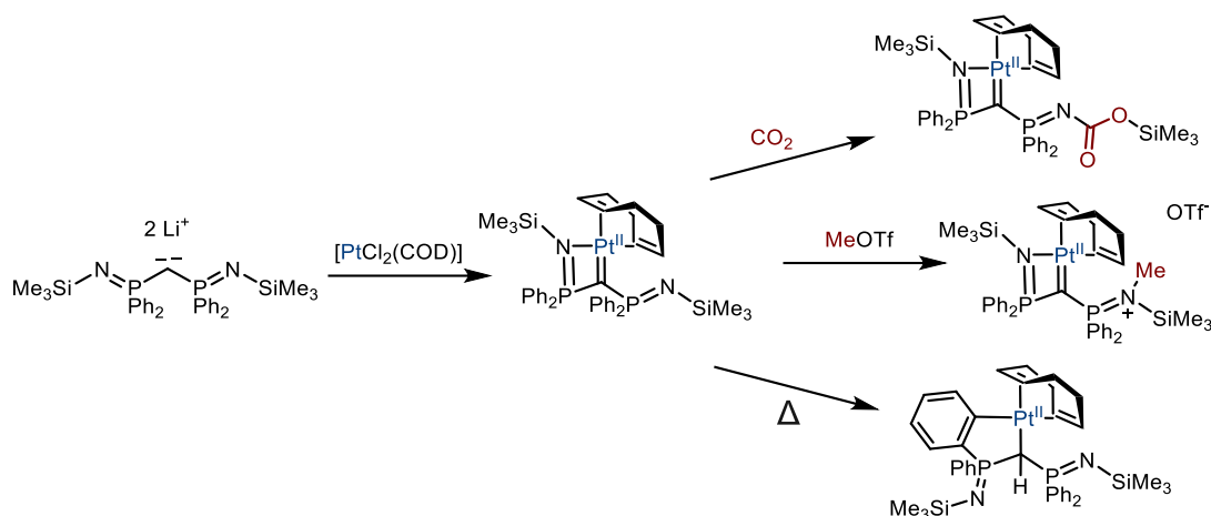
Scheme I.1: Synthesis and reactivity of Cavell's \text{Pt}^{\text{II}} carbene complex
