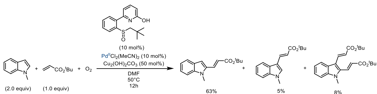
Scheme I.86: Catalytic activity and synthesis of Jiao's complex for the catalytic alkenylation of indoles
