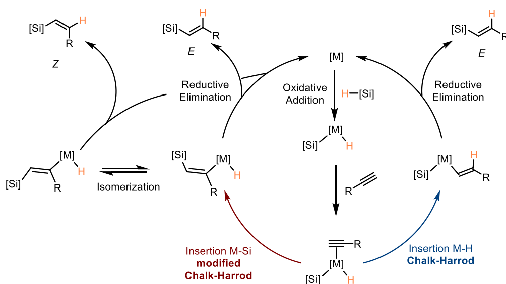
Scheme IV.18: Catalytic cycles of TM catalyzed hydrosilylation: Chalk-Harrod and modified Chalk-Harrod mechanisms.
