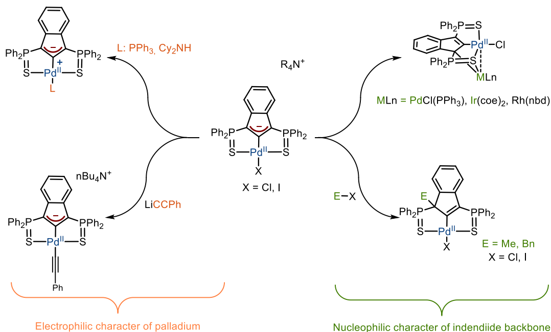
Scheme I.23: Evidencing the bifunctional character of the Indenediide-Pd complex
