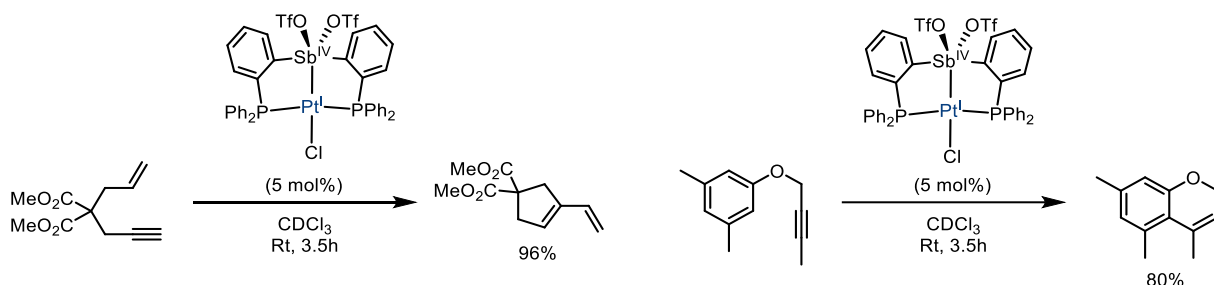
Scheme I.101: Catalytic activity of PSbP-Pt complex in enyne cyclization and intramolecular hydroarylation reactions
