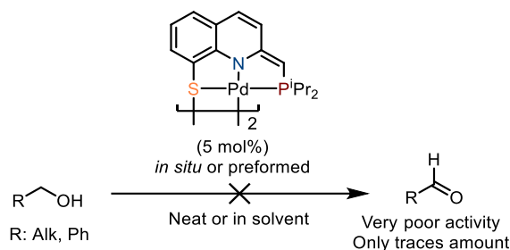
Scheme III.15: Absence of reactivity in the catalytic dehydrogenation of alcohols the dearomatized dimeric complex.
