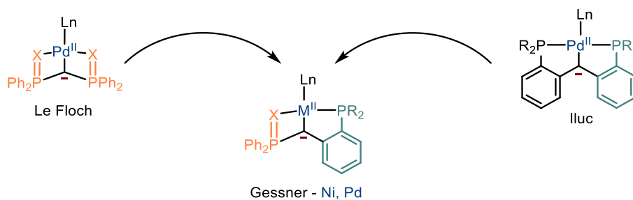
Figure I.7: Gessner's approach merging Le Floch and Iluc's ligand design
