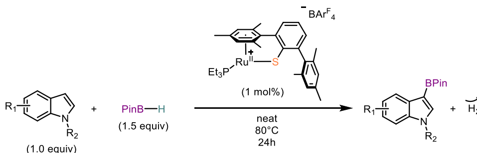
Scheme IV.8: General reaction scheme of the catalytic dehydrogenative borylation reported by Ohki and Oestreich with the cationic DmpS-Ru II complex
