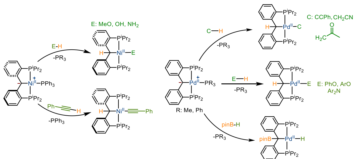
Scheme I.6: Reactivity of Piers' and Iluc's carbene complexes towards E-H bonds
