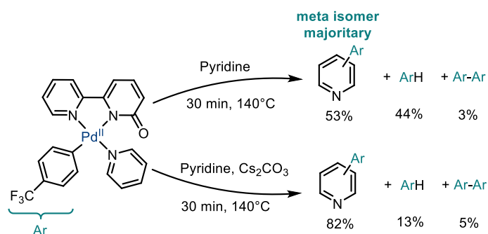
Scheme I.81: C-H activation and reductive elimination of pyridone-Pd complex
