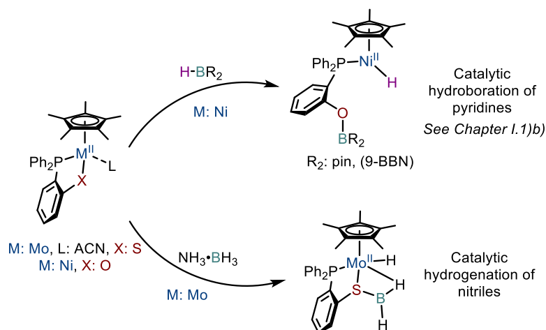
Scheme IV.9: Piano-stool complexes of Wang for cooperative M-X bond activation and catalytic reactions
