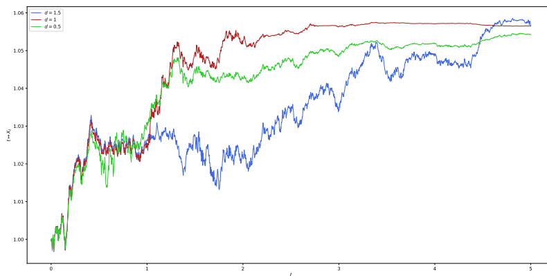
Figure 6.8 t \mapsto X_t^* , with \sigma_1 = \sigma_2 = 1 , \lambda_1 = \lambda_2 = 0.5 , T = 5 and \rho = -0.7 for d = 1.5 , 1 and 0.5. The same realizations of the Brownian motions W^1 and B was used for all experiments.
