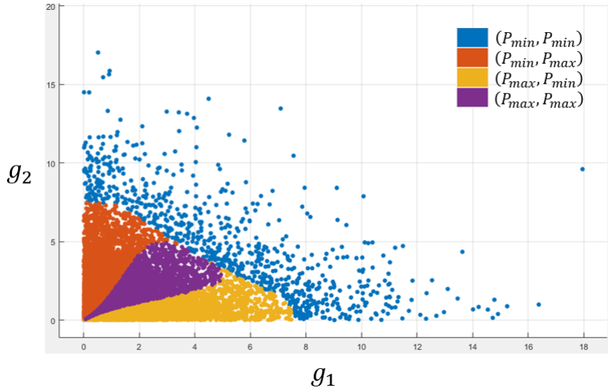
FIGURE 3.7 – Quantization regions of goal-oriented quantizer for 2-band energy efficiency problem. When one channel is dominant, it is better to transmit with higher power levels in that dominant channel. Otherwise, both transmitters choose the same transmit power.
