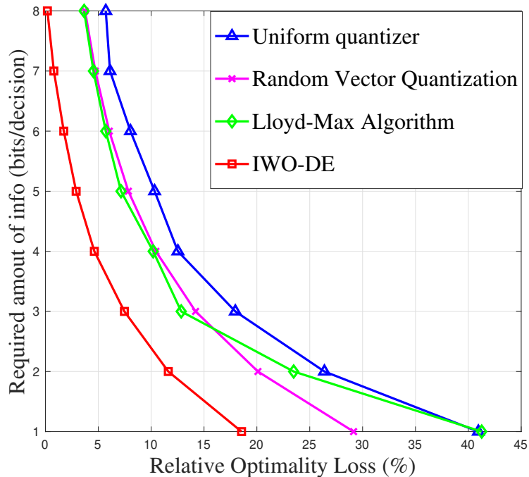
FIGURE 3.9 – Required bits of quantization v.s. relative optimality loss for Case II (packet success transmission rate as benefit of energy efficiency) with B_1 = 4 bits/decision. The benefits from using our algorithm is very apparent on this figure. For example, for an optimality loss of 5% between the perfect CSI case and the finite-rate feedback case, the amount of information needed to perform beamforming can be reduced by around 2 by moving from the best state-of-the-art approach to the proposed approach.
