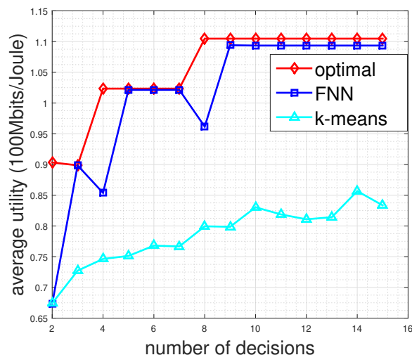
FIGURE 3.5 – Average utility v.s. number of decisions for N_t = 4 and N_r = 1 (MISO). Here \sigma^2 = 5\text{mW} , P_0 = 10\text{mW} and P_{\max} = 12\text{mW} . FNN is better than k -means quantizer and close to theoretical optimum.
