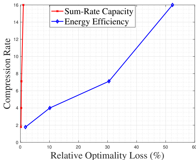
FIGURE 3.8 – The compression rate as a function of the relative optimality loss (%) for single user 2-band scenario for energy efficiency and sum-rate capacity. Compressing the channel gain for sum-rate capacity function is easier than compressing the channel gain for energy-efficiency function.
