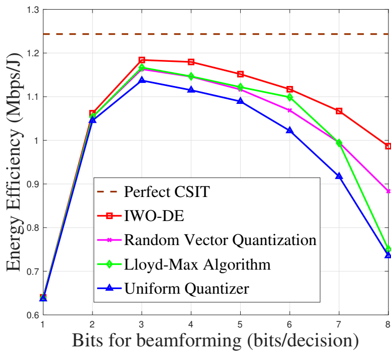
FIGURE 3.12 – Energy efficiency v.s. bits of quantization for beamforming ( B_2 ) for case II (packet success transmission rate as benefit function of EE). The conventional approach is sensitive to the available amount of feedback information for beamforming when power level quantization is rough while the proposed approach offers good performance for a large range of feedback rates.
