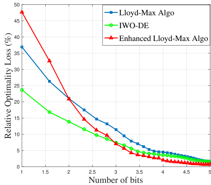
FIGURE 4.2 – Relative optimality loss as a function of number of bits of quantization for LM algorithm, IWO-DE algorithm, enhanced Lloyd-Max algorithm( using value density instead of the original p.d.f.) for EE (bit error rate) cost function
