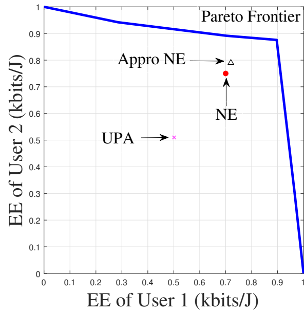
FIGURE 6.4 – Performance achieved by alg. 7 (NE) and alg. 8 and UPA with N_t = 2 and N_r = 4 for 2-user situation. Policy found by alg. 8 is very near to the exact NE and Pareto-dominates it. Moreover, two policies found by proposed algorithms both outperform UPA.
