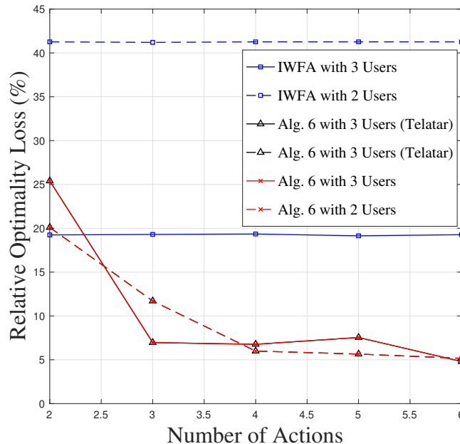
FIGURE 5.2 – Relative optimality loss (%) of average social welfare as a function of number of actions for iterative water-filling algorithm(IWFA), alg. 6 with Telatar set as the underlying action space, and alg. 6 for 2-user and 3-user scenarios with P_{\max} = 1\text{mW} and \sigma^2 = 1\text{mW} and number of bands S = 3 . Braess’s Paradox exists in almost all configurations except for M = 2 decisions. Optimal action set maximizing the average social welfare with given cardinality is always the Telatar-type set. Our conjecture is verified for number of actions in 2 \leq M \leq 6 .
