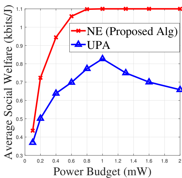
FIGURE 6.3 – Performance under NE and UPA as function of the power budget of user with N_t = N_r = 2 for 2-user situation. There are two different regions : one corresponds to Prop. 6.3.5. In the region uncovered by Prop. 6.3.5, alg. 8 still dominates UPA.
