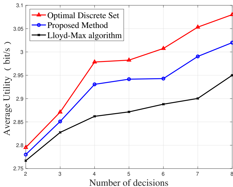
FIGURE 3.2 – Average utility (sum-rate capacity) v.s. number of decisions for Lloyd-Max Algorithm, enhanced improve and branch algorithm and optimal discrete set with given number of decisions. There are 6 bands, maximum power is P_{\max} = 4\text{mW} and variance of noise \sigma^2 = 1\text{mW} . Without Knowledge about optimal decision function, proposed approach still yields acceptable performance compared to Lloyd-Max quantizer which entails the knowledge of regularity property assists the design of goal-oriented quantizer.
