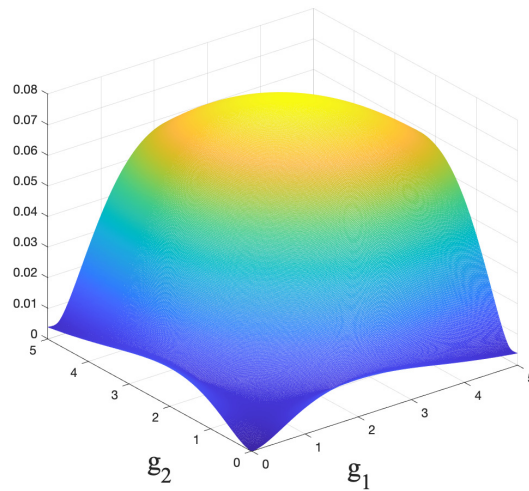
(b) New density weighted by maximum eigenvalue function \lambda_2(\mathbf{g}; f^{\text{QUA}})
