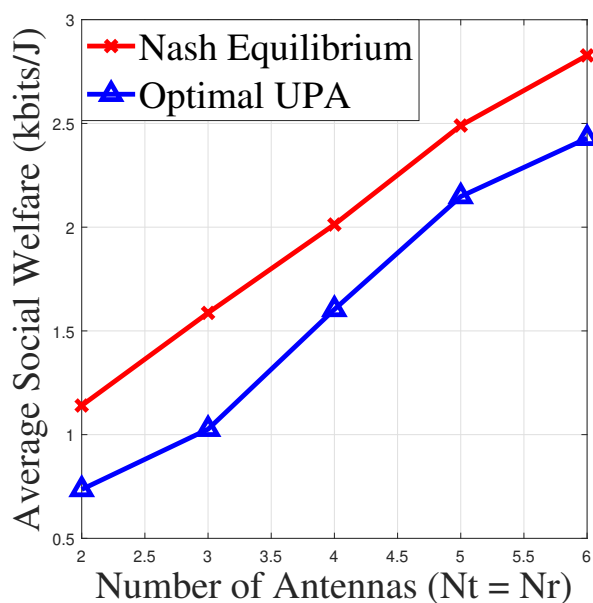
FIGURE 6.2 – Average social welfare under NE and uniform power allocation as function of number of antennas ( N_t = N_r ) with \bar{P}_k = 10\text{mW} for 2-user situation. NE found by our alg. 7 outperforms UPA
