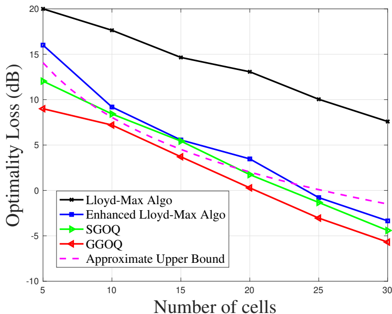
FIGURE 4.3 – Optimality loss (dB) as a function of number of cells for Lloyd-Max algorithm, approximate upper bound in Eq. 4.27, enhanced Lloyd-Max algorithm, SGOQ and GGOQ.
