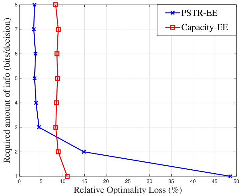
FIGURE 3.11 – Required bits of quantization v.s. relative optimality loss for utility function of case I (capacity as benefit function of EE) and case II (packet success transmission rate as benefit function of EE). Here, with B_2 = 6 bits/decision, the curves are much steeper, indicating that the choice of the number of feedback rate is more critical in this regime as soon as small optimality losses are desired.
