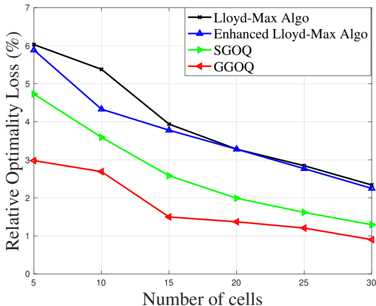
FIGURE 4.5 – Relative optimality loss v.s. number of cells for Lloyd-Max algorithm, enhanced Lloyd-Max algorithm (using weighted parameter distribution \lambda_1(\mathbf{g}; f^{\text{SL}}) \phi(\mathbf{g}) instead of \phi(\mathbf{g}) ), SGOQ and GGOQ. Here d_2 = d_1 = 4 and P_{\max} = 20\text{mW} . Proposed two algorithms could largely reduce the relative optimality loss compared to Lloyd-Max algorithms (enhanced version includes).
