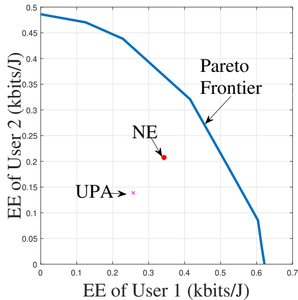
FIGURE 6.1 – Energy Efficiencyes under NE and uniform power allocation (UPA) with N_t = N_r = 2 for 2-user situation. NE found by our exact algorithm outperforms Uniform power allocation (UPA) policy.
