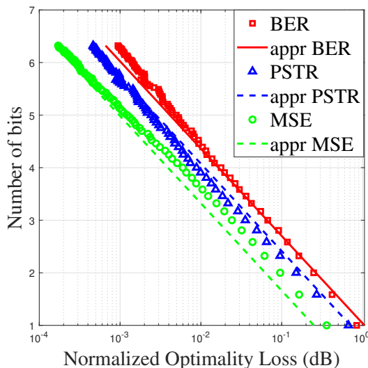
FIGURE 4.1 – Number of bits as a function of the normalized optimality loss (NOL) of EE (bit error rate) with N = 10 provided by enhanced LM algorithm (probability distribution is replaced by normalized value density), its approximate NOL, EE (packet success transmission rate) with c = 1 and its approximate NOL and MSE and its approximate NOL in dB. This figure reveals the accuracy of our high-resolution approximation. Our approximation in high-resolution regime could explain easily the hardness of quantization for different cost functions in scalar case.
