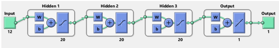
FIGURE 3.4 – Feed-forward neural network model for MIMO system ( N_t = 3 and N_r = 2 ). Number of neurons in input layer is 2N_tN_r .
