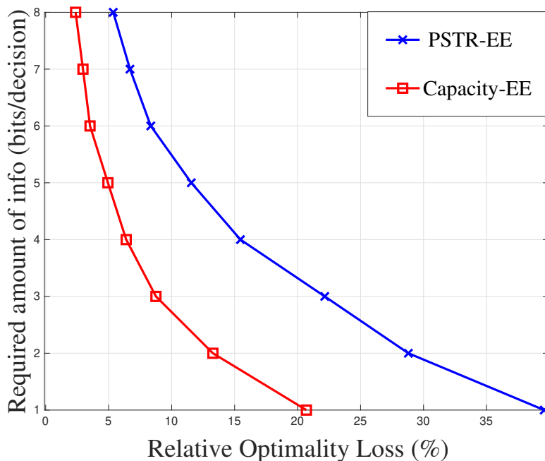
FIGURE 3.10 – Required bits of quantization v.s. relative optimality loss for utility function of case I (capacity as benefit function of EE) and case II (packet success transmission rate as benefit function of EE) with B_1 = 4 bits/decision. Here, it is seen that considering the packet success rate as benefit function of EE requires more feedback resources than using the capacity function. Remarkably, it is possible to quantify this extra amount of resources..
