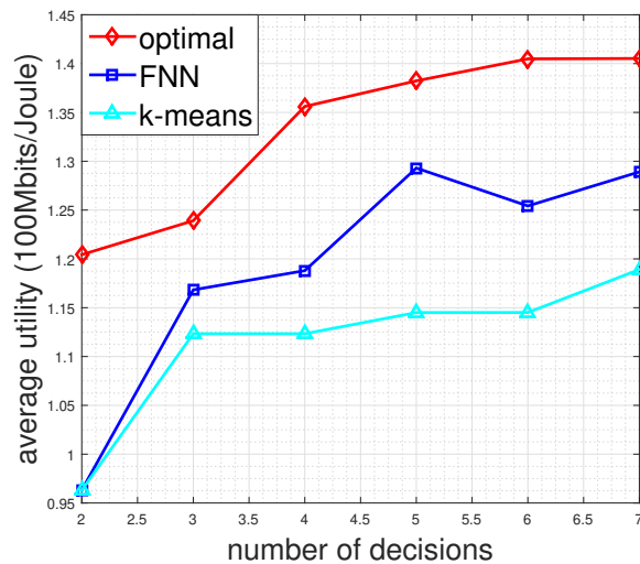
FIGURE 3.6 – Average utility vs. number of decisions for N_t = 3 and N_r = 2 (MIMO) , \sigma^2 = 5\text{mW} , P_0 = 10\text{mW} and P_{\max} = 10\text{mW} . FNN is better than k-means quantizer and close to theoretical optimal utility.
