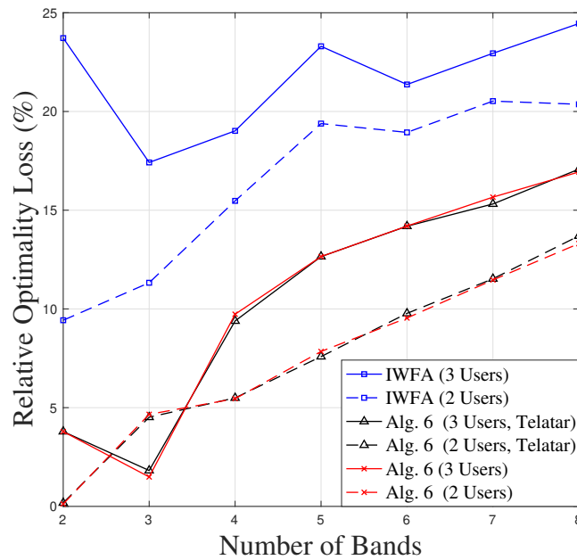
FIGURE 5.3 – Relative optimality loss (%) of average social welfare as a function of number of bands for iterative water-filling algorithm(IWFA), alg. 6 with Telatar set as the underlying action space, and alg. 6 for 2-user and 3-user scenarios with P_{\max} = 1\text{mW} and \sigma^2 = 1\text{mW} and number of actions is fixed as M = 4 . Braess’s Paradox always exists and optimality loss grows for all approaches as the number of bands increases.
