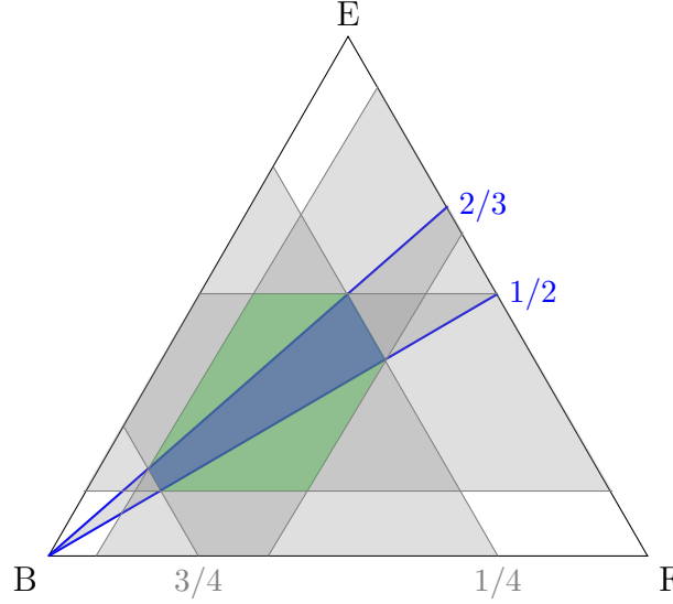
Figure 6.4: Set of realization probabilities \Pi_\Theta (green hexagon), rectangular set of probabilities \Pi_\Theta^R (blue rectangle). The grey numbers indicate the set of probabilities for B , the blue numbers the set of conditional one-step-ahead probabilities for E .
