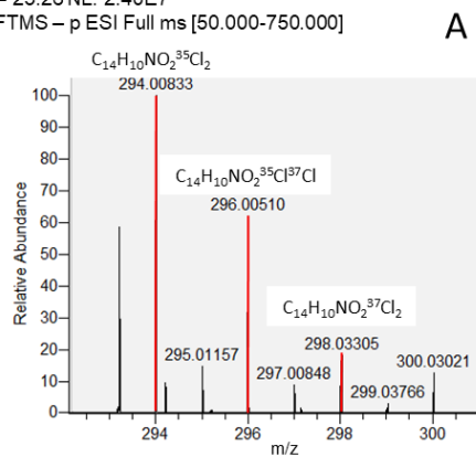
Figure S5: Negative ESI (A) isotopic pattern of DCF ( m/z 294) and (B) fragments of interest in MS 2 (20 eV) in a tissue sample of L. stagnalis exposed 7 days to DCF.
