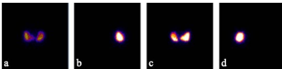
Figure 5.13: Simulated SPECT projections for the 2-organ phantom at different projection angles: a) 0^\circ , b) 90^\circ , c) 180^\circ and d) 270^\circ as the gamma camera in auto-contouring motion moves clockwise. a) spleen is on the left and the right kidney on the right, b) shows the right kidney, c) 180^\circ shows the inverse of a) and d) highlights the spleen
