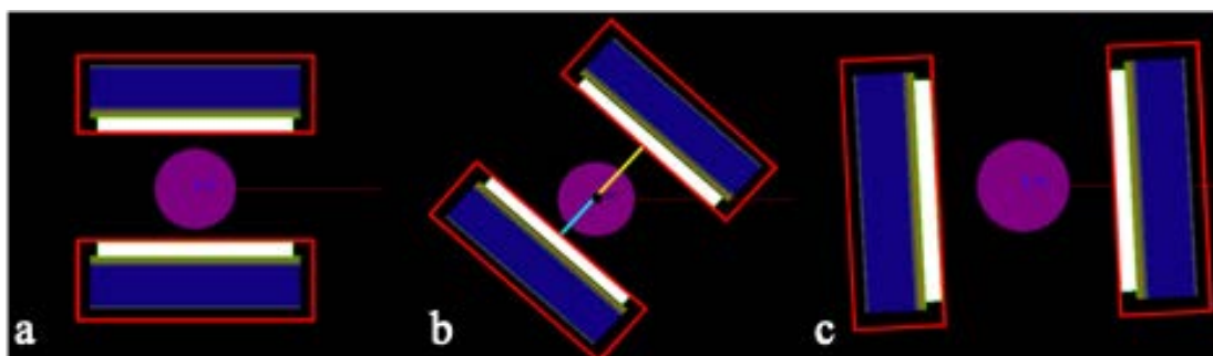
Figure 5.12: Auto-contouring motion of the gamma camera around the 2-organ phantom model. a) Detector heads at 0^\circ and 180^\circ , b) Detector heads at 45^\circ and 225^\circ , c) Detector heads at 90^\circ and 270^\circ Collimator (white); Crystal (grey); PMT (blue); SPECT head (red); phantom model (purple)
