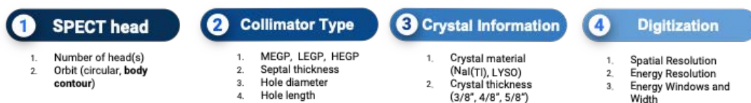
Figure 5.3: Schematic of modelling the gamma camera components and its response
