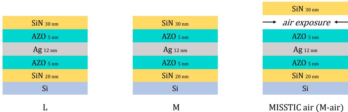
Figure 4.9 Schematic representation of the LINA (L), MISSTIC (M) references and the MISSTIC stack exposed to air (M-air).
