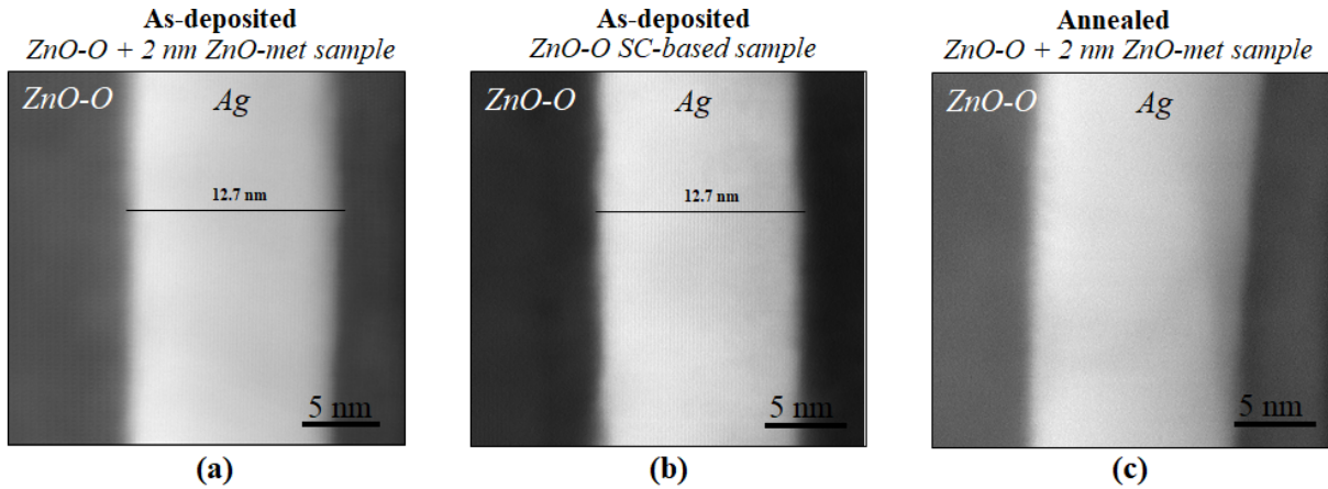
Figure 5.6 STEM cross section of the Ag-based stacks of (a) a ZnO-O + 2\text{ nm} ZnO-met buffer and (b) a ZnO-O reference sample. It is not possible to distinguish the buffer layer from the single crystal. In passing, the silver thickness agrees with XRR estimate. (c) STEM cross section of a ZnO-O + 2\text{ nm} ZnO-met buffer after annealing at 350^\circ\text{C} for 10 min.
