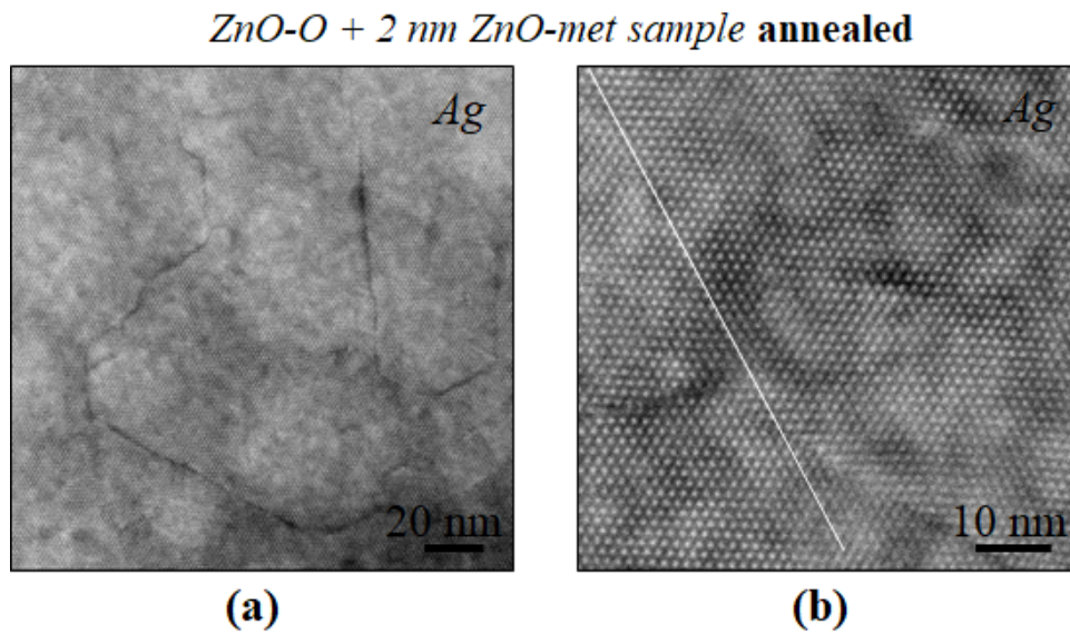
Figure 5.16 (a-b) STEM plane view of an annealed ZnO-O + 2 nm ZnO-met buffer sample. The clear Moiré pattern originates from the hexagon/hexagon epitaxy as sketched in Fig. (5.17)-b. The periodicity of \sim 1.6 nm corresponds to the overlap of atomic columns of ZnO and Ag as shown in Fig. (5.17)-b. The line in figure (b) shows that darker areas correspond to anti-phase domain boundary delineating domains of a few tens of nanometres.
