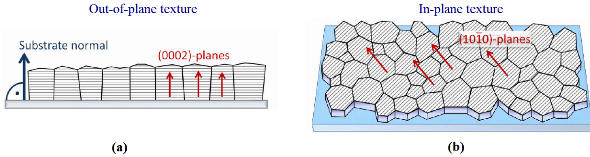
Figure 2 Sketch of oriented ZnO grains (a) along the perpendicular direction of the surface, the so-called out-of-plane texture, and (b) along the surface plane, the so-called in-plane texture [3])
