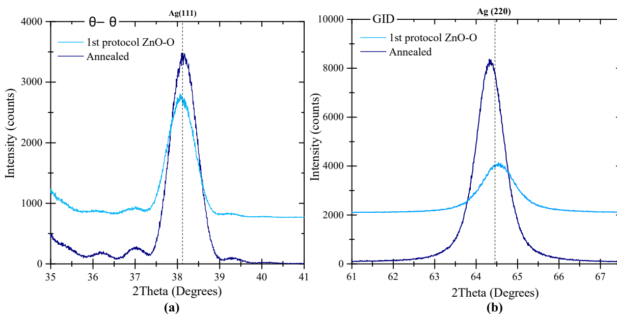
Figure 4.27 (a) \theta - 2\theta and (b) grazing incidence diffractograms of the O-terminated ZnO sample, treated with the first protocol, before and after annealing.
