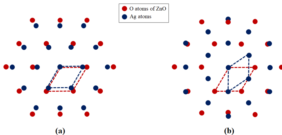
Figure 1.21 Representation of the in plane epitaxy of Ag(111)||ZnO(000 \bar{1} )-O : (a) hexagon/hexagon and (b) rotated orientations.
