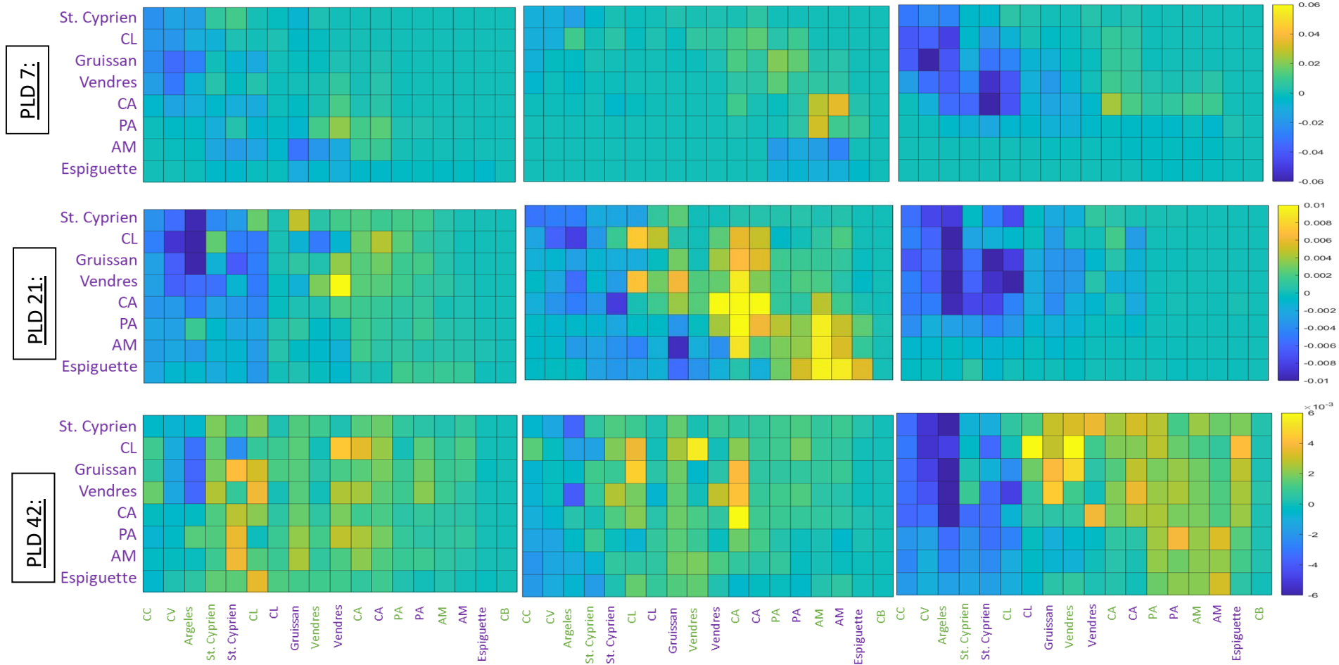
Figure 3.6: Difference in transfer rates (%) between the connectivity matrices with and without added error for different release periods and different PLDs (days). The natural substrate zones are depicted in green and the artificial substrate zones are depicted in purple. On the y-axes are the release zones, on the x-axis are the arrival zones. Every square is the average transfer rate between the two zones. Notice the difference in colour scales.
