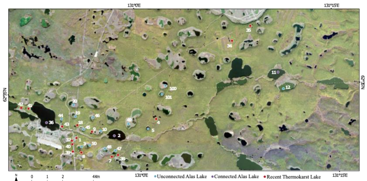
Figure 3. Map showing the complete distribution of sampled lakes for all four seasons by lake type. Unconnected alas lakes are indicated by a blue point, recent thermokarst lakes are indicated by a red point, and connected alas lakes are indicated by a purple point.
