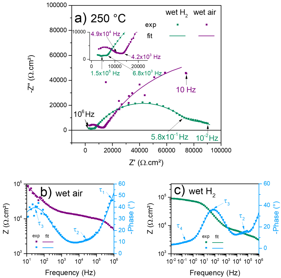
Figure D.9: EIS spectra of BZY-b symmetrical cell at 250 °C. a) Nyquist plot; b) Bode plot in wet air and c) Bode plot in wet \text{H}_2 . The insert in the Nyquist plot exposes a zoom of the high frequencies points.
