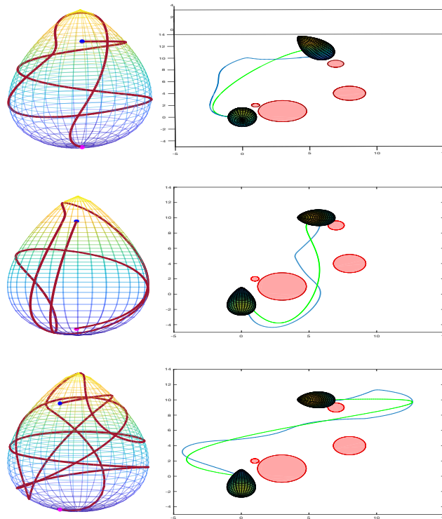
Figure 3.6: Left side: curve \gamma_2 on the egg. Right side: Curve obtained by applying the Continuation Method (blue) to initial chosen curve (green).
