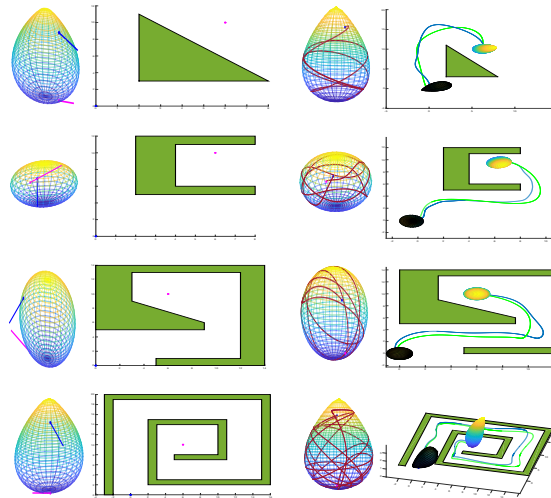
Figure 2.2: Different examples of bodies rolling on the plane with obstacles.
