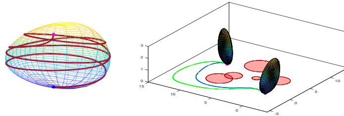
Figure 3.10: Left side: Non-symmetric convex body with initial and end contact points and curve \gamma_2 . Right side: Curve obtained by applying the Continuation Method (blue) to the initial chosen curve (green).
