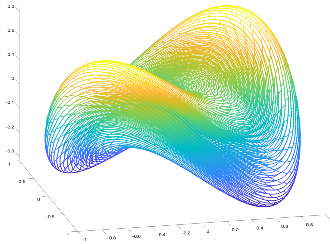
Figure 3.2: Ball in 3-D generic case.
