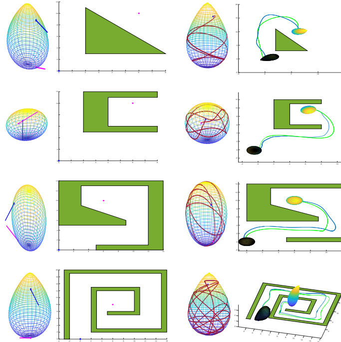
Figure 3.9: Left side: convex body with initial and end contact points with orientations and obstacles on the plane (in green). Right side: curve \gamma_2 on the convex body and curve obtained by applying the Continuation Method (blue) to the initial chosen curve (green).
