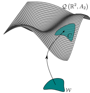
Figure 3.1: Obstacle maps in M .
