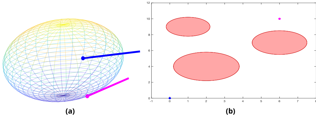
Figure 3.3: Left side: sphere with initial and end contact points and its orientations. Right side: obstacles (in red) and initial and end contact points on the plane.
