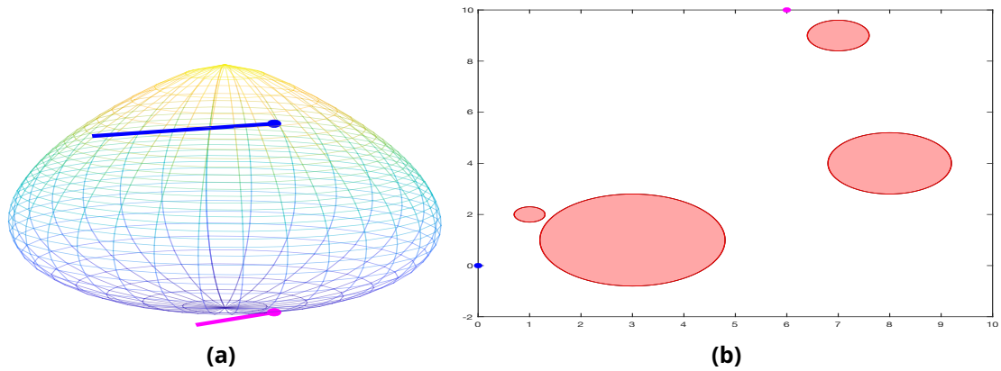
Figure 3.5: Left side: egg with initial and end contact points and its orientations. Right side: obstacles (in red) and initial and end contact points on the plane.
