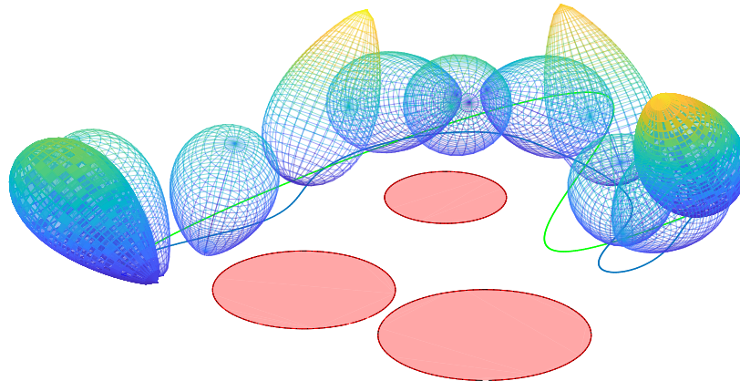
Figure 3.2: Convex body rolling along the curve obtained by the application of the Continuation Method (blue curve).
