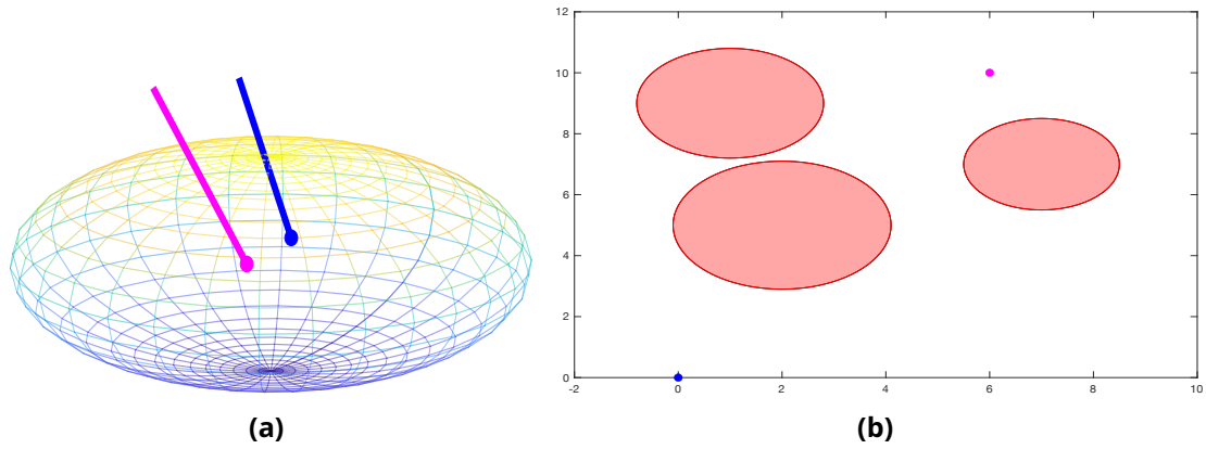
Figure 3.7: Left side: flattened ball with initial and end contact points and its orientations. Right side: obstacles (in red) and initial and end contact points on the plane.
