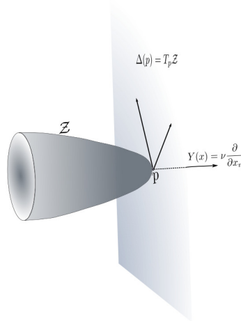
Figure 4.1: Singular set and its tangent space at p with the translation vector Y(x) .
