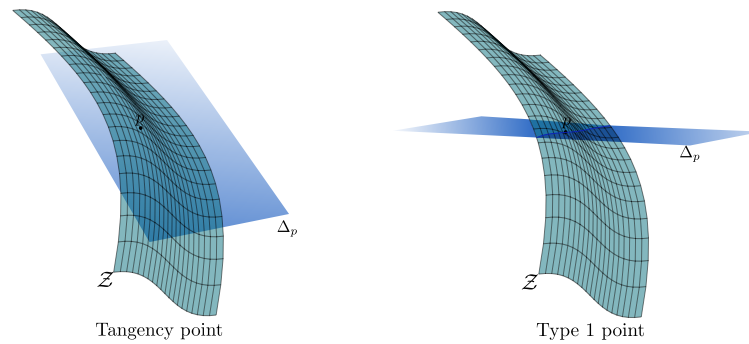
Figure 2.1: Two different points from \mathcal{Z} in the 3-D generic case.
