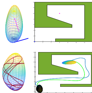
Figure 3.11: Top: Non-symmetric convex body with initial and end contact points with orientations and obstacle on the plane (in green). Bottom: curve \gamma_2 on the convex body and curve obtained by applying the Continuation Method (blue) to the initial chosen curve (green).
