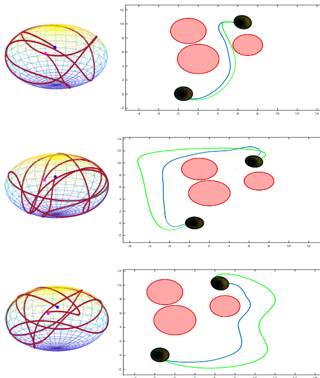
Figure 3.8: Left side: curve \gamma_2 on the flattened ball. Right side: curve obtained by applying the Continuation Method (blue) to initial chosen curve (green).
