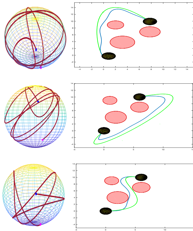
Figure 3.4: Left side: curve \gamma_2 on the sphere. Right side: Curve obtained by applying the Continuation Method (blue) to initial chosen curve (green).
