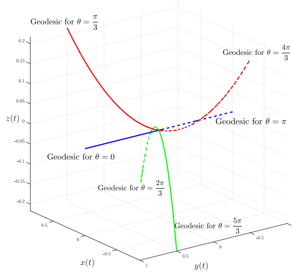
Figure 3.1: Geodesics for \theta \in \{0, \frac{\pi}{3}, \frac{2\pi}{3}, \pi, \frac{4\pi}{3}, \frac{5\pi}{3}\} when r = 0 .
