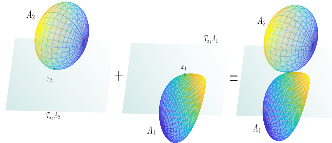
Figure 2.1: Identification of tangent spaces at a contact point.
