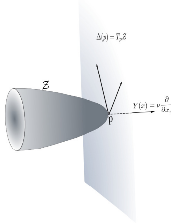
Figure 2: Singular set and its tangent space at p with the translation vector Y(x) .
