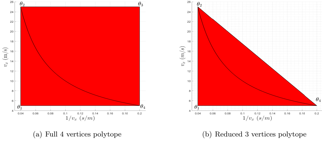
Figure 4.1: Full and Reduced Conservatism Polytopes w.r.t the real parameters variations.
