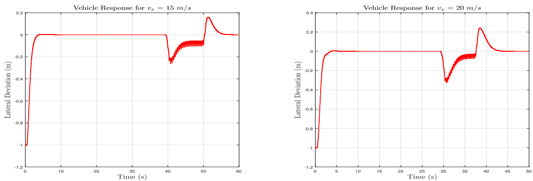
(c) Lateral deviation response for speed test v_x = 15 m/s (d) Lateral deviation response for speed test v_x = 20 m/s
