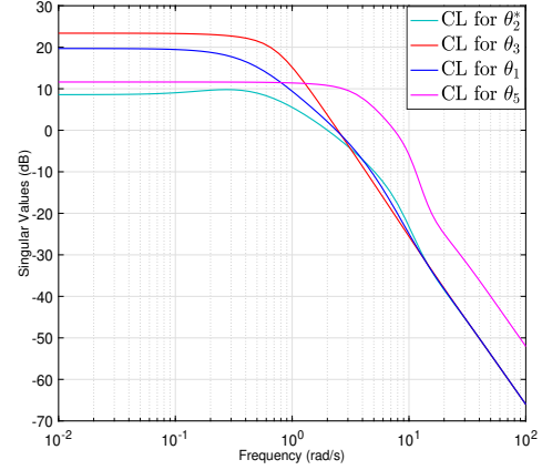
(b) Frequency response y_L/r .
