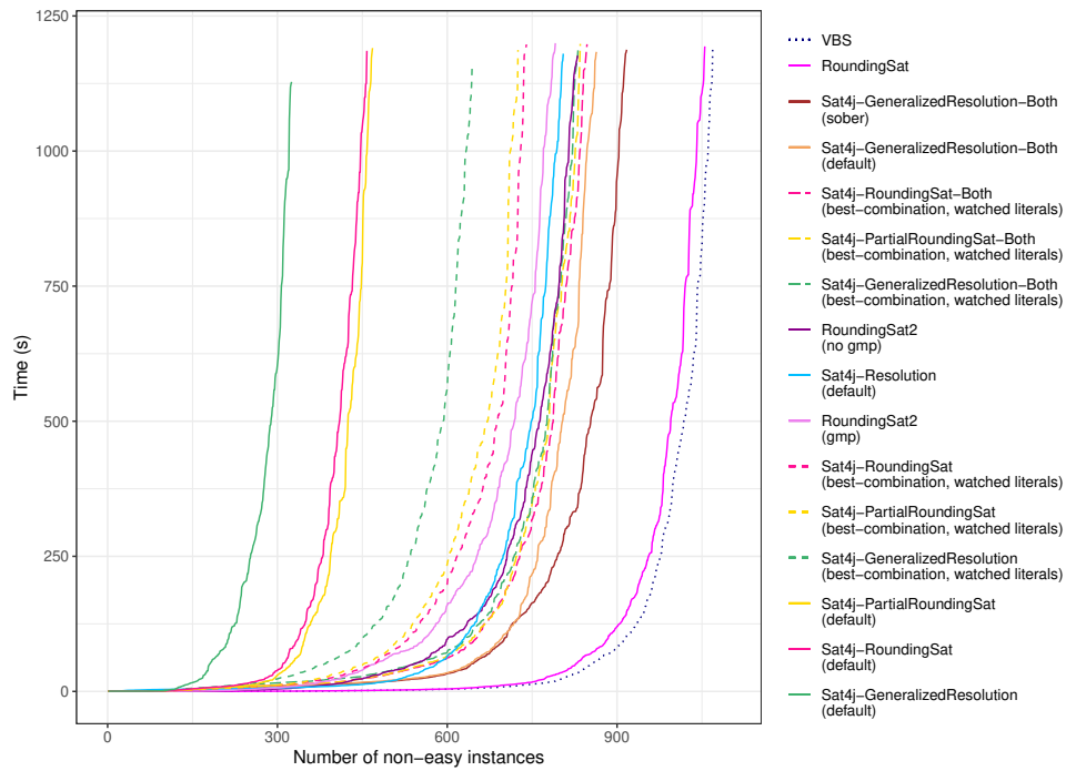
Figure 7.28: Cactus plot comparing several configurations of Sat4j with different versions of RoundingSat (using watched literals).
