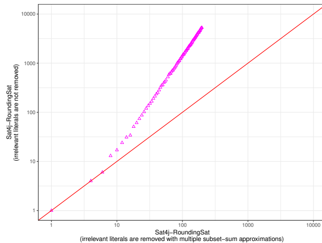
Figure 5.23: Scatter plot comparing the number of cancellations performed during the execution of Sat4j-RoundingSat on the vertexcover-completegraph family with the removal of irrelevant literals activated (with the ad hoc algorithm) and without (logarithmic scale).
