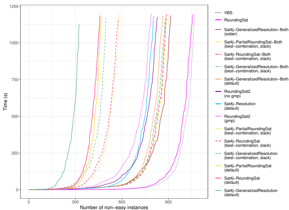
Figure 7.27: Cactus plot comparing several configurations of Sat4j with different versions of RoundingSat .
