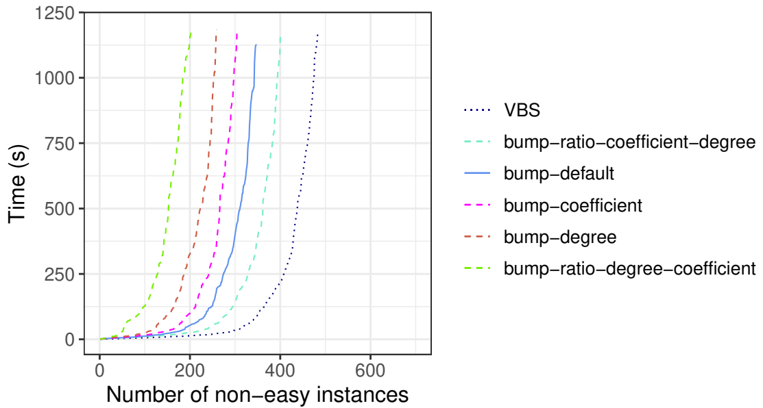
Figure 7.1: Cactus plot of the various coefficient and degree-based bumping strategies implemented in Sat4j-GeneralizedResolution .
