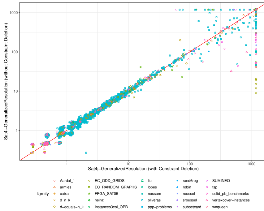
Figure 4.8: Comparison of the runtime (in seconds) of Sat4j-GeneralizedResolution with and without learned constraint deletion enabled (logarithmic scale).
