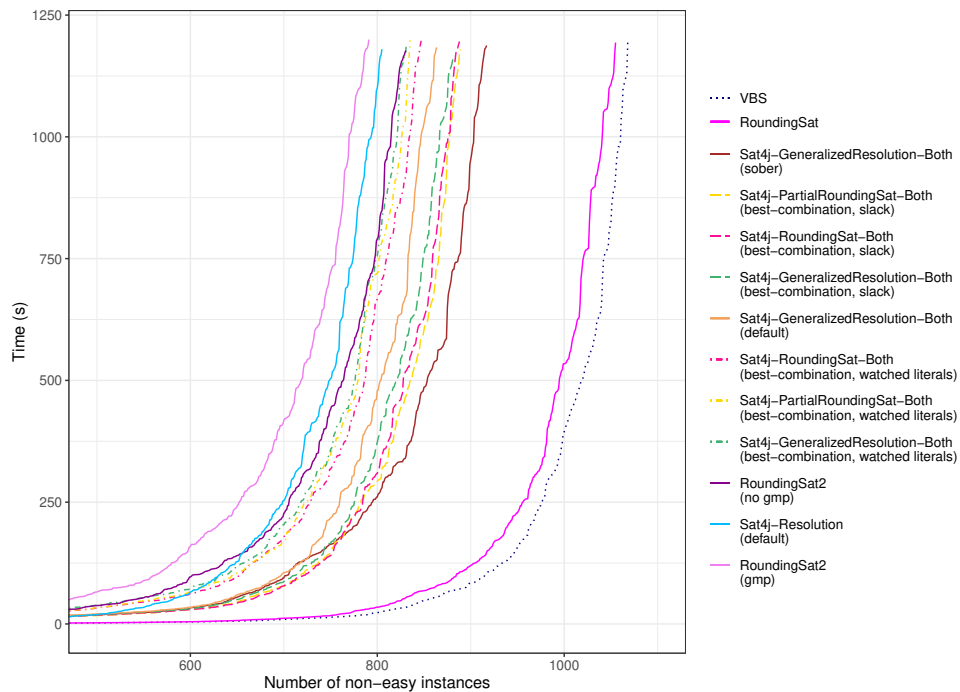
Figure 7.29: Cactus plot comparing several configurations of Sat4j with different versions of RoundingSat (many core solvers).
