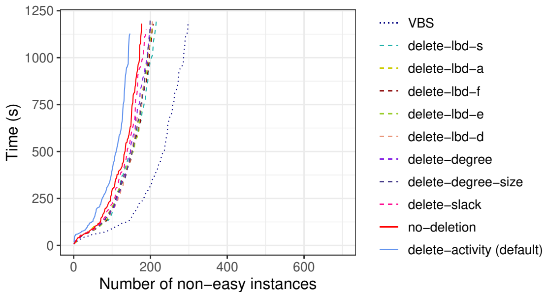
Figure 7.8: Cactus plot of the various learned constraint deletion strategies implemented in Sat4j-GeneralizedResolution .
