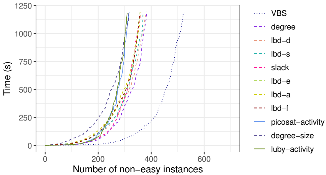
Figure 7.18: Cactus plot of the various quality measures used for learned constraint deletion and dynamic restarts in Sat4j-PartialRoundingSat .
