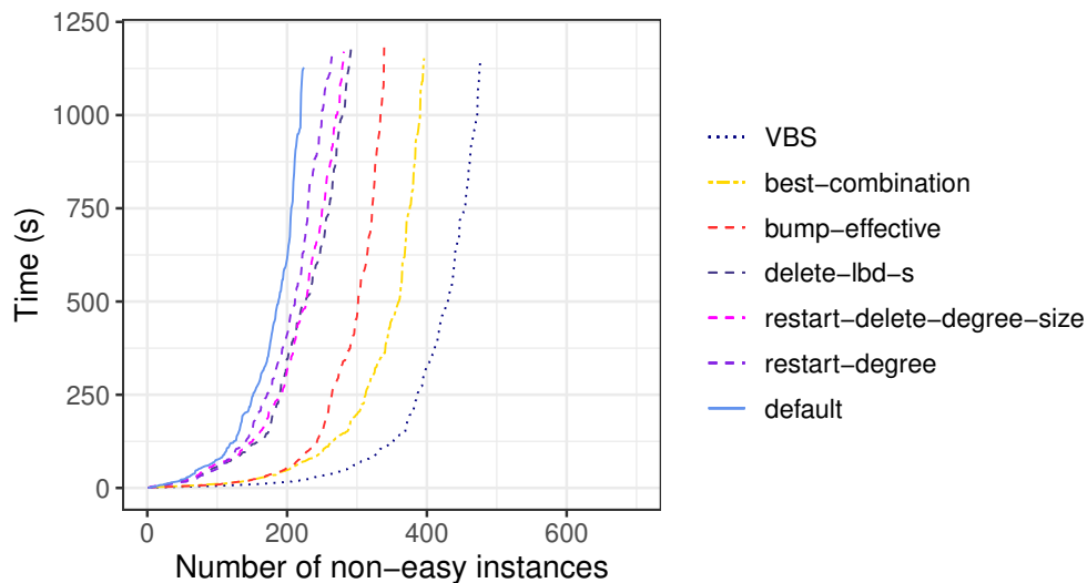
Figure 7.20: Cactus plot of the best strategies enabled in Sat4j-GeneralizedResolution .
