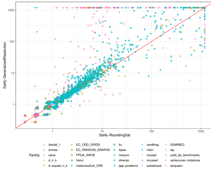
Figure 4.4: Scatter plot comparing the runtime (in seconds) of Sat4j-GeneralizedResolution and Sat4j-RoundingSat , in logarithmic scale.
