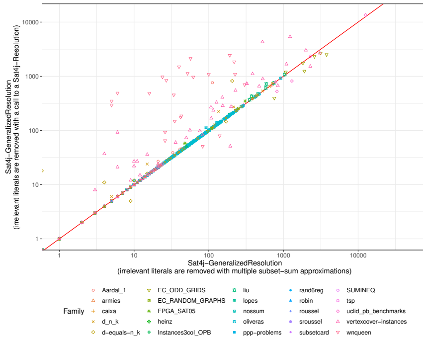
Figure 5.9: Scatter plot comparing the number of irrelevant literals detected using the ad hoc algorithm and the SAT-based approach in Sat4j-GeneralizedResolution (logarithmic scale).
