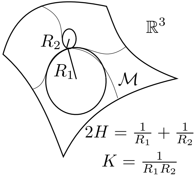
Figure 1.6: Schematic of principal radii of curvature, R_1 and R_2 , on a 2D manifold \mathcal{M} embedded in \mathbb{R}^3 .
