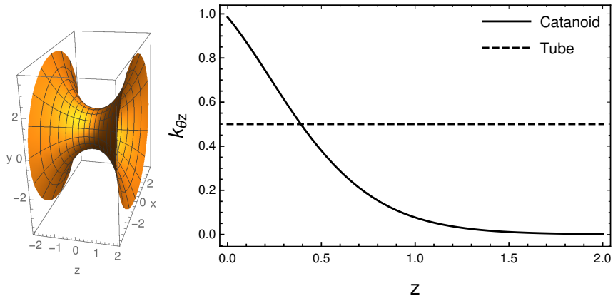
Figure B.3: Left: plot of the catenoid with radius r_0 = 1 . Right: Plot of the force linear response coefficient for the mixed shape derivative ( i.e. the term in the normal force that goes like f \sim k_{\theta z} \partial_{\theta z} u ) for the helical shape perturbations on such a surface.
