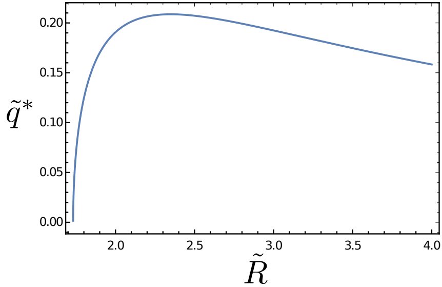
Figure 2.2: Location of the peak of the growth rate ( \tilde{q}^* \equiv R_{eq}q^* ) for a tube under constant tension, as a function of the tube radius. The initial tube radius R_{eq} corresponds to the equilibrium radius of a tube under zero pressure.
