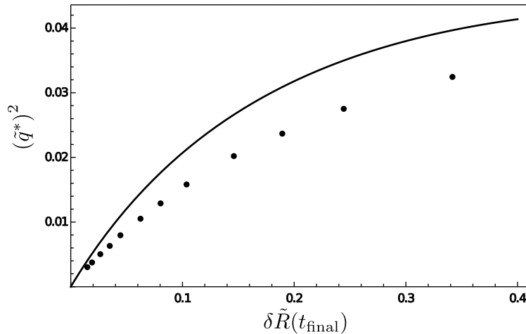
Figure 2.6: Dominant wave-number squared, (\tilde{q}^*)^2 , plotted against final radius minus critical radius \delta\tilde{R}(t_{\text{final}}) = \tilde{R}(t_{\text{final}}) - \sqrt{3} , the solid line corresponds to the peak of the growth rate as a function of wavenumber and points represent the peak found by numerically solving the full dynamics.
