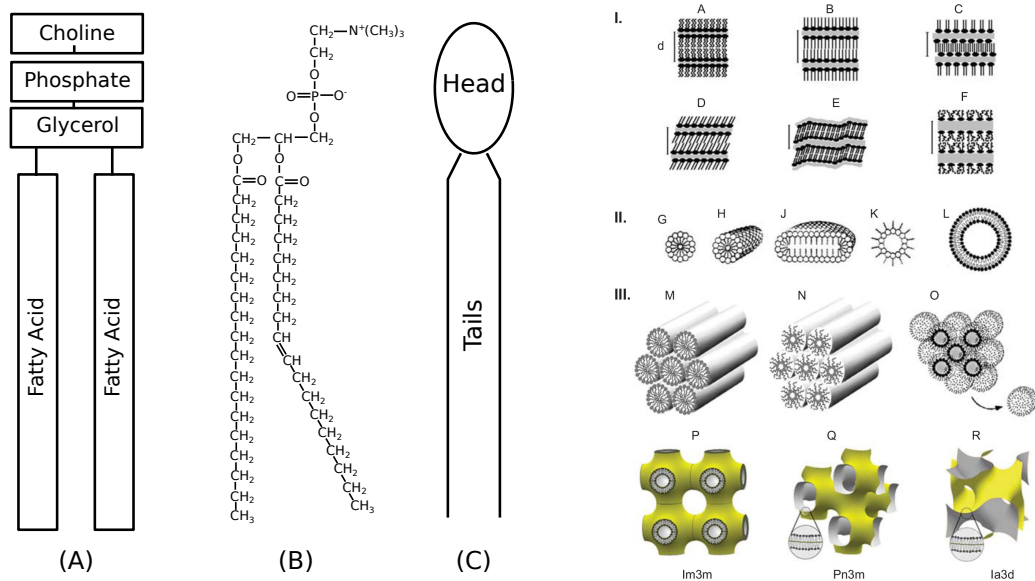
Figure 1.2: Left Panel: (A) Shows the general structure of a lipid molecule, (B) Specific chemical structure of Phosphatidylcholine, (C) Hydrophilic head and hydrophobic tail representation. Figure is a reproduction of a similar figure in [Alberts et al., 2002]. Right Panel: Figure taken from [Koynova and Tenchov, 2013] showing the vast phase space lipid membranes can occupy; I. Lamellar phases, II. Micelles and Liposomes & III. Non-lamellar liquid-crystalline phases.
