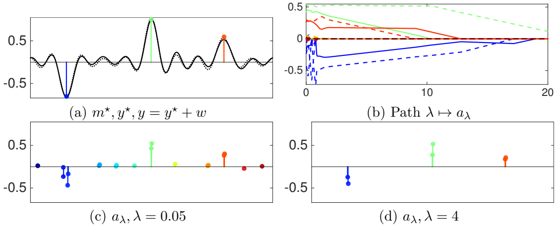
Figure 5.5: Sparse spikes deconvolution results obtained by computing the solution a_\lambda of (\mathcal{P}^{\ell^1(\mathcal{G}_n)})(\lambda, y) . The color reflects the positions of the spikes on the 1-D grid. (a) shows the input measure m^* and the observation y = y^* + w . (b) shows how the solution a_\lambda (vertical axis) evolves with \lambda (horizontal axis). Each curve shows the evolution of \lambda \mapsto (a_\lambda)_i for indexes i \in \{1, \dots, G - 1\} . The color encodes the value of i . Plain curves correspond to correct spikes locations i associated to the input measure m^* . Dashed curves correspond to incorrect spikes (not present in the input measure m_0 ). (c,d) show the results a_\lambda obtained for two different values of \lambda .
