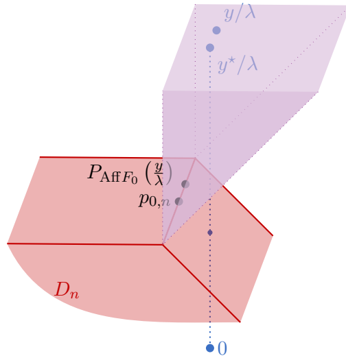
Figure 5.6: Illustration of the proof of Theorem 5.4 . The solution set to the dual problem \mathcal{D}^{\ell^1(\mathcal{G}_n)}(0, y^*) is the horizontal face, but the solution with minimal-norm p_{0,n} lies on the smaller face (edge) F_0 . For \lambda and \|y - y^*\|_{\mathcal{H}}/\lambda small enough, the projection of y/\lambda onto D_n is P_{\text{Aff } F_0}(\frac{y}{\lambda}) .
