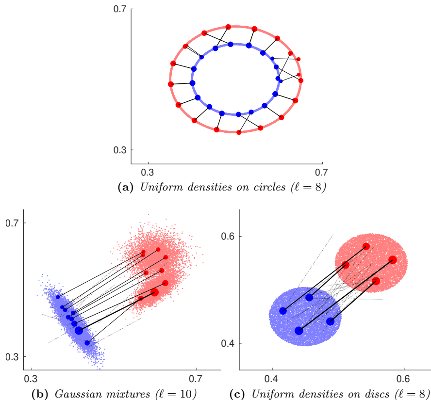
Figure 7.14: Examples of transport between “continuous” measures recovery using the FFW algorithm.
