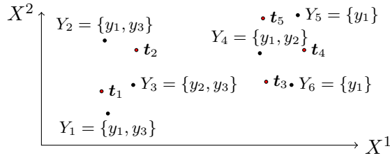
FIGURE 2.2: 3-nn classifiers
