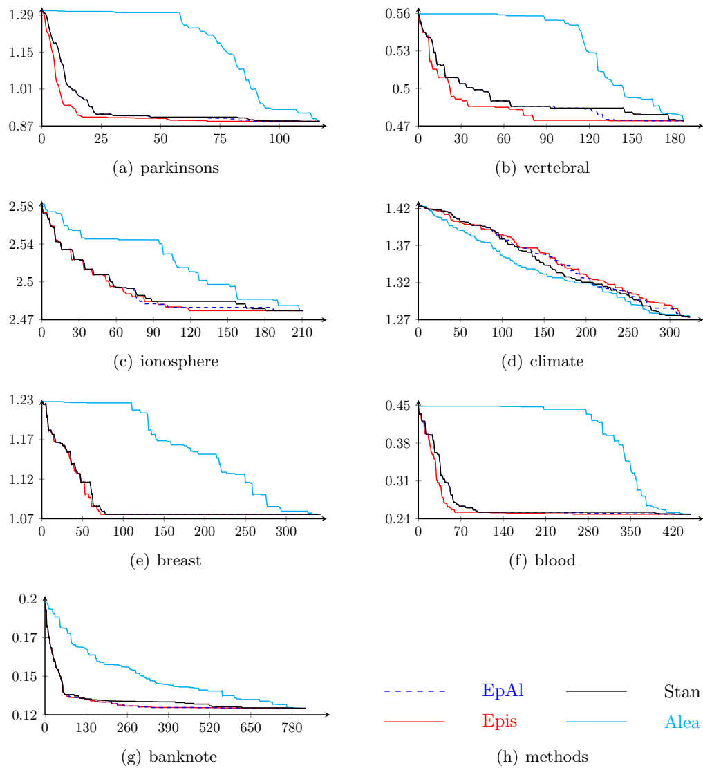
FIGURE 4.4: Average maximum distances (y-axis) over 5 \times 5 -folds for the Parzen window classifier ( K = 8 ) as a function of the number of examples queried from the pool (x-axis).
