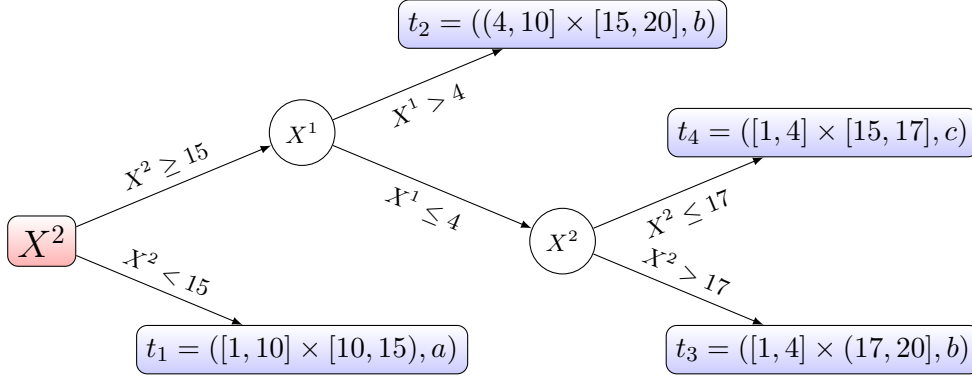
FIGURE 3.8: Decision tree illustration \theta_l
