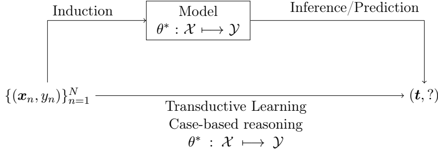
FIGURE 1.1: Inductive versus transductive learning
