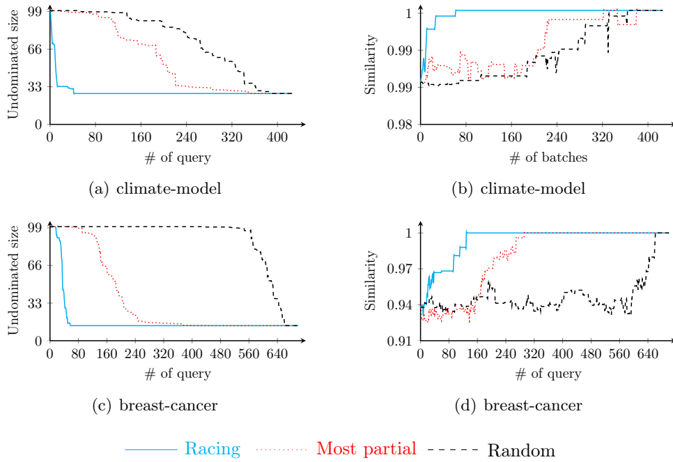
FIGURE 3.5: Experiments for interval-valued features data with preferred model
