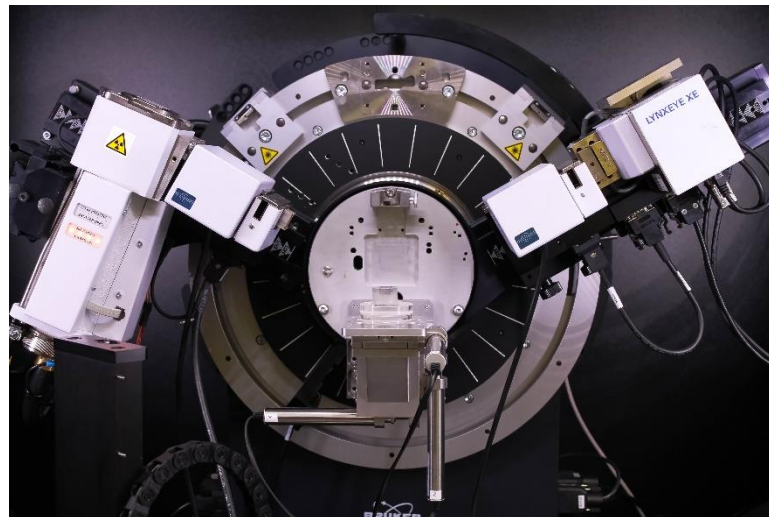
Figure III.5 : DRX (Bruker D8 DISCOVER, source ICB).
