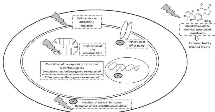
Figure 1. Schematic representation of mechanisms involved in the reduction of mycotoxin contamination (dotted line: fungicide/fungistatic actions, solid line: anti-mycotoxin synthesis activity, dash line: detoxifying activity)
