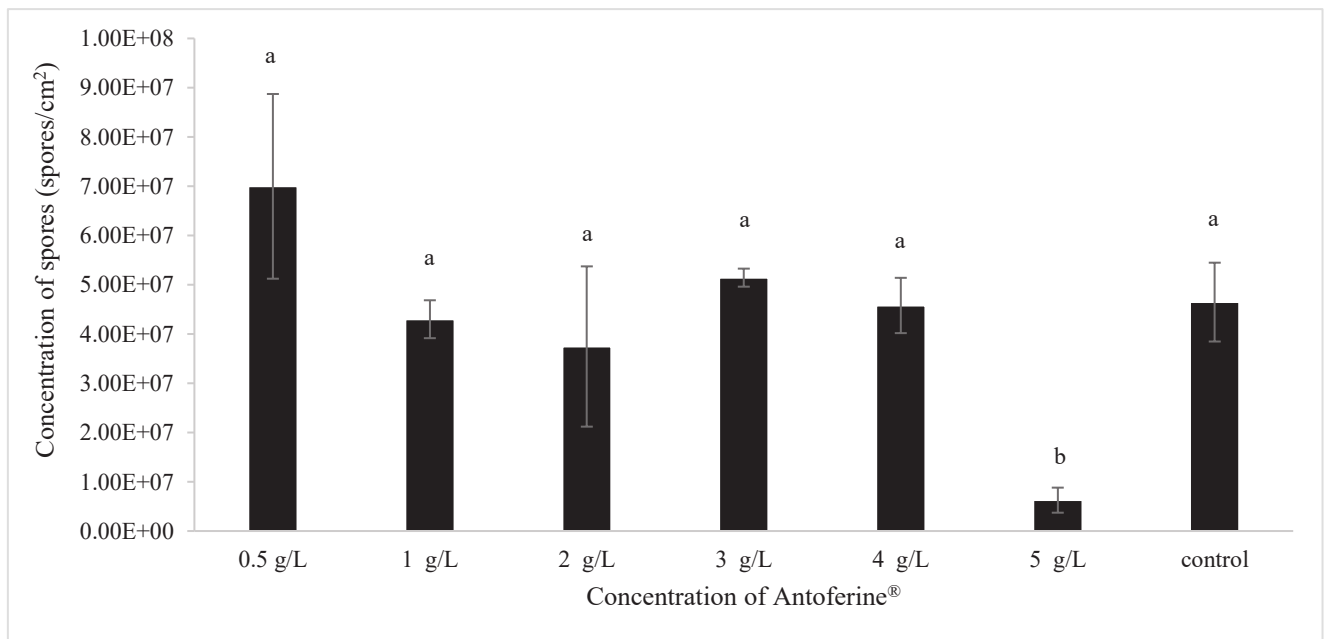
Fig. 2 Effect of different concentrations of Antoferine® on spore production after 5 days in PDA medium at 25 °C. (a) for A. flavus . (b) for A. carbonarius . (c) for F. verticillioides .
