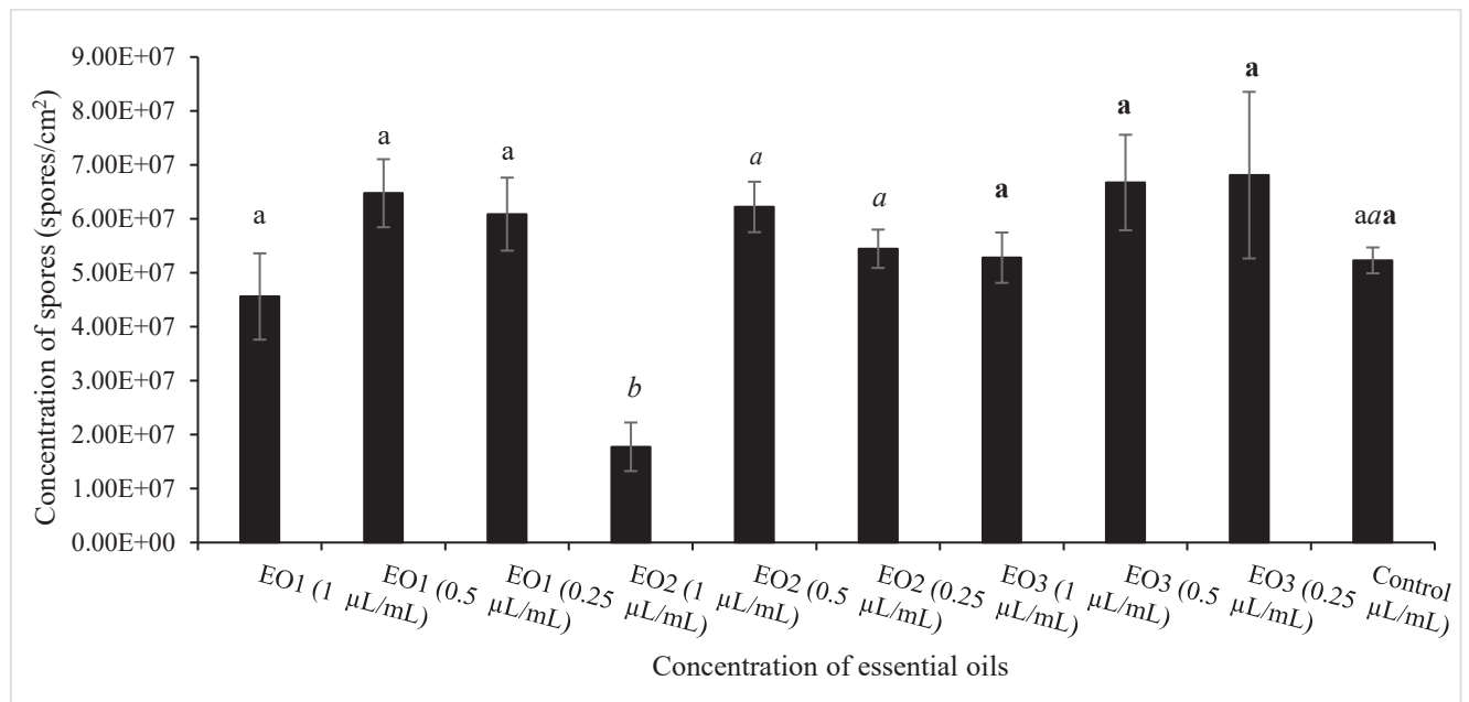
Fig. 3 Effects of different concentration of C. schoenanthus (EO1), C. nardus (EO2) and E. camaldulensis (EO3) essential oils on spore production after 5 days in PDA medium at 25 °C. (a) for A. flavus . (b) for A. carbonarius . (c) for F. verticillioides . Differences between control and tested essential oils were determined separately for each EOs according to ANOVA and Tukey's multiple comparison tests. For each EOs, bars with different letters indicate significant differences ( p < 0.05 ).
