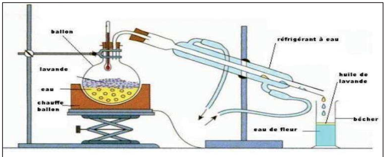
Figure 5: Principe de la distillation simple ( https://www.physicsforums.com/threads/hydrodistillation-and-original-uses ).
