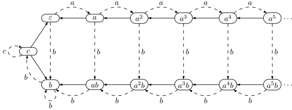
Figure 4: The outbidding condition: more b 's than a 's.
