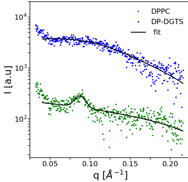
Figure S8. SAXS scattering curves of multilamellar vesicles made of DP-DGTS (blue symbols, scaled by 10) and DPPC lipids (green symbols) at T = 20\text{ °C} . Black lines are the best fit obtained.
