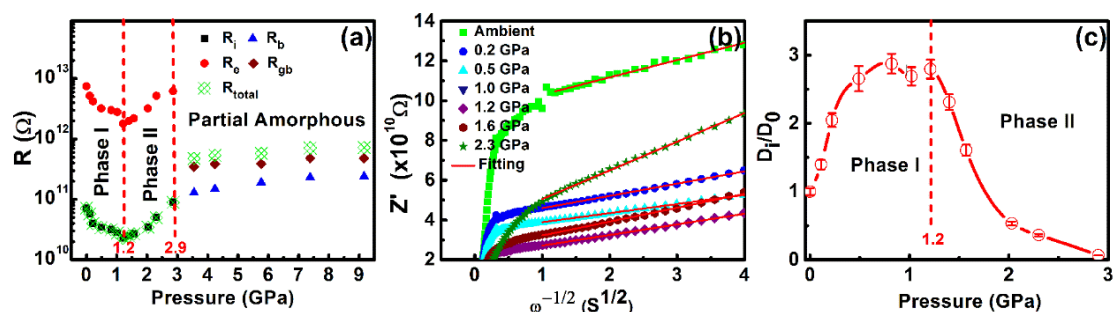
Figure 3.9 (a) Pressure dependence of R_i , R_e , R_b , R_{gb} , and R_{total} . (b) Z' as a function of \omega^{-1/2} plots at low frequencies from ambient pressure to 2.3 GPa. (c) Pressure dependence of the relative ionic diffusion coefficient from ambient pressure to 2.3 GPa.
