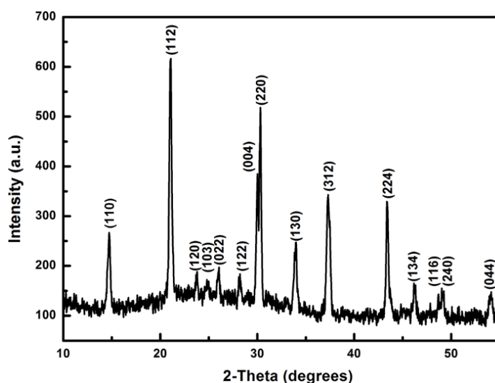
Figure 3.5 The XRD pattern of CsPbBr 3 powders.
