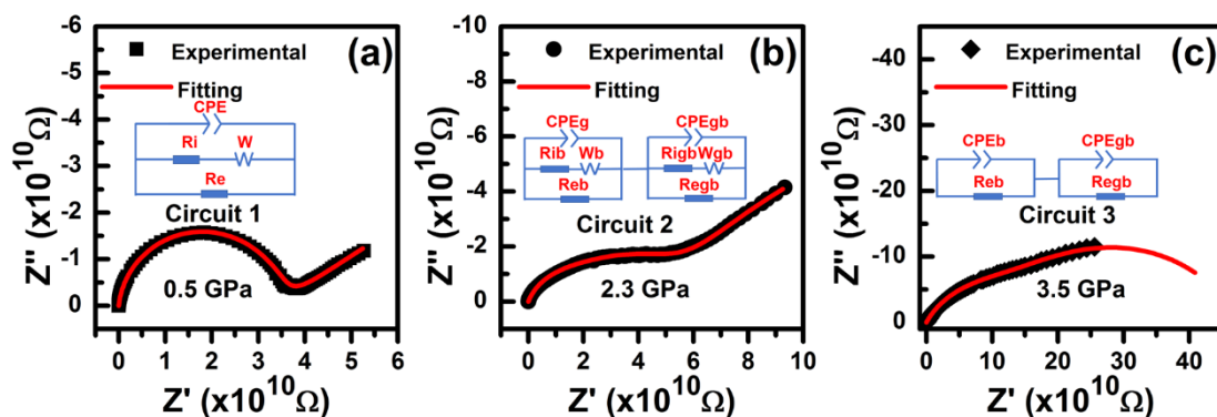
Figure 3.8. The experimental and fitting data for CsPbBr 3 powder impedance spectra at different pressures. (a) 0.5 GPa; (b) 2.3 GPa; and (c) 3.5 GPa.
