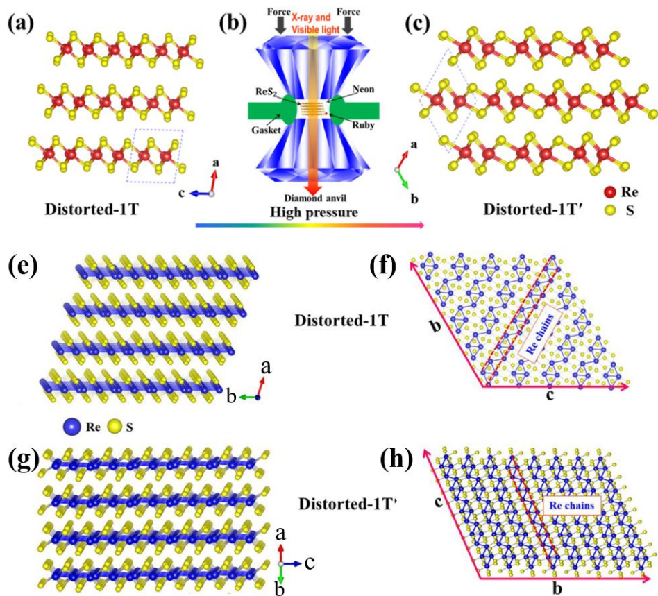
Figure 4.5 (a) The cross-section illustration of layered distorted-1T ReS 2 . (b) Schematic diagram of the high-pressure diamond-anvil cell setup. (c) The cross-section illustration of layered distorted-1T' ReS 2 . (e-h) Structure details of distorted 1T and 1T' ReS 2 . (e) The cross-section illustration of distorted 1T ReS 2 layers direction along a-axis. (f) Top view of the layer structure of a monolayer distorted 1T ReS 2 . Unit cell and Re chains are highlighted. (g) The cross-section illustration of distorted 1T' ReS 2 layers along \overline{xy} direction. (h) Top view of the layer structure of a monolayer distorted 1T' ReS 2 . Unit cell and Re chains are highlighted. 225
