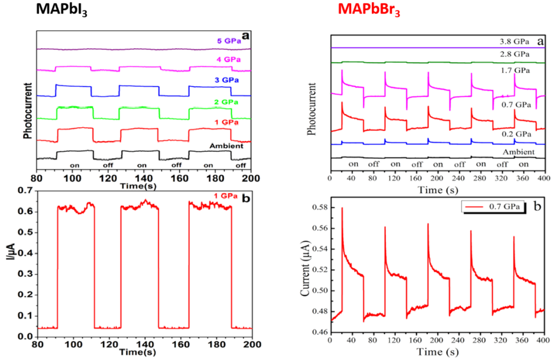
Figure 3.3 Left: (a) the pressure dependence of photocurrents in MAPbI 3 , (b) the detailed response of photocurrent at 1.0 GPa; Right: (a) The pressure dependence of photocurrents in MAPbBr 3 , (b) The detailed response of photocurrent at 0.7 GPa.
