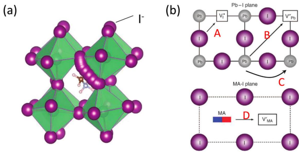
Figure 3.10 The schematic diagram of the ion movement paths in MAPbI 3 .
