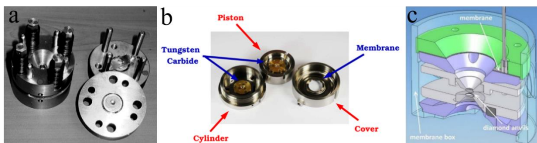
Figure 2.2 The picture of (a) MPDAC and (b) MDAC, (c) a stainless steel membrane is located in the cover. To generate pressure, helium is inflated into the membrane through the capillary tube.
