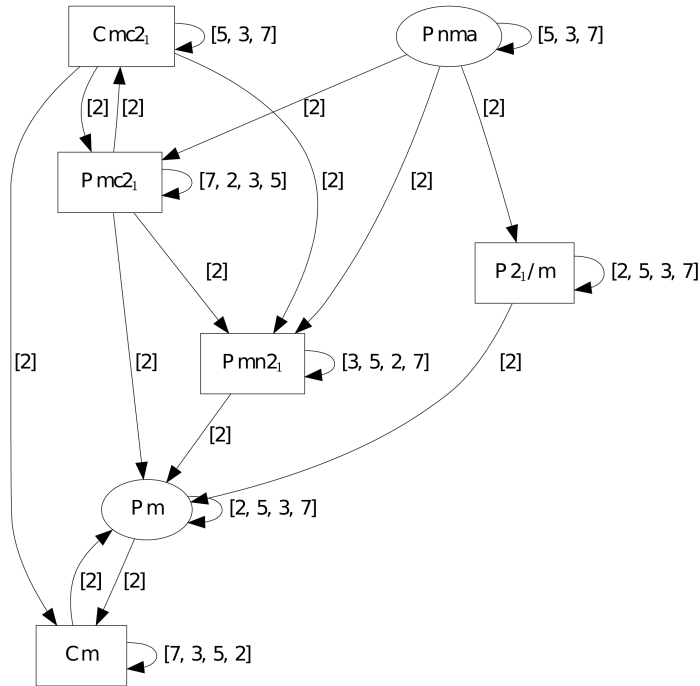
Figure 4.4: Group-Subgroup graph from Pnma to Pm .
