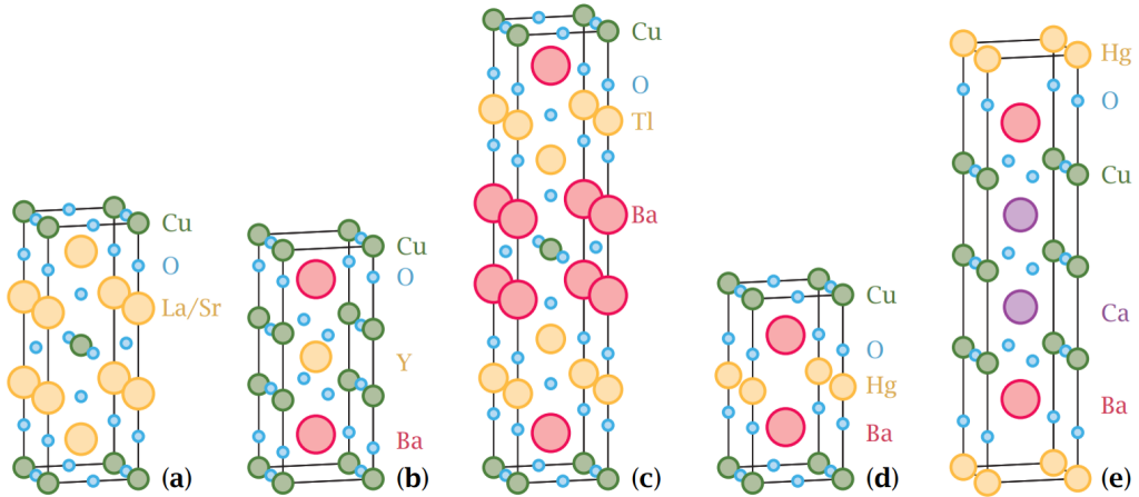
Figure 1.11: The crystal structures of (a) La_{2-x}Sr_xCuO_4 , (b) YBa_2Cu_3O_6 , (c) Tl_2Ba_2CuO_6 , (d) HgBa_2CuO_4 , (e) HgBa_2Ca_2Cu_3O_8 [91].
