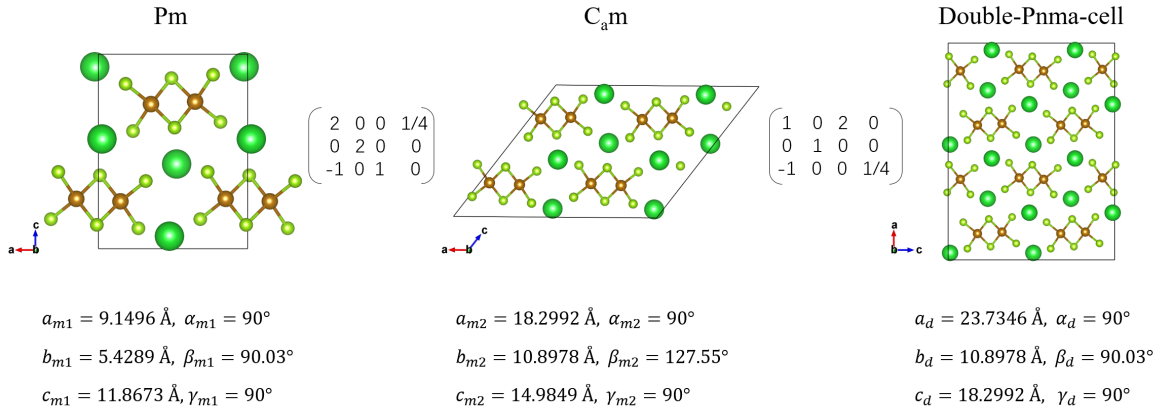
Figure 5.7: The crystal structures of Pm , C_m and \text{double-Pnma-cell} and the transformation matrices between them. The subscript m indicates the monoclinic cell and d for the double-setting cell.
