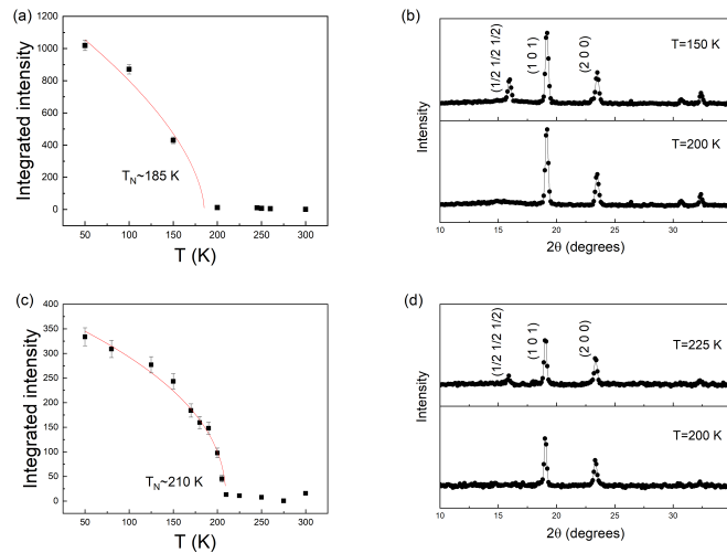
Figure 3.29: (a) and (c) Temperature dependence of the integrated intensity of the magnetic reflection (\frac{1}{2} \frac{1}{2} \frac{1}{2}) of C1 and C5. (b) and (d) Neutron powder diffractograms of C1 and C5 below and above T_N .
