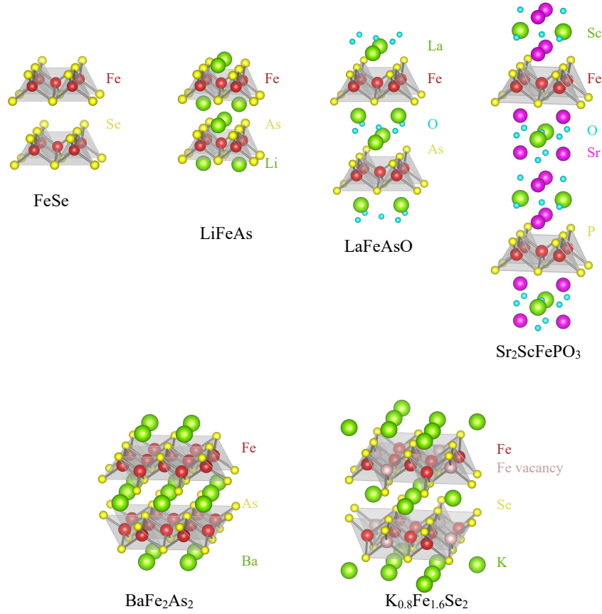
Figure 1.13: The crystal structures of the six classes of FeSCs. Note that the Fe layers in K 0.8 Fe 1.6 Se 2 are the same as in BaFe 2 As 2 but with Fe vacancies.
