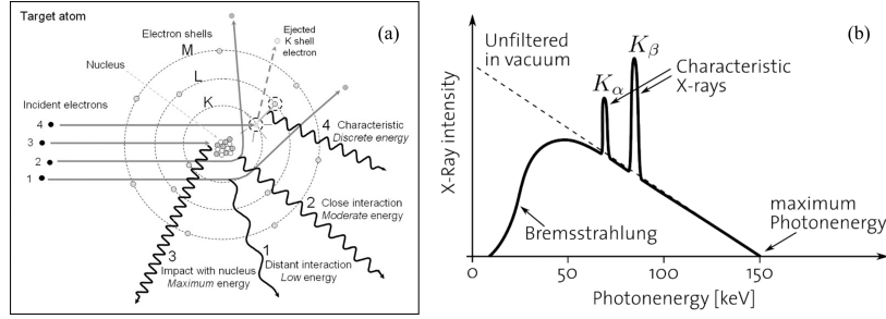
Figure 3.13: (a) Illustration of the bremsstrahlung (1,2,3) and characteristic (4) radiations [177]. (b) Typical X-ray spectrum produced by an X-ray tube [176].
