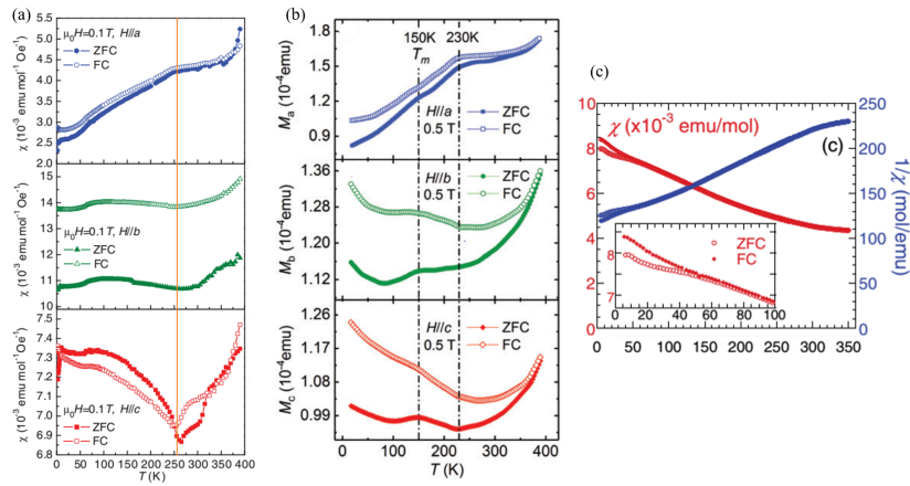
Figure 2.7: Temperature dependencies of dc magnetic susceptibility \chi(T) for \text{BaFe}_2\text{Se}_3 under ZFC and FC modes from reference [134] (a), [127] (b). The applied field is along a (top), b (middle), and c (bottom). (c) \chi(T) curves of \text{BaFe}_2\text{Se}_3 after ZFC and FC from reference [133]. The susceptibility are deduced under applied field of 5 T and subtract the one at 1 T to minimize effects from ferromagnetic impurity.
