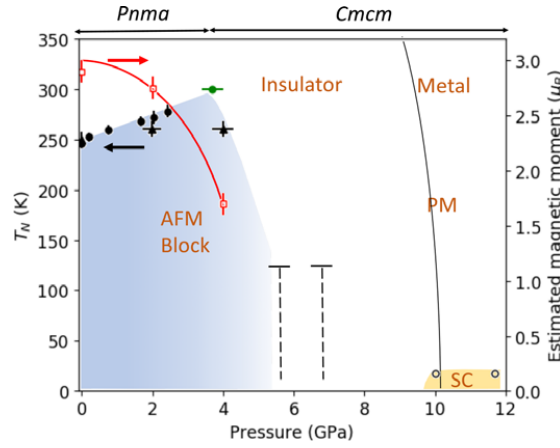
Figure 2.13: Pressure versus temperature phase diagram for \text{BaFe}_2\text{Se}_3 from experimental results [149]. The antiferromagnetic (AFM) transition temperature T_N (black symbols, left axis) and estimated ordered moment (red symbols, right axis) are shown. For the T_N determination, the filled circles and triangles represent the \mu\text{SR} and neutron diffraction results, respectively. The horizontal lines at the pressures of 5.5 and 6.8 GPa mark the lowest measured temperature of 120 K, at which the block-type short range magnetic correlations were observed. The green filled circle marks the structural transition [3.7(3) GPa] identified at room temperature. The superconducting dome and black line marking the metal-insulator transition are inferred from [1].
