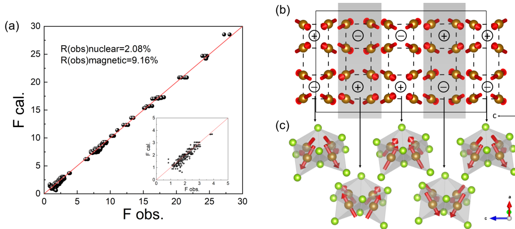
Figure 5.9: (a) Result of the refinement for the C_{4m} magnetic structure. Structure factors of nuclear and magnetic Bragg reflections collected at 10 K are plotted against the calculated values. The inset shows the range of low F values, which mainly represents the magnetic reflections. (b) Projections of the Fe atoms on the b_d c_d -plane with the tilting spins in Block-A magnetic order. The yellow balls indicate the Fe atoms. The red arrows are the spins of Fe. The + and - indicate the net moments of the blocks. The Fe ladders-A (B) are represented by white (grey) backgrounds. (c) The \text{FeSe}_4 tetrahedra of the blocks in (b) (indicated by the black arrows).
