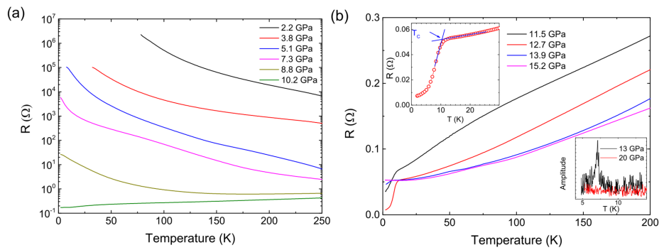
Figure 2.14: The temperature dependence of the resistance of \text{BaFe}_2\text{Se}_3 at various pressures. [1]
