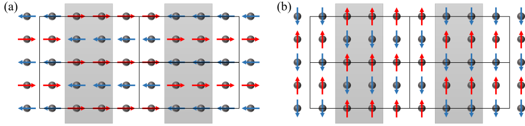
Figure 2.17: (a) Magnetic structure of \text{BaFe}_2\text{Se}_3 . (b) Magnetic structure of \text{CsFe}_2\text{Se}_3 , \text{KFe}_2\text{Se}_3 , and \text{RbFe}_2\text{Se}_3 .
