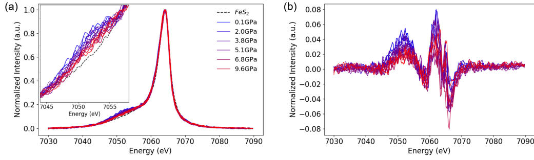
Figure 5.16: (a) Normalized Fe K_\beta X-ray emission spectroscopy of \text{BaFe}_2\text{Se}_3 at different pressures, together with \text{FeS}_2 zero-spin reference from reference [209]. The inset is a zoom around 7050 eV at which the spectra changed. (b) Difference between the XES spectra of \text{BaFe}_2\text{Se}_3 and \text{FeS}_2 in (a).
