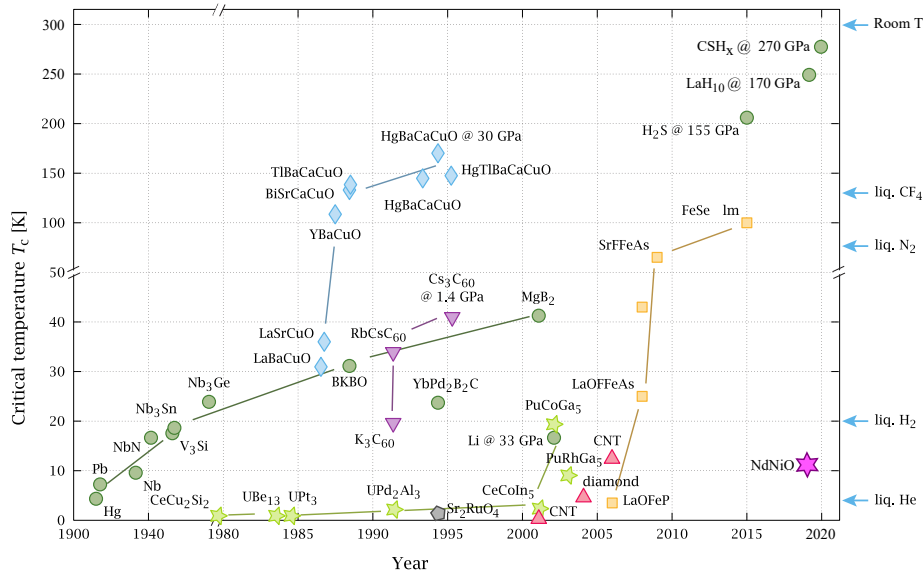
Figure 1.10: History of some discovered superconducting compounds [91]. Note in particular the BCS superconductors (green circles), the cuprates (blue diamonds), and the iron-based superconductors (yellow squares).
