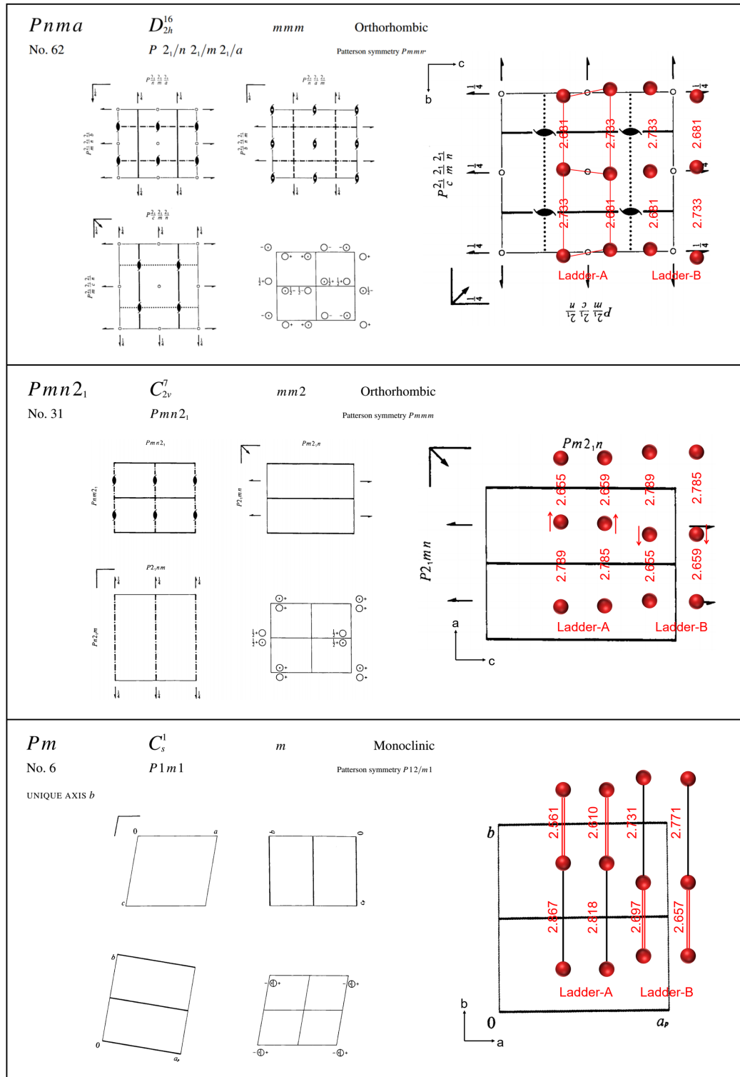
Figure 4.6: Diagrams for the symmetry elements and the general position of Pnma (top), Pmn2 1 (middle), and Pm (bottom) [173]. The two ladders in one unit cell are shown with the corresponding diagram for the three space groups. The Pnma structure is extracted from reference [4] while Pmn2 1 and Pm are based on our results. In Pnma , the two Fe-blocks (indicated by the solid red lines) of the ladder have the same Fe-Fe distances due to the inversion centers. In Pmn2 1 , the absence of inversion centers allows a Fe displacement towards one direction (indicated by the red arrows). Therefore, a large difference in Fe-Fe distance between the two Fe-blocks along the chain is induced. In Pm , since the 2 1 screw axis is absent, eight different Fe-Fe distances are observed. The red double-lines indicate the short Fe-Fe bonds while the black lines indicate the long ones.
