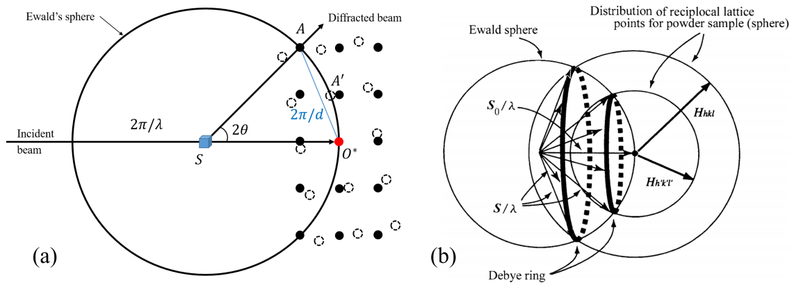
Figure 3.10: (a) Visualization of the diffraction condition in a crystal using the Ewald's sphere with radius 2\pi/\lambda and the reciprocal lattice projection in a plane of the reciprocal lattice. The lattice after rotation around O^* is shown as the dash circles. A and A' are the lattice dots on the Ewald's sphere. (b) Illustration of powder diffraction using the Ewald's sphere [172].
