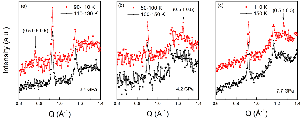
Figure 5.14: The patterns collected below and above the Néel temperatures at 2.4(a), 4.2(b), and 7.7(c) GPa.
