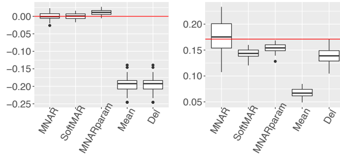
Figure 3.4: Mean (left) and variance (right) estimations of Y_{1,1} when data are generated under the fixed effects model.
