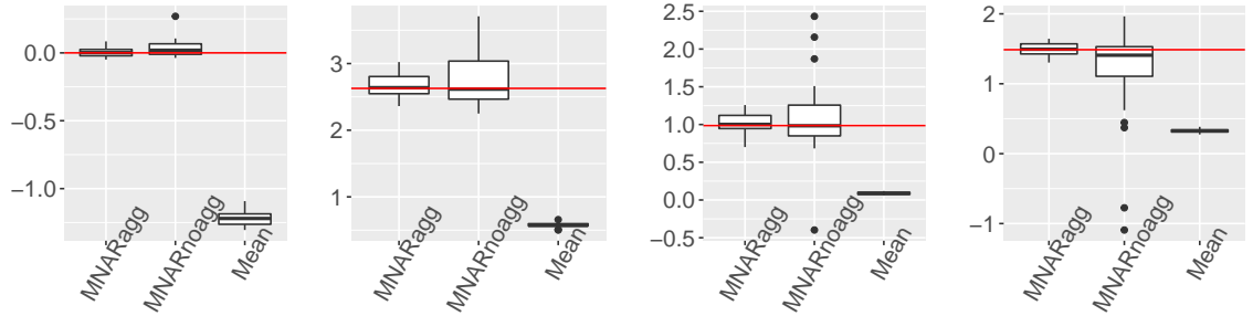
Figure C.13: Mean (left) and variance (middle left) estimations of Y_{.1} and covariances estimations of \text{Cov}(Y_{.1}, Y_{.2}) (between two missing variables) (middle right) and of \text{Cov}(Y_{.1}, Y_{.8}) (between one missing variable and one pivot variable) (right). True values are indicated in red lines.
