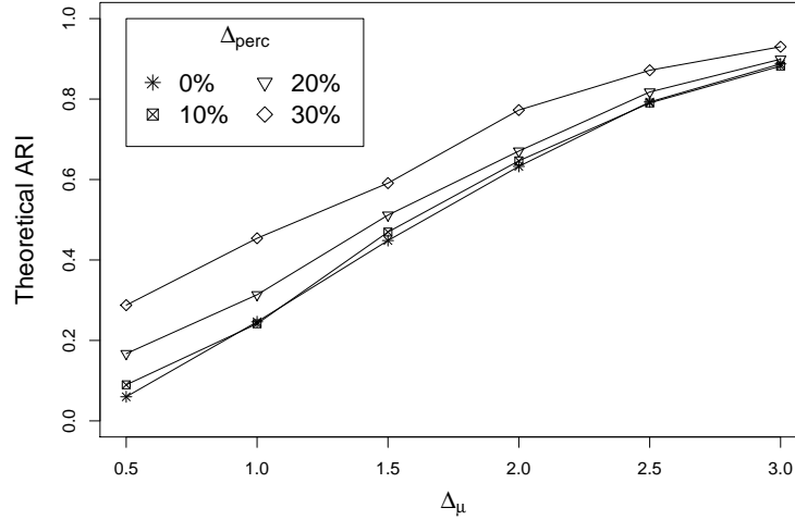
Figure 5.3: Relative effect of both the mixture component separation strength \Delta_\mu and the MNAR evidence \Delta_{\text{perc}} on theoretical ARI. For example, if \Delta_{\text{perc}} = 10\% , it means that the second class has 10% more missing values than the first class.
