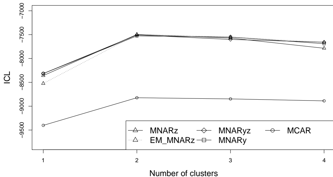
Figure 5.7: Comparison of the different algorithms in terms of ICL for bivariate Gaussian data ( n = 2000 , d = 2 ) and two classes when the true missing-data mechanism is \text{MNAR}_z and \Delta_\mu = (4, 4) . The algorithms have been performed for K = 1, 2, 3, 4 . The dots are the means for the process of drawing 10 times the triplet (Y, Z, C) .
