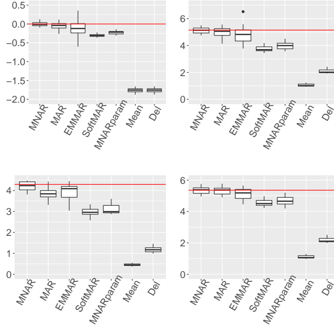
Figure 3.3: Mean (top left) and variance (top right) estimations of the missing variable and covariances (bottom) estimations of \text{Cov}(Y_{1,1}, Y_{2,2}) ( i.e. covariance between two missing variables) and of \text{Cov}(Y_{1,1}, Y_{8,8}) ( i.e. between one missing variable and one pivot variable). True values are indicated by red lines.
