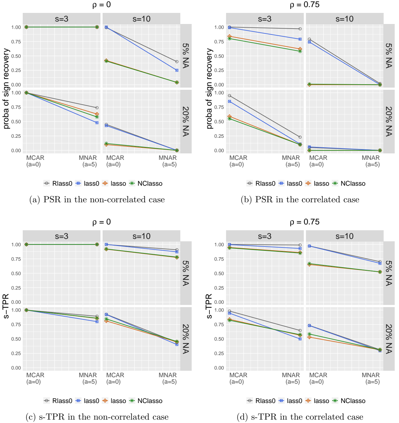
Figure A.1: PSR and s-TPR with an s -oracle tuning, for sparsity levels , s = 3 and s = 10 (subplots columns), proportions of missing values 5% or 20% (subplots rows), and two missing data mechanisms (MCAR vs MNAR).
