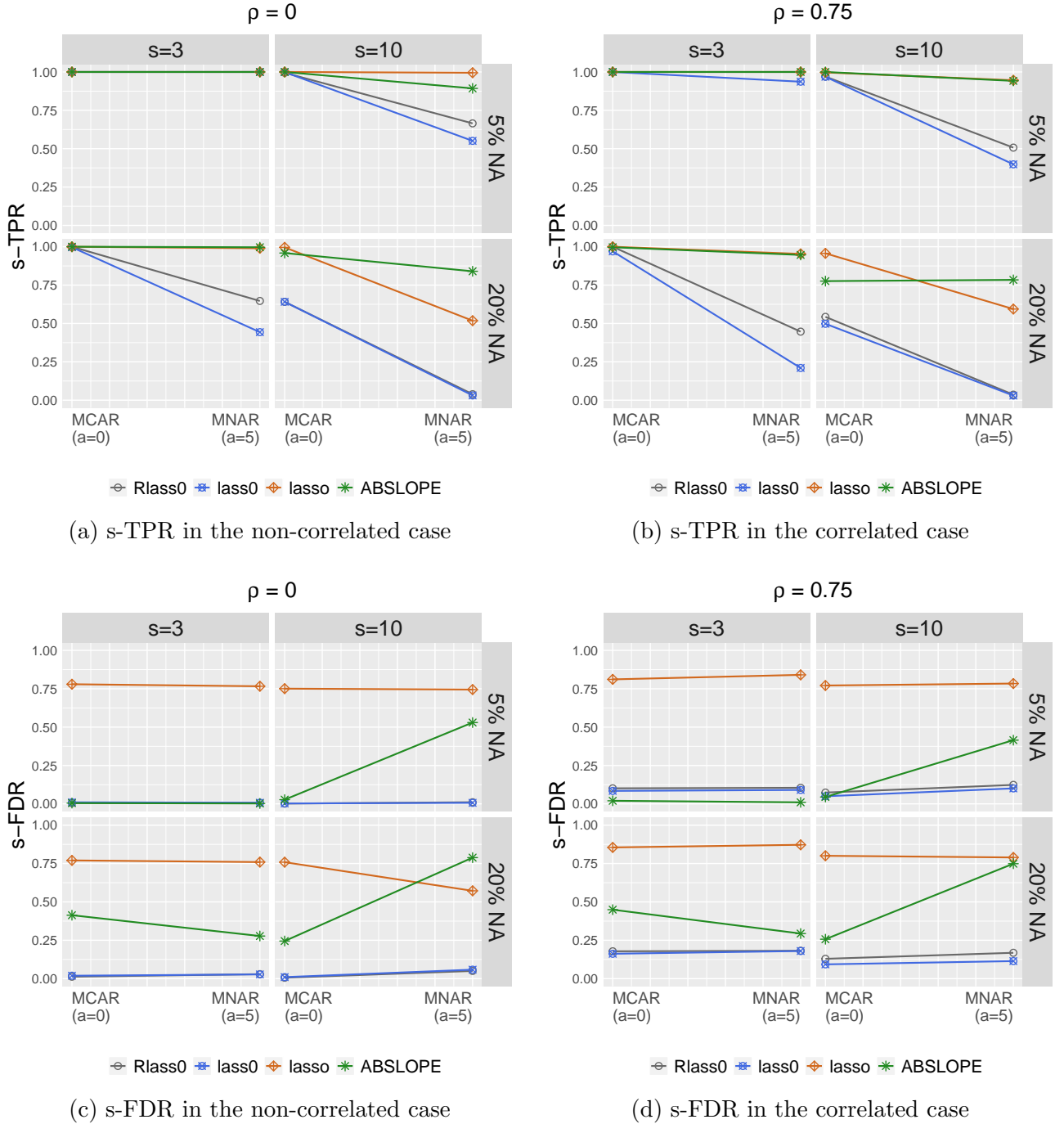
Figure A.3: s-FDR and s-TPR with automatic tuning, for sparsity levels s = 3 and s = 10 (subplots columns), proportions of missing values 5% or 20% (subplots rows), and two missing data mechanisms (MCAR vs MNAR).
