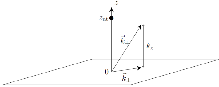
Figure 5: Representation of an atom at height z above a plane surface. The wavevector \vec{k} is decomposed along its transverse \vec{k}_\perp and longitudinal k_z components.
