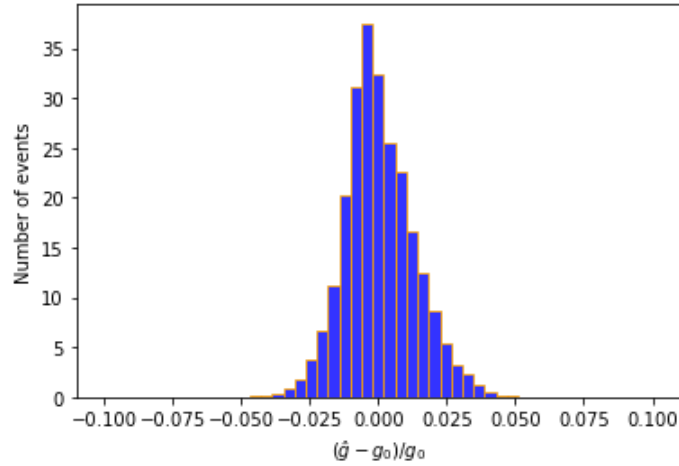
Figure I.21: Histogram of estimators \hat{g} for 10000 random draws in the case of the cylindrical chamber.
