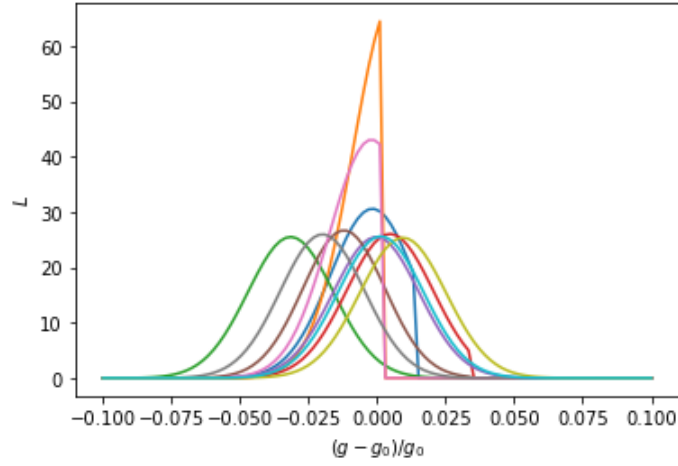
Figure I.20: Sample of 10 normalized likelihoods calculated in the case of the cylindrical chamber for independent random draws of 1000 atoms.
