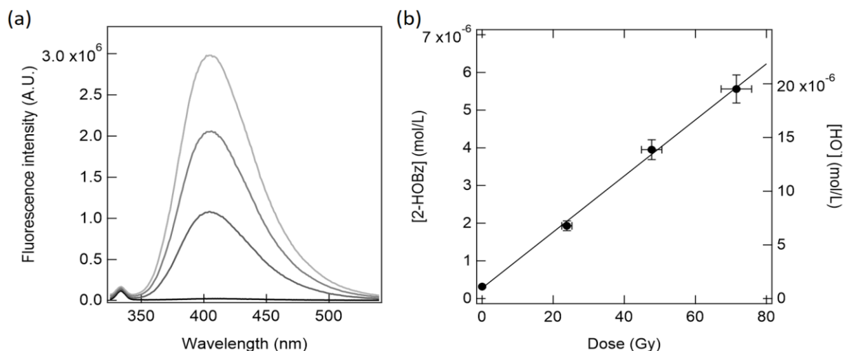
Figure II-17: Determination of the hydroxyl radical yield for gamma irradiation. Presented data were obtained on NaBz 10 mM aerated solutions: (a) Fluorescence signal curves obtained for increasing time of exposure, (b) Deduced hydroxyl radical concentration as a function of the dose. The hydroxyl concentration was deduced from calibration curves obtained with the same fluorimeter with the same solution varying the concentration of Na 2-HOBz.
