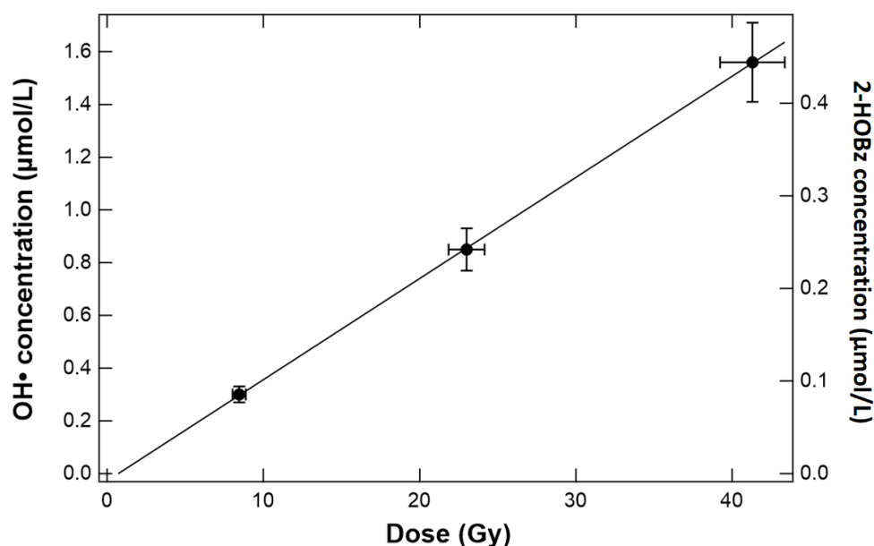
Figure IV-3: Concentration of HO\cdot radicals formed in aerated 0.01 mol/L NaBz solutions irradiated with 1.28 keV X-rays as a function of dose. Data were fitted by using a linear regression.
