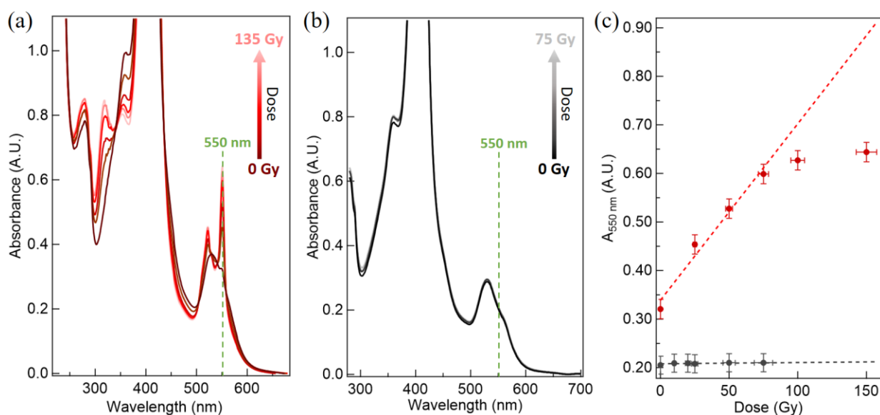
Figure IV-16: UV-Analysis of gamma irradiated solution of ferricytochrome c (45 \mu M in 20 mM phosphate buffer, pH =7.2) in aerated condition. Absorption spectra (a) without SOD (b) in presence of SOD (5 \mu M), (c) Optical density (OD) at 550 nm as function of the dose and fitted by a linear regression ( y=a +bx ). Fitting parameters were found to be a=0.339\pm 0.006 and b=0.0036\pm 0.0004 (OD/Gy). Vertical error bars indicate the standard error of the mean.
