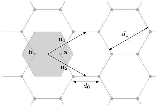
(a) \mathcal{L} = \mathbf{u}_1\mathbb{Z} + \mathbf{u}_2\mathbb{Z} is the triangular lattice, N = |\mathbf{R}| = 2 and m = 1 . The honeycomb lattice is the superposition of two sifted versions of \mathcal{L} : \mathcal{L}^H = (\mathcal{L} + \mathbf{a}) \cup (\mathcal{L} + \mathbf{b}) . The Wigner-Seitz cell \Gamma is colored in gray. Vertices linked by gray lines are nearest neighbors. The nearest neighbor distance d_0 and the second nearest neighbor distance d_1 > d_0 are displayed.
