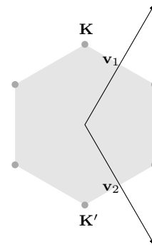
(b) The vectors \mathbf{v}_1 and \mathbf{v}_2 generate the reciprocal lattice \mathcal{L}^* . The first Brillouin zone \Gamma^* is colored in gray. The vertices \mathbf{K} and \mathbf{K}' of \Gamma^* are shown, the others are obtained by rotation by 2\pi/3 and 4\pi/3 about the origin.
