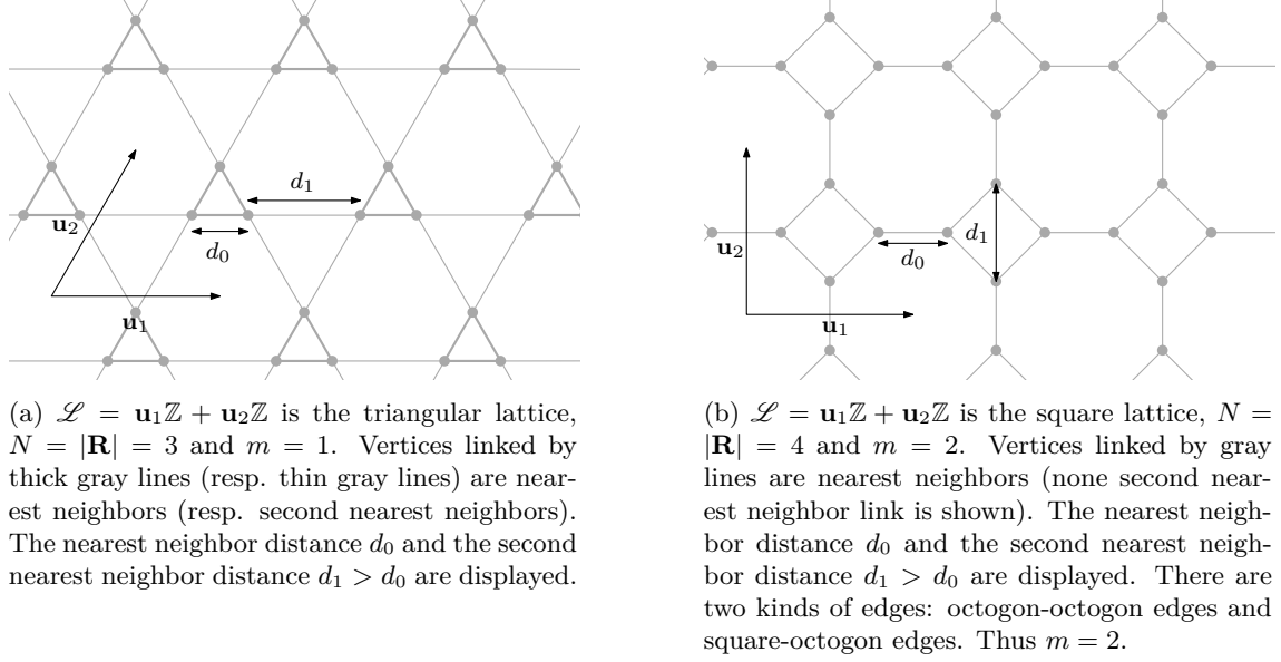
Figure 3.1 – Examples of lattices \mathcal{L}^{\mathbf{R}} with different parameters.
