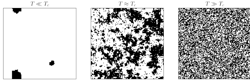
Figure 6: The figure shows the final configuration of a 2D Ising model with first neighbours interaction for different temperatures. From the left to the right. When T \ll T_c the system displays a global magnetisation (the spins are aligned), at the critical temperature, T \approx T_c , clusters of different sizes of aligned spins coexist. Finally, when T \gg T_c the entropic effects are dominant and the global magnetisation is zero. Simulations are performed using a Monte Carlo algorithm. The size of the lattice is 128 \times 128 spins.
