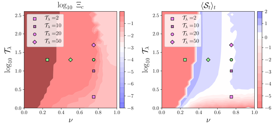
Figure 31: The left and right heat-map shows \log_{10} \Xi_c (resp. average Sharpe ratio) as a function of the memory timescale \mathcal{T}_\lambda and the weight parameter \nu . The dark red zones correspond to the regions where \Xi_c > 0.99 , where crises are permanent.
