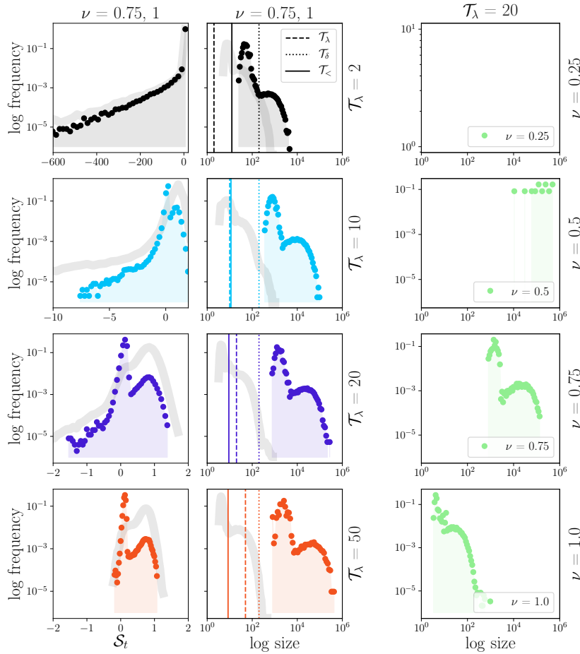
Figure 33: The two left columns show the histograms of Sharpe ratio \mathcal{S} and crisis duration \mathcal{T}_< for four values of \mathcal{T}_\lambda : 2, 10, 20 and 50, all for the same value of \nu (shown as symbols in the two heat-maps on the left). The faded grey lines show the same histograms in the benchmark case \nu = 1 that correspond to the \mathcal{H}_k\mathcal{H}_c point in Fig. 28. Other parameters used are: \delta = 0.005 , c_0 = 0.017 , \sigma_z = 0.15 and \alpha = 15 .
